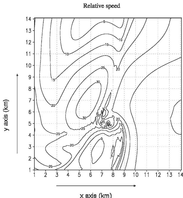
FIG. 14. Vortex-relative speed at 3600 s on grid 2. Vortex translational velocity is 19 and -6 \text{ m s}^{-1} and was found by removing the first-order modes from the velocity pattern of the vortex.
