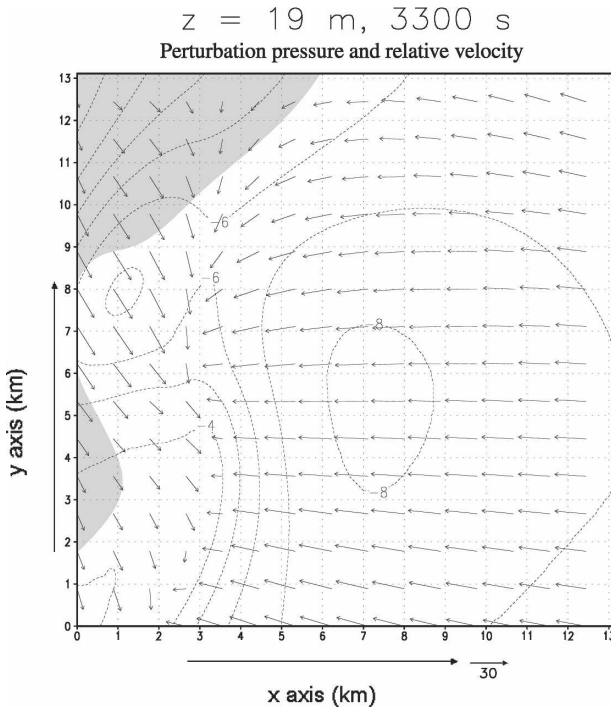
FIG. 3. Perturbation pressure and vortex-relative velocity vectors for grid 2 at 3300 and 19 m above the surface. Contours of perturbation pressure have an increment of 0.5 mb. Magnitude of reference vector has units of \text{m s}^{-1} .
