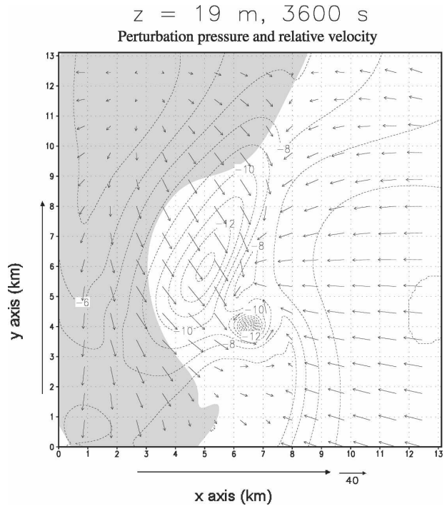
FIG. 4. Same as in Fig. 3, but at 3600 s. Minimum perturbation pressure in vortex is -19 \text{ mb} .
