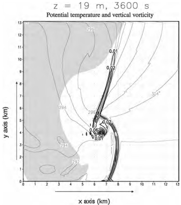
FIG. 2. Same as in Fig. 2, but at 3600 s.
