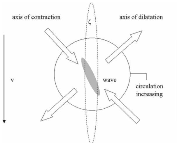
FIG. 9. Depiction of the increase of circulation caused by a rotated vorticity segment (shaded) with respect to an unbounded one-dimensional vorticity band (dashed). Block arrows denote the deformation field associated with the vorticity band; solid arrows the velocity field. The circular region denotes a sample region where circulation is increasing.
