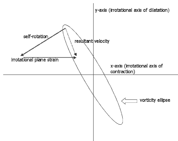
FIG. 6. Schematic showing elliptical vorticity patch in large-scale irrotational straining field. Bold solid arrows denote contributions to resultant velocity in vorticity patch (dashed arrow). Based on schematic from Neu (1984a).
