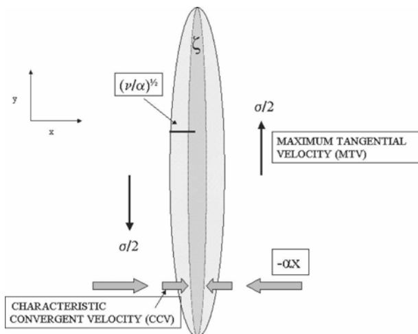
FIG. 10. Schematic showing definitions of MTV and CCV, as described in text.
