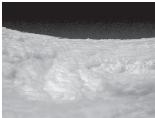
FIG. 7. Digital photograph of the eyewall of Hurricane Isabel taken 12 Sep 2003 from the NOAA WP-3D aircraft while inside the eye. The curved, finger-like feature is seen in the middle of the photograph.
