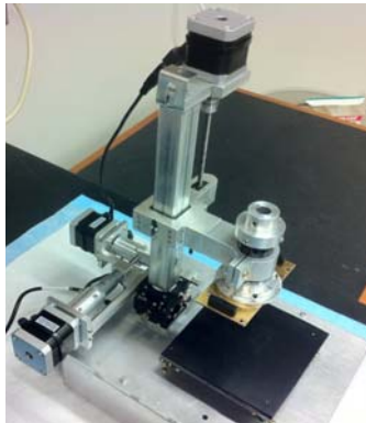
Figure 1.2: Image of the translation stage that automates raster-scanning and pressure-sensing.
