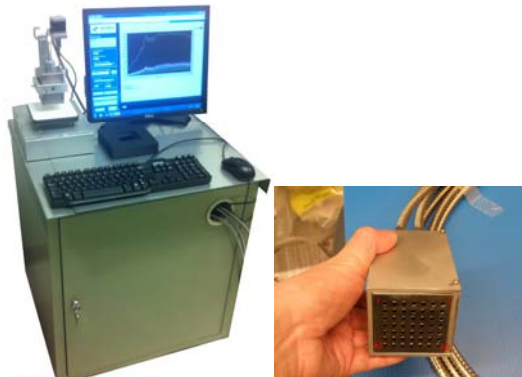
Figure 1.1: Image of 49-Channel System and probe with 49 channels.
