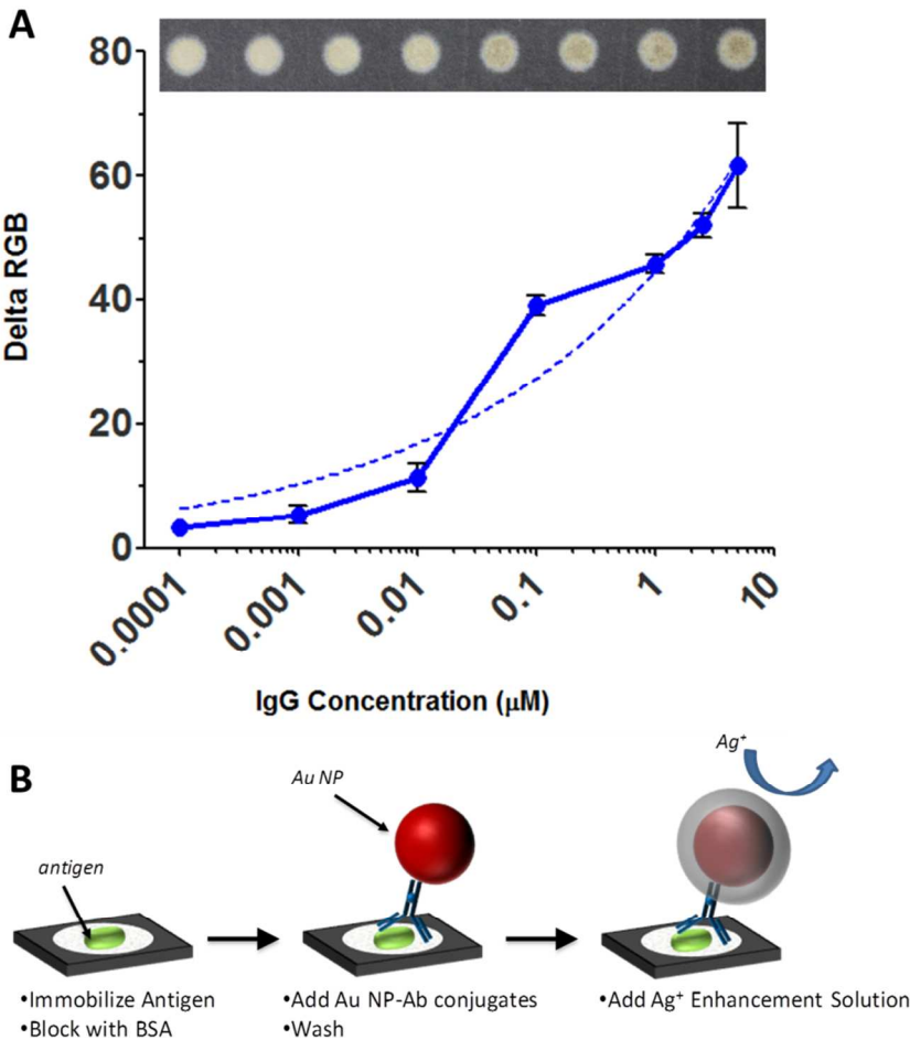
Figure 4. Enzyme-free P-ELISA of Rabbit IgG in DI H 2 O using IgG antibody conjugated Au NPs with silver enhancement stain. (A) Plot of delta RGB vs. IgG concentration using Au NP – silver enhancement procedure. Error bars indicate SEM with n=4. (B) Schematic of Enzyme-free P-ELISA Assay.
