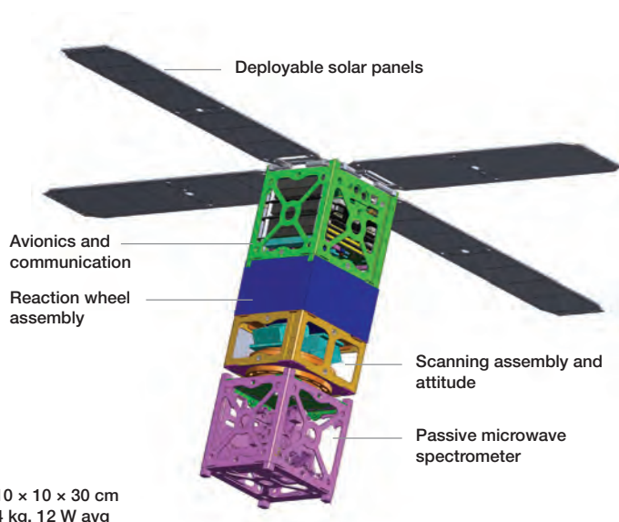
This rendering shows an MIT and Lincoln Laboratory computer-aided design of a passive microwave sounder concept packaged in a nanosatellite (CUBESAT) form factor.
