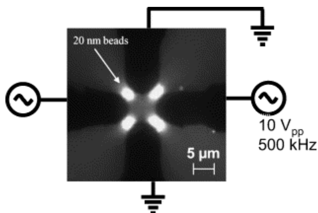
Figure 3.9: 20 nm latex beads shown attracted to high electric field regions between the electrodes.
