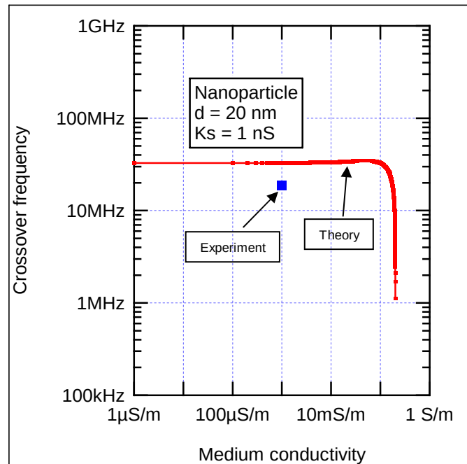
Figure 3.12: Predicted dependence of DEP crossover frequency on suspension conductivity.
