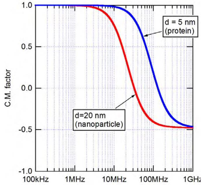
Figure 3.11: Frequency dependence of the Clausius-Mossotti factor, assuming a surface conductance of K_s = 1 \text{ nS} .
