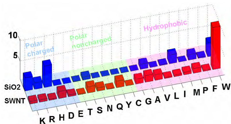
Figure 5.4. Relative occurrence of amino acids in nanotube and control experiments. The red and blue bars are for SWNT samples and their controls, respectively.
