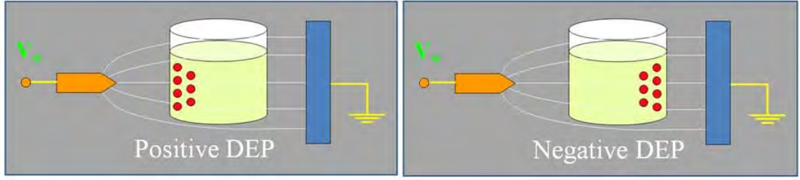
Figure 2.2 Positive and negative DEP
