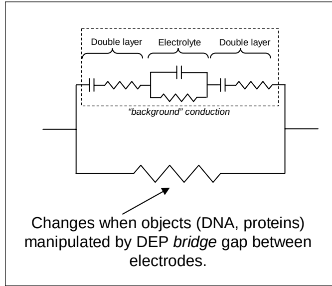
Figure 3.4: Effective circuit model for objects trapped using DEP between electrodes.
