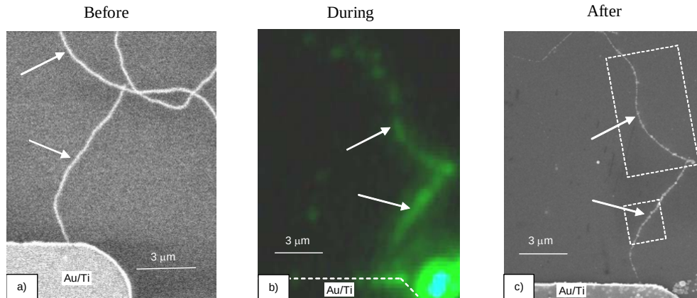
Figure 4.7: Key result of this work. A) SEM image of the nanotubes and gold electrodes before the DEP experiments. B) Fluorescence microscopy images taken during the DEP experiment. (The solution was still on the sample.) C) SEM image of the nanoparticles attached to the nanotubes after the DEP experiments.
