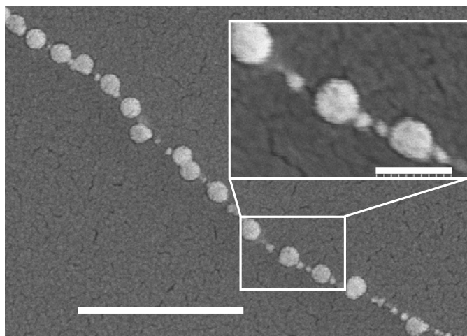
Figure 4.8: Another zoom of fig. 7. Both the 20 nm and 100 nm particles are clearly visible along the length of the nanotube. Scale bar: 1 \mu\text{m} ; inset: 200 nm.
