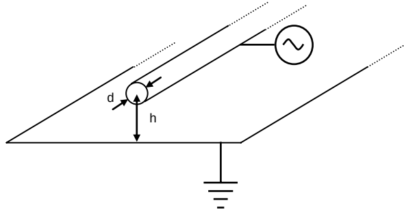
Figure 4.4: Model geometry for cylinder above a ground plane. In practice there is a dielectric (oxide) between the nanotube and the conducting Si substrate.
