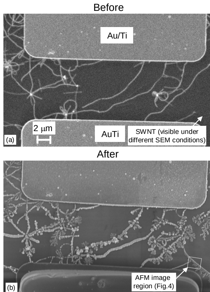
Figure 4.11: SEM images of SWNTs before and after DEP experiments.
