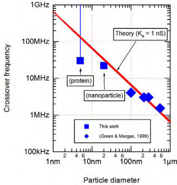
Figure 3.13: Crossover frequency vs. particle diameter in the low suspension conductivity limit. The measurement for the protein crossover frequency corresponds to a lower limit only, limited by the electronics used, thus the bar.
