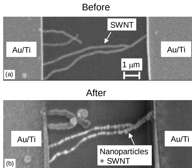
Figure 4.10. SEM image of nanotube contacted electrically on both ends before and after DEP experiments using 2 nm gold nanoparticles. The Au nanoparticles are attached to the nanotubes after the DEP experiments.
