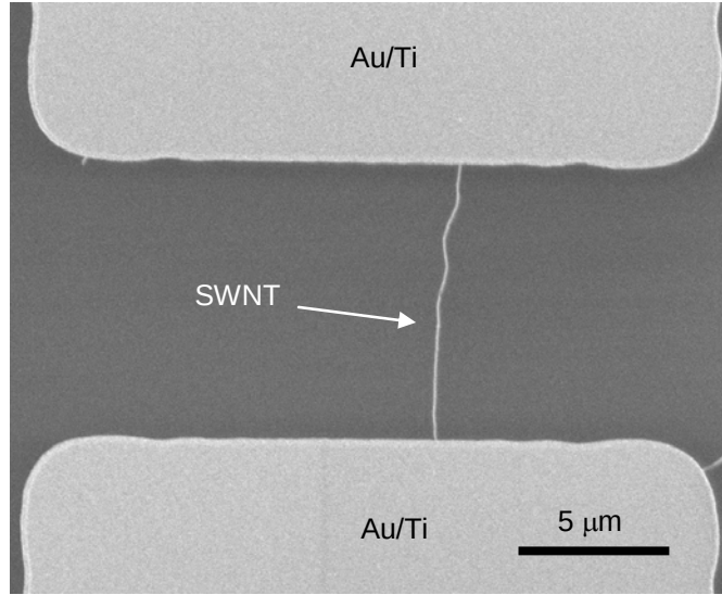
Figure 4.2: SEM image of typical nanotube contacted electrically with Au/Ti bi-layer, before the DEP experiments.
