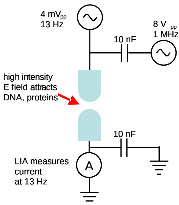
Figure 3.2: Circuit for conductance measurements.
