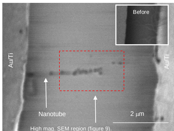
Figure 4.5 SEM images of nanotube contacted electrically on both ends, before and after the trapping experiments using 100 nm polystyrene nanoparticles. The alignment along the tubes is clear.
