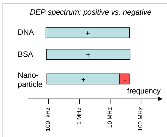
Figure 3.10: DEP spectrum, showing frequency regions where positive (+) and negative (-) DEP were observed. 30 MHz was the upper frequency limit for our electronics.
