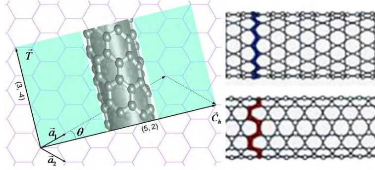
Figure 1.1. A graphite rolled up into a (5,2) nanotube. Depending on the roll-up vector, a carbon nanotube can be zigzag, armchair or chiral.
