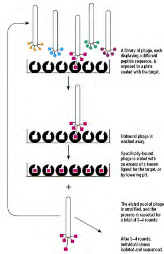
Figure 2.4 Panning with Ph.D peptide display. Image from reference 3.
