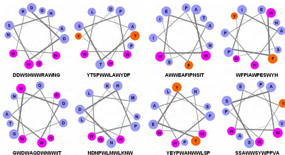
Figure 5.7: Helical wheel presentations of the peptides found which bind to SWNTs.
