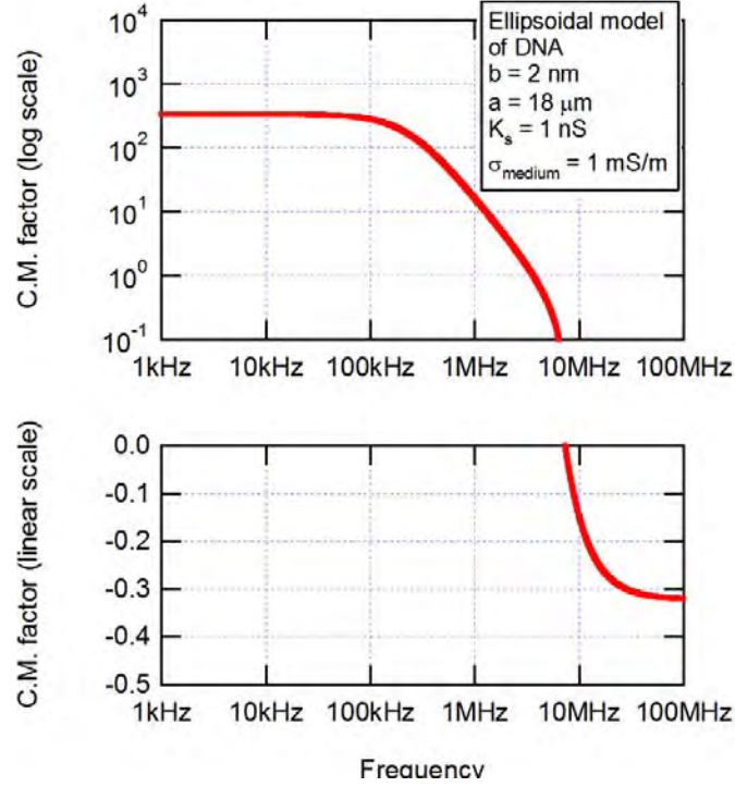
Figure 3.14: Calculated effective C.M. factor for DNA, assuming an ellipsoidal model
