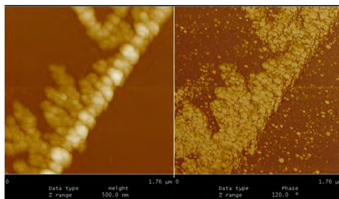
Figure 4.12: A) Tapping mode and b) phase contrast mode AFM images of a Au nanoparticles on a nanotube.
