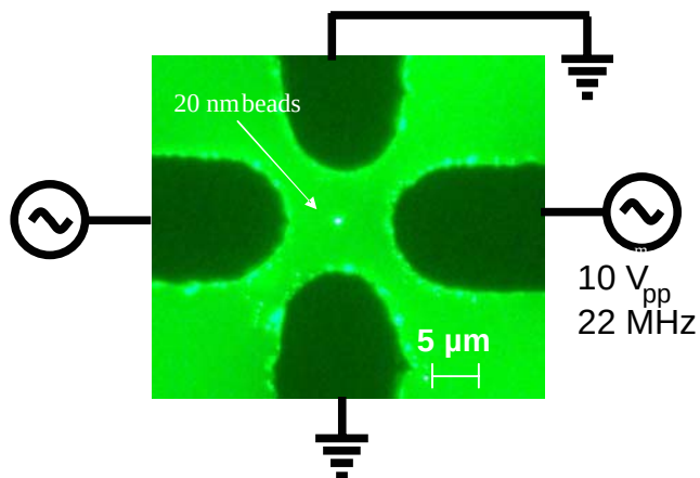
Figure 3.8: 20 nm latex beads shown trapped in the center of the electrodes due to negative DEP.
