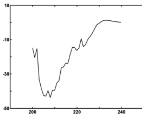
Figure 5.3. CD measurements of peptide P1.
