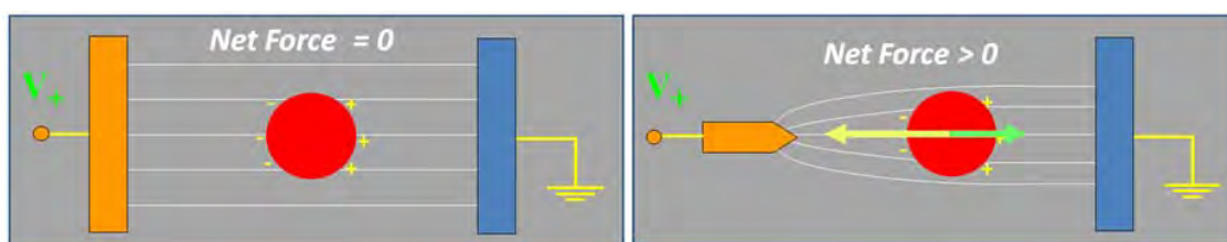
Figure 2.1 Particles in the uniform and non-uniform fields
