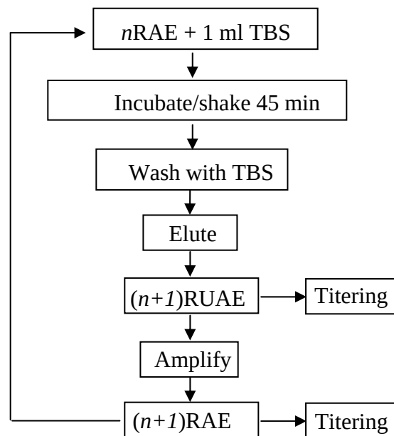
Figure A-2.1. The schematic process for phage display experiments. RT stands for Room Temperature; n\text{R(U)AE} for the n th-Round of (Un)Amplified Elution. 10 \mu\text{l} NEB phage is used for 0\text{RAE} .
