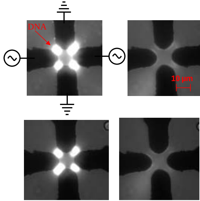
Figure 3.5: Images of fluorescently labeled DNA. The four images were taken in on/off/on/off sequence in a time span of about 30 seconds. The applied voltage was 1 MHz, 8 V_{pp} .
