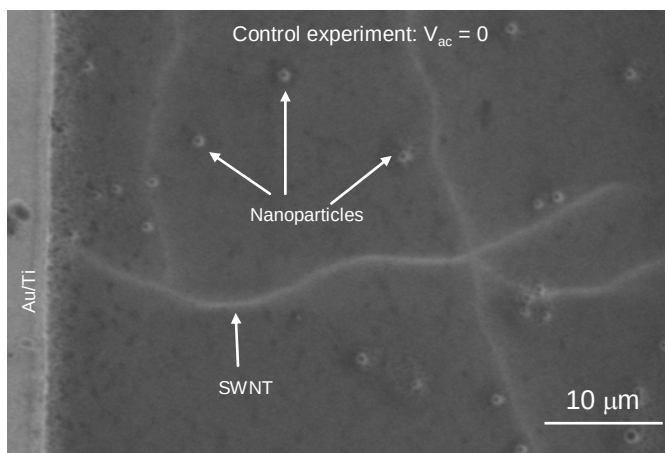
Figure 4.9: Control experiment in which no ac voltage was applied shows that nanoparticles do not attach to nanotubes.
