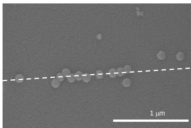
Figure 4.6: High magnification image of region outlined in Figure 4.5, after Au has been sputtered to enhance resolution and contrast of the 100 nm nanoparticles. The dashed white line shows where the nanotube is, which is not visible because it is covered by 10 nm of sputtered Au.
