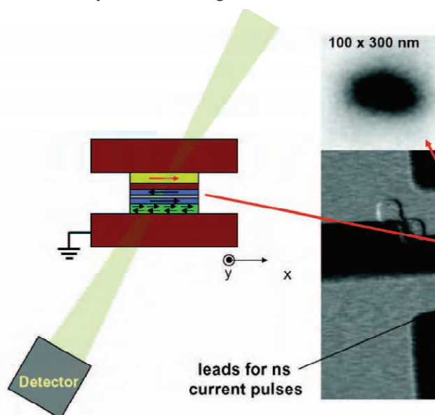
Figure 3.9. Scanning transmission x-ray microscopy reveals the structure and local magnetic properties of a 100 × 300 nm GMR device under a gold capping layer. (Courtesy Joachim Stöhr, Stanford Linear Accelerator Center.)
