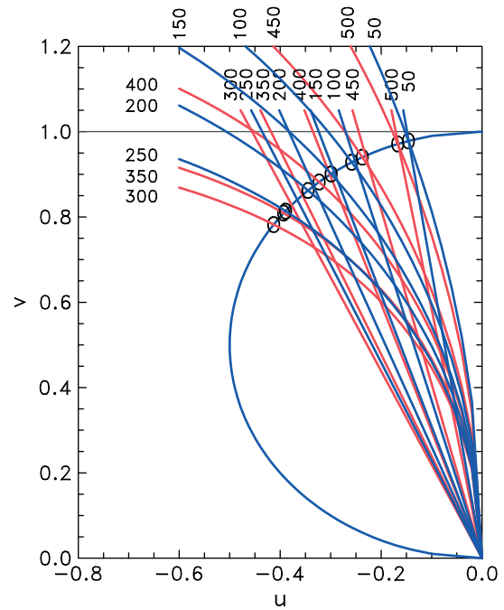
Figure 1. The circle corresponding with Equation (24) and the curves given by Equation (26) for typical values of the parameters \sigma and \nu . These parameters are derived from the radial profile of v_g used to construct Figure 2. The straight lines are those given by Equation (27) for the same parameters. The numbers marking the curves are the radii (km) at which the parameters \sigma and \nu are calculated. The darker (blue) curves correspond to radii \leq 250 km and the lighter (red) curves for radii \geq 300 km. This figure is available in colour online at www.interscience.wiley.com/journal/qj
