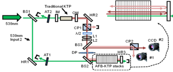
Fig. 3. Experimental setup for the image recovery.
