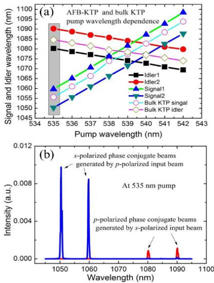
Fig. 3. (Color online) (a) Measured signal and idler wavelengths of AFB-KTP and bulk KTP as a function of pump wavelength; (b) Phase conjugated beam spectra generated by p -polarized input beam (blue peaks) and s -polarized input beam (red peaks).
