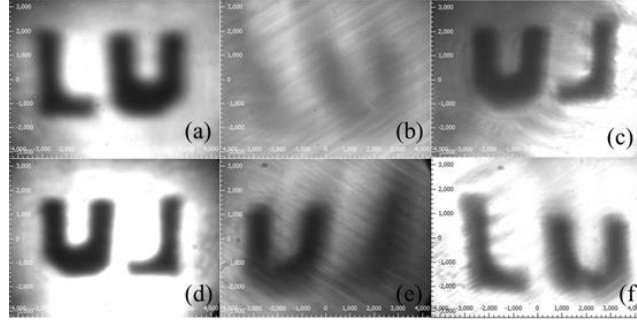
Fig. 2. P -polarized (a) and s -polarized (d) input beam without distortion images, after distortion images (b) and (e); restored images (c) and (f) by phase-conjugated beams at pump wavelength of 539 nm.
