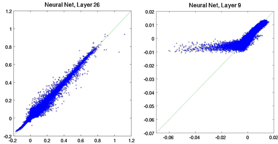
Fig. 1. Layer bias. Scatterplots of the neural network approximation for the layers l = 26 and l = 9 . In each diagram the values of the original parameterization y_l are plotted along the horizontal axis, the approximated values \tilde{y}_l along the vertical axis. The green line shows the diagonal y_l = \tilde{y}_l .
