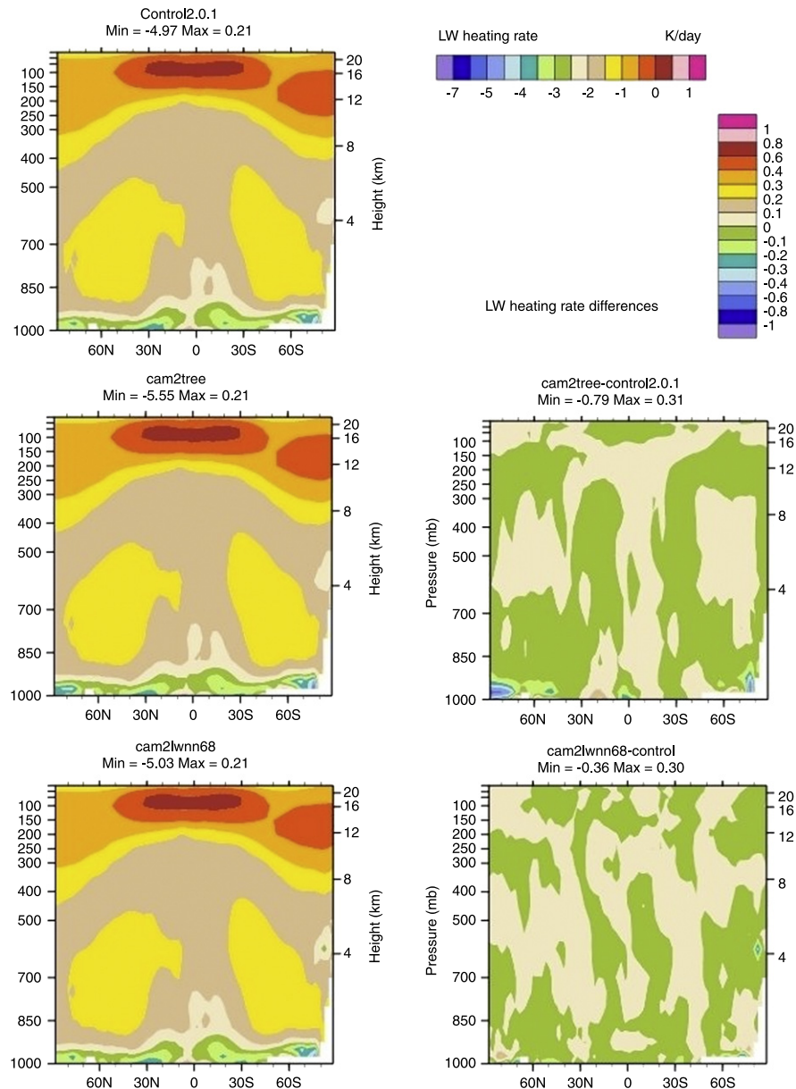
Fig. 5. Comparison of the predicted annual zonal means of the LWR heating rates computed with the original parameterization (top row), a tree based emulation (center row) and a neural network emulation (bottom row). The right column plots the difference between the simulation and the control.
