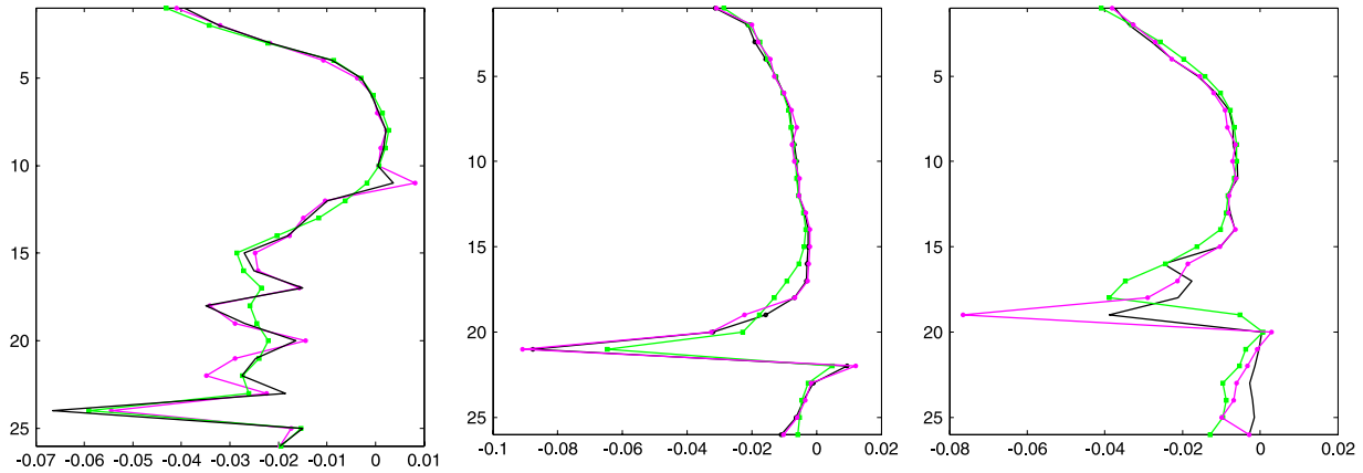
Fig. 4. Approximation of three representative heating rate profiles. Black line without markers: original parameterization. Magenta with circle markers: Component-wise emulation. Green with square markers: vector-valued Random-Forest emulation. Heating rates units are J/kg/s. (For interpretation of the references to colour in this figure legend, the reader is referred to the web version of this article.)
