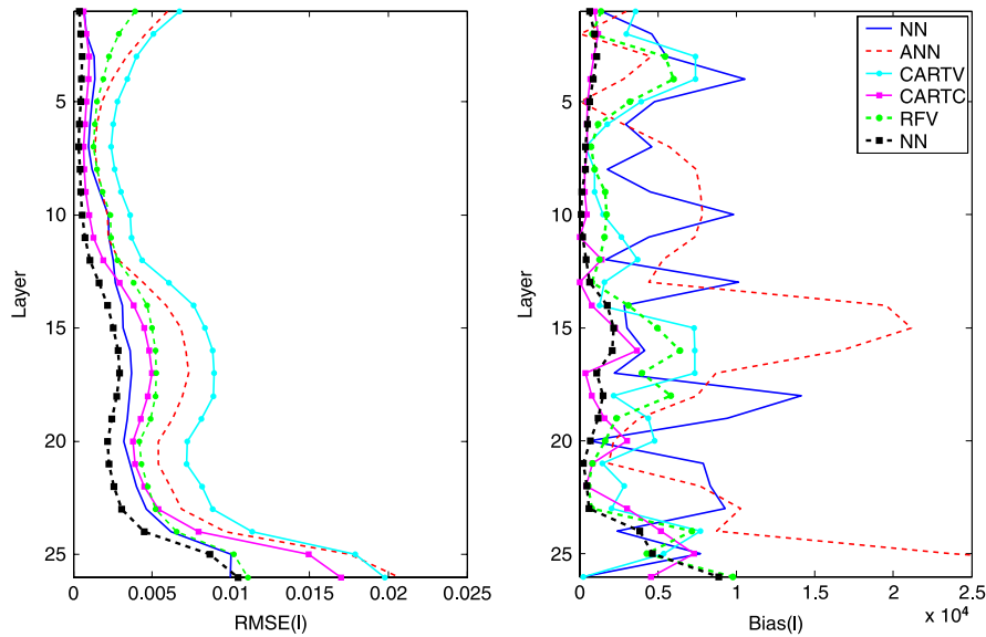
Fig. 2. Comparison of neural network, approximate nearest neighbor, and several regression tree emulations. Left: layer-wise root mean square errors. Right: layer-wise absolute values of bias.
