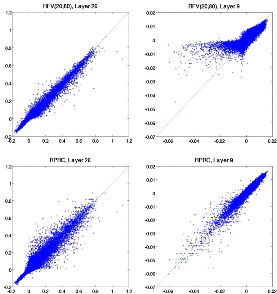
Fig. 3. Scatterplots for the approximation of the heating rates in the 26th and 9th vertical layer with componentwise CART (RPRC) and the vector-valued Random Forest (RFV) approximation.
