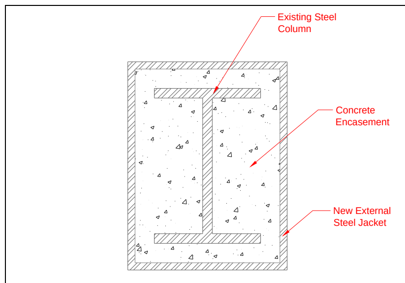
Figure 16. Steel column with concrete-filled steel jacket.
