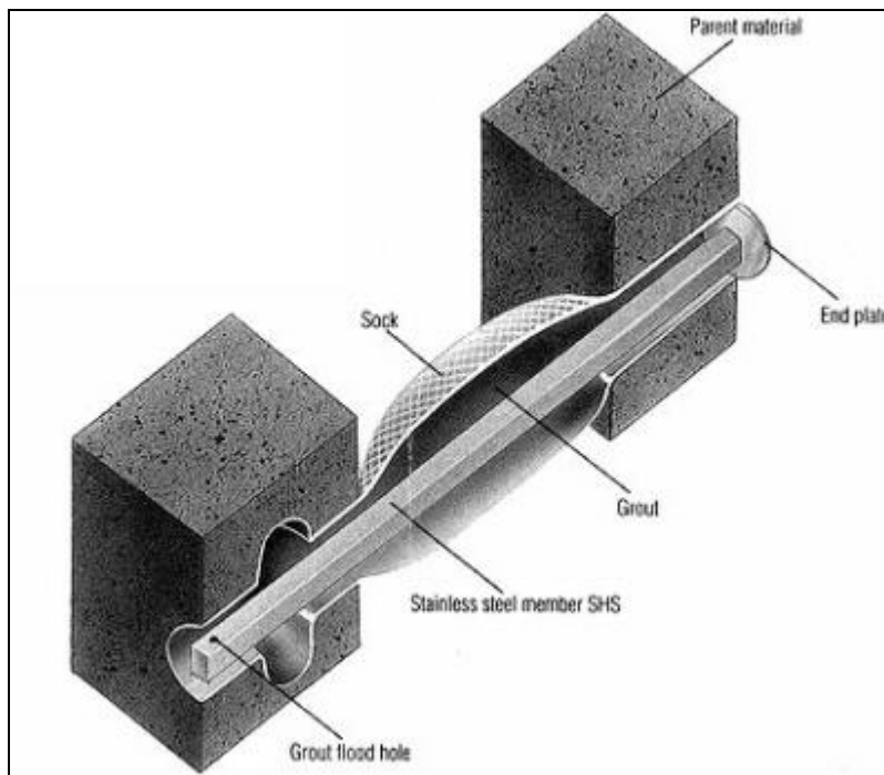
Figure 31. Retrofitted Reinforcement by means of coring (Sanicki 1998).
