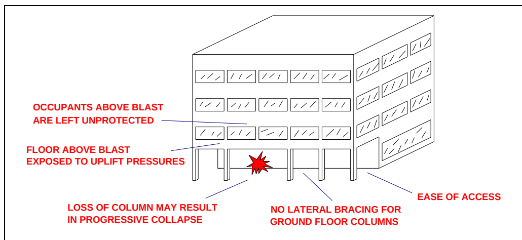
Figure 29. AT issues related to building overhangs.
