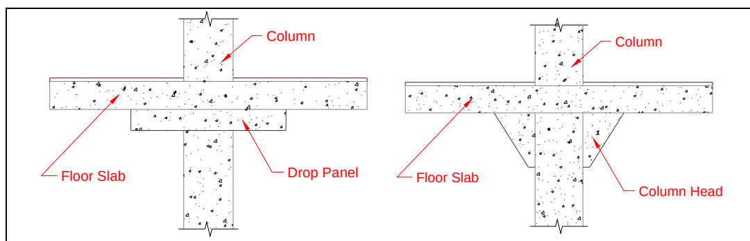
Figure 23. Details of drop panel and column head connection enhancements.
