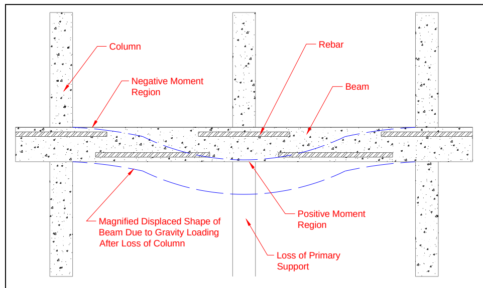
Figure 27. Reinforced concrete beam response to column loss.
