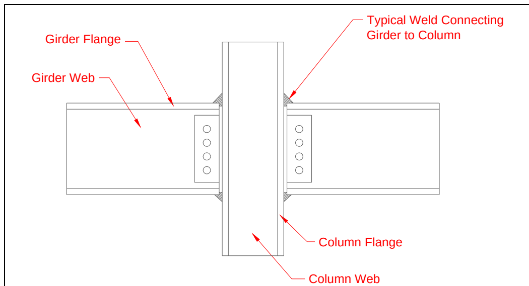
Figure 13. Conventional welded structural steel frame beam/column connection.
