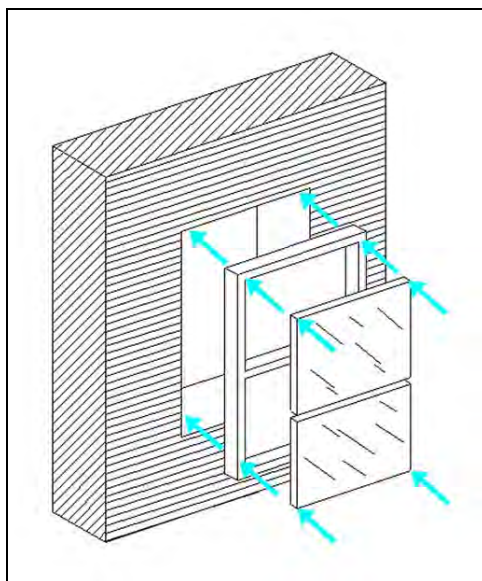
Figure 40. Blast load path through a window system.
