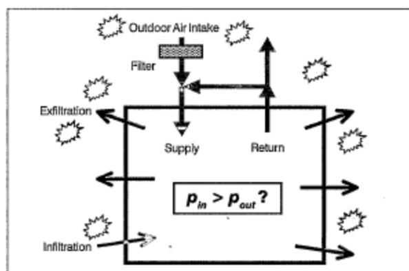
Figure 53. Pressurization/filtration protection (Persily 2004).
