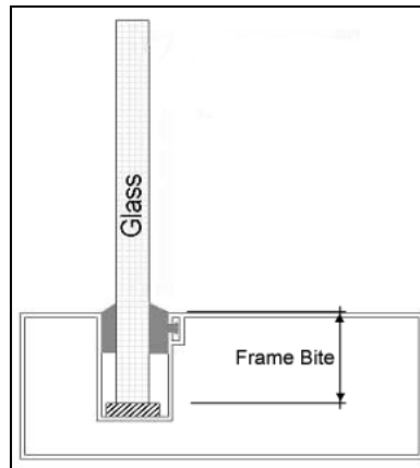
Figure 42. Diagram showing frame bite.
