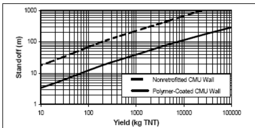
Figure 33. Comparison of standoff required for CMU walls with and without sprayed polymer coating (ETL 02-4).
