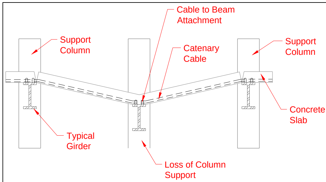
Figure 28. Conceptual diagram of cable support system for structural redundancy.
