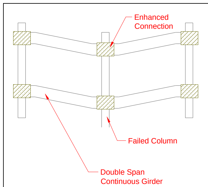
Figure 21. Conceptual diagram of catenary action.
