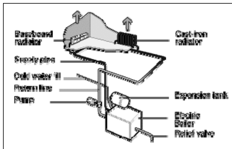
Figure 49. Radiator loop system (Hayden 1996).
