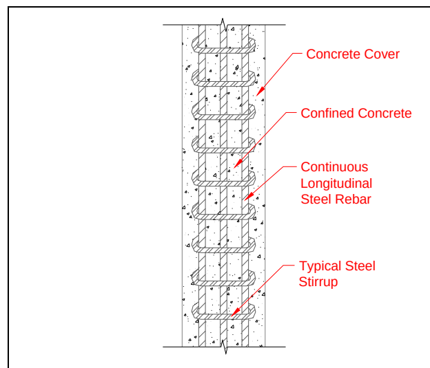
Figure 14. Components of a reinforced concrete column.
