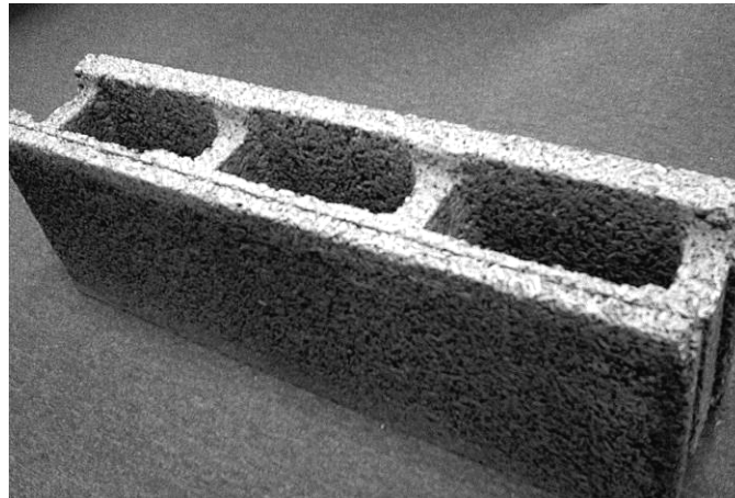
Figure 32. Individual Durisol® block showing cavities for concrete and steel reinforcement (ERDC-CERL 2005).
