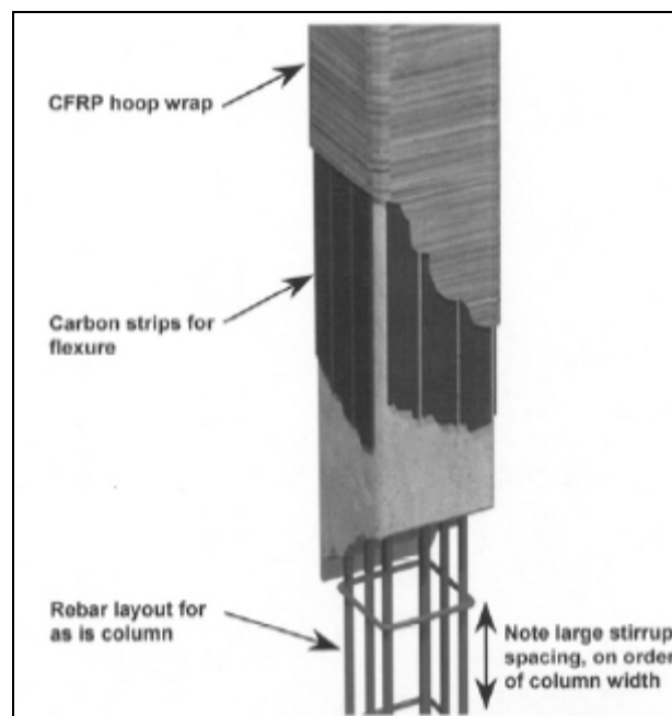
Figure 19. CFRP flexure strips applied under CFRP hoop wrap (Crawford, Malvar, and Morrill 2001).
