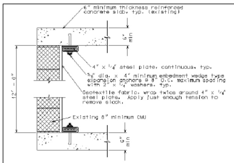
Figure 36. Cross section of geotextile fabric installation (ETL-1110-3-494).
