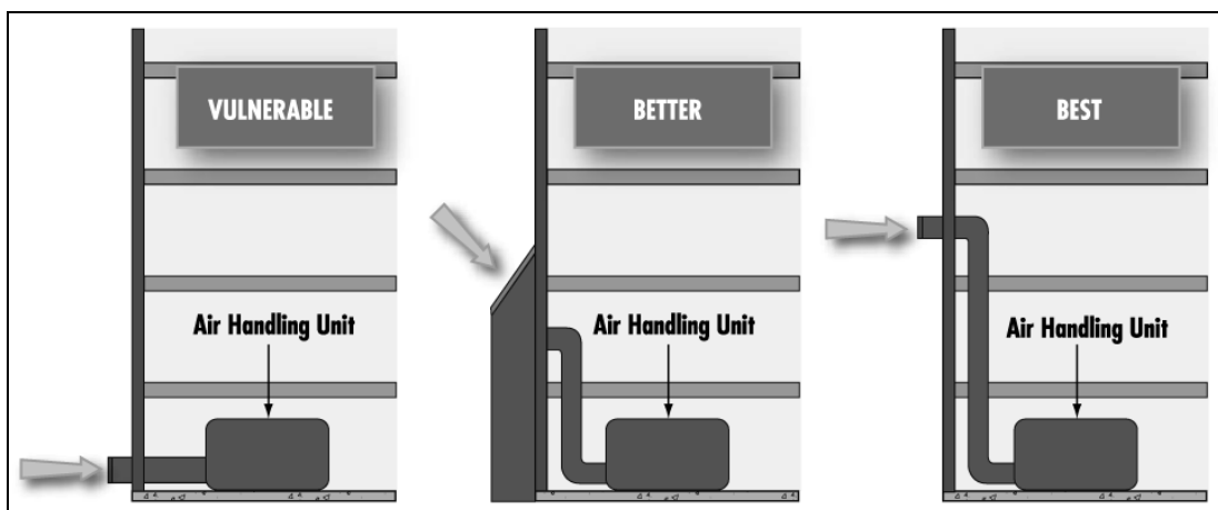
Figure 51. Protecting air intakes (CDC/NIOSH 2002).
