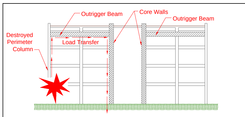
Figure 25. Outrigger beam and belt load-carrying system.
