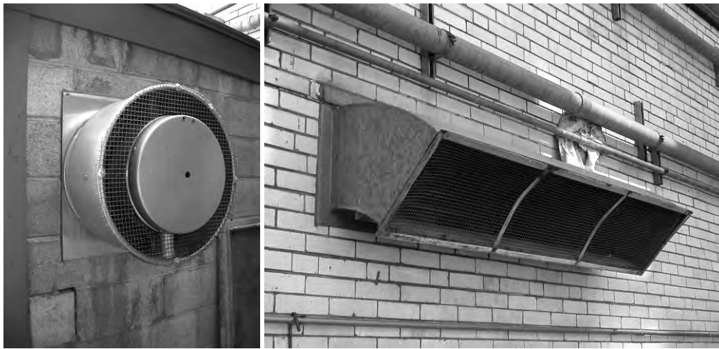
Figure 54. Exhaust vents come in various configurations and should be selected to blend with the historic architecture (ERDC-CERL 2005).
