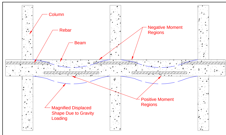
Figure 26. Typical reinforced concrete beam design for normal gravity loading.
