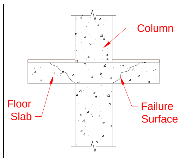
Figure 22. Conceptual diagram of punching shear.
