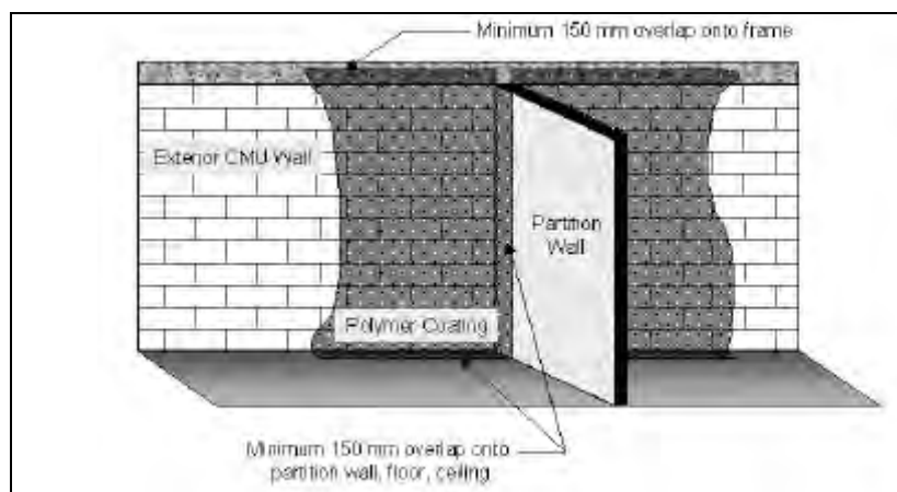
Figure 34. Polymer coating overlapping structural components (ETL 02-4).
