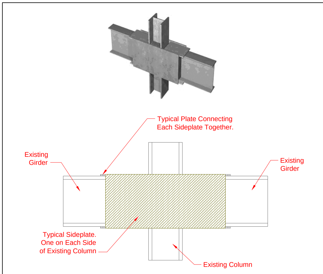
Figure 20. Enhanced structural steel connection (upper illustration Houghton and Karns 2001).
