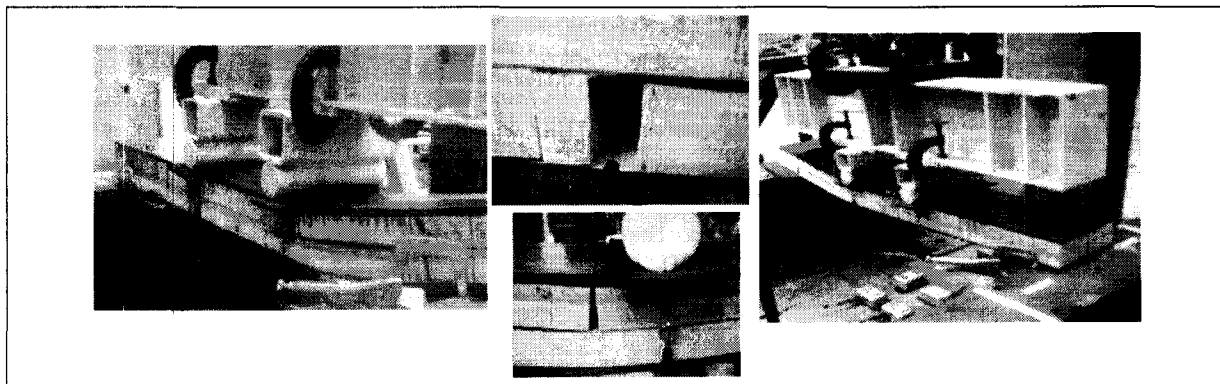
Figure 24 Progression of Failure in the Repaired Specimen
