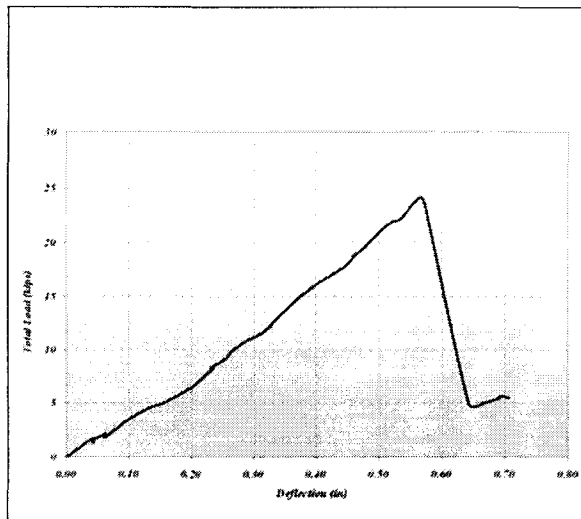
Figure 15 Load vs. Deflection Undamaged
