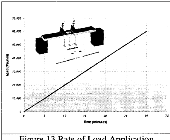
Figure 13 Rate of Load Application
