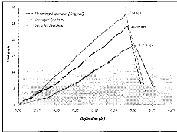
Figure 23 Load vs. Deflection: All
