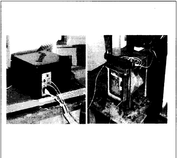
Figure 5 FSI and optical fiber sensors
