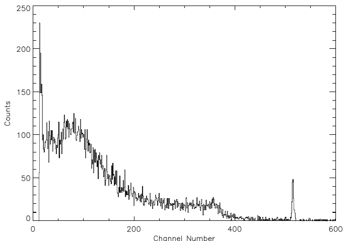
Figure 3: Spectrum of 662 keV photons from ^{137}\text{Cs} as detected by a single strip in amorphous-contact detector. Combining energies from multi-strip events increases the “photopeak” to Compton ratio.
