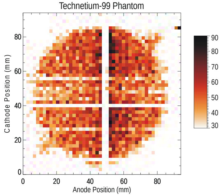
Figure 6. Image of ^{99}\text{Tc} phantom measured at 140 keV with the detector from the previous figure and a collimator. Uniform disk of 8 cm diameter of source material. Fill tubes are seen in upper right and lower left corners.
