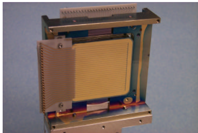
Figure 1. Germanium detector with amorphous contacts. Each side has 25 strips with 2 mm pitch and 5 cm length. Both sides have a guard ring. The detector is held by a germanium lip extending out beyond the guard ring.
