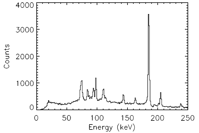
Figure 9. Complete ^{235}\text{U} spectrum measured while collecting the image in the previous figure. The image is in the gamma ray line at 185 keV only.
