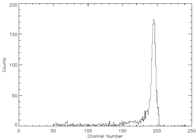
Figure 2: Spectrum of 60 keV photons from ^{241}\text{Am} as detected by a single strip. The low energy shoulder is due to passive material between the source and the detector.
