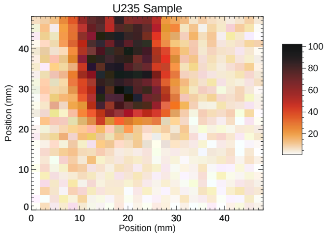
Figure 8. Image of ^{235}\text{U} sample from previous figure as measured in 185 keV gamma rays. Image pixels are 2 \times 2 mm.
