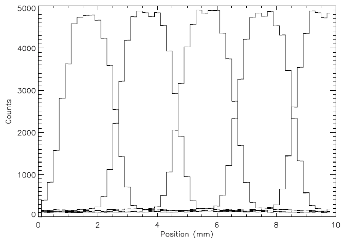
Figure 4: Scan of 60 keV photon beam across a face of the detector. The \sim 500 micron-wide beam was scanned in steps of \sim 200 microns. The leftmost strip is the edge strip, showing no strip distortions even for the edge strip.
