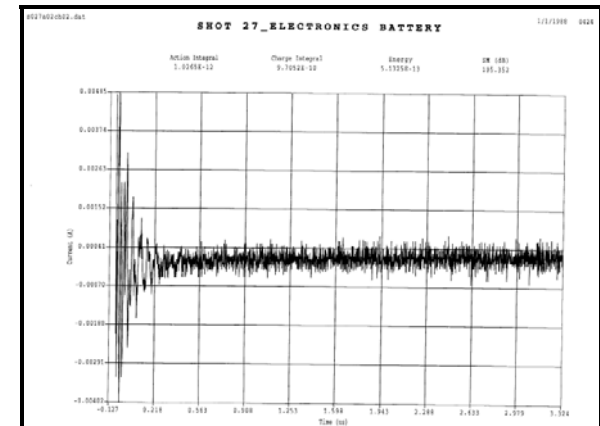
Figure N-13. Example EID current data plot.
