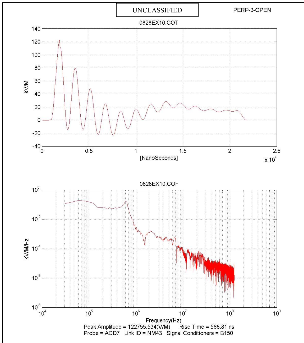
Figure C-6. Sample tailored environmental wave form.
