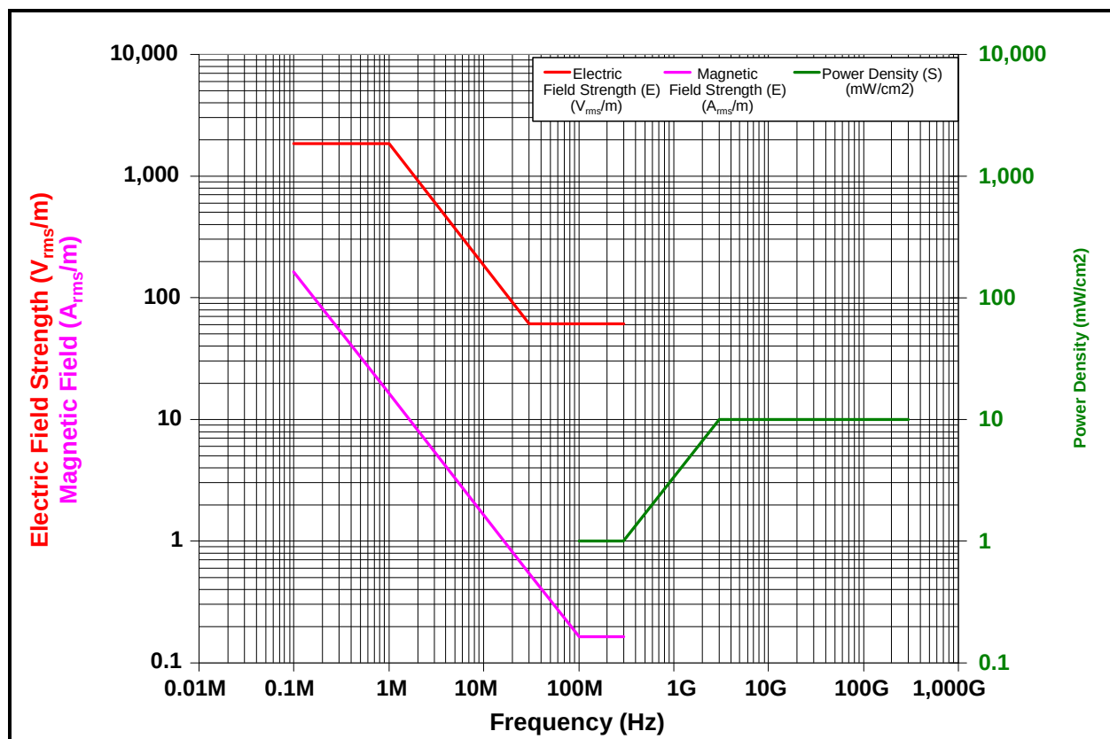
Figure 1. MPEs based on IEEE C95.1-2005 for controlled environments.
