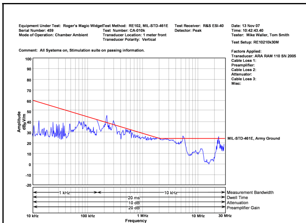
Figure K-4. Sample emissions data plot.
