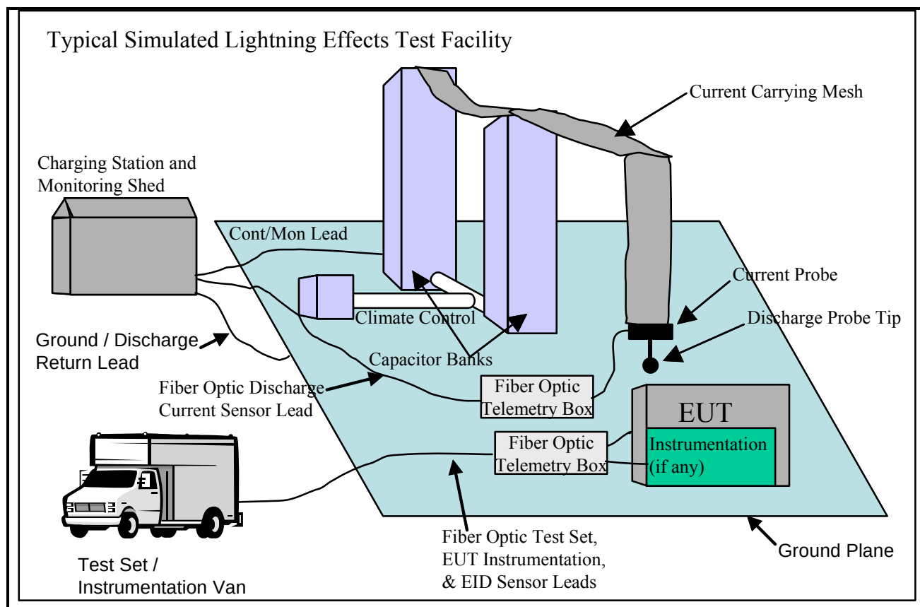
Figure C-2. Typical NSL test setup.
