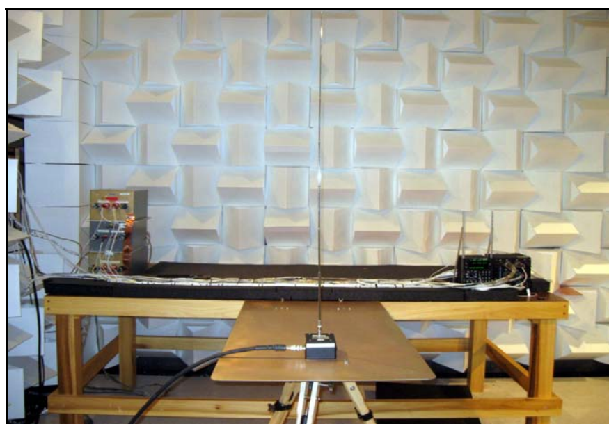
Figure K-5. Sample emissions set-up photo for MIL-STD-461E.
