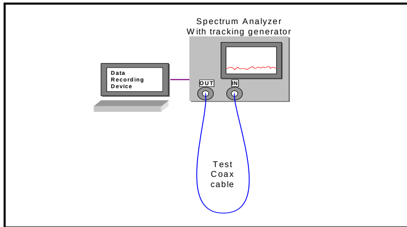
Figure A-3. Cable loss test setup.
