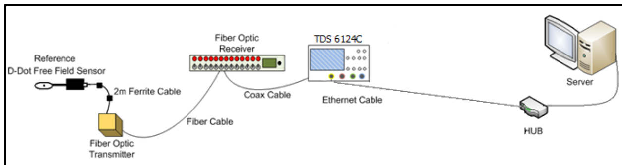
Figure J-1. Fiber optic configuration example.
