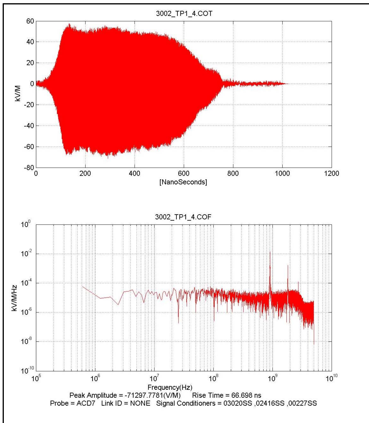
Figure J-5. Narrowband signal reference probe data.
