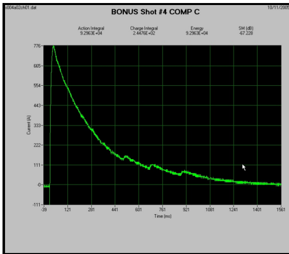
Figure N-10. Example component C test waveform.
