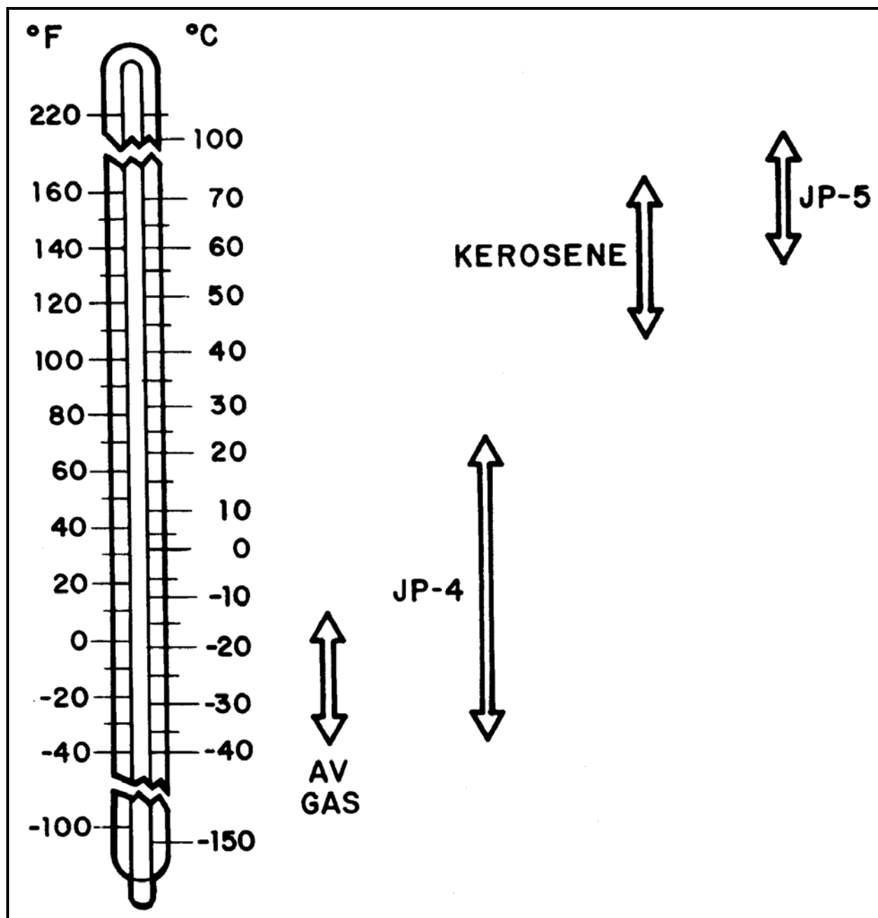
Figure G-2. Temperature-flammability ranges for fuels.
