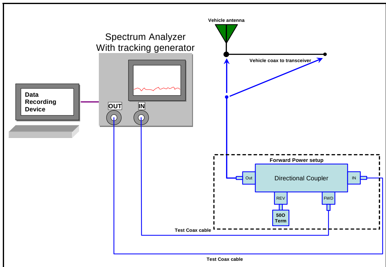
Figure A-4. Forward power test setup.
