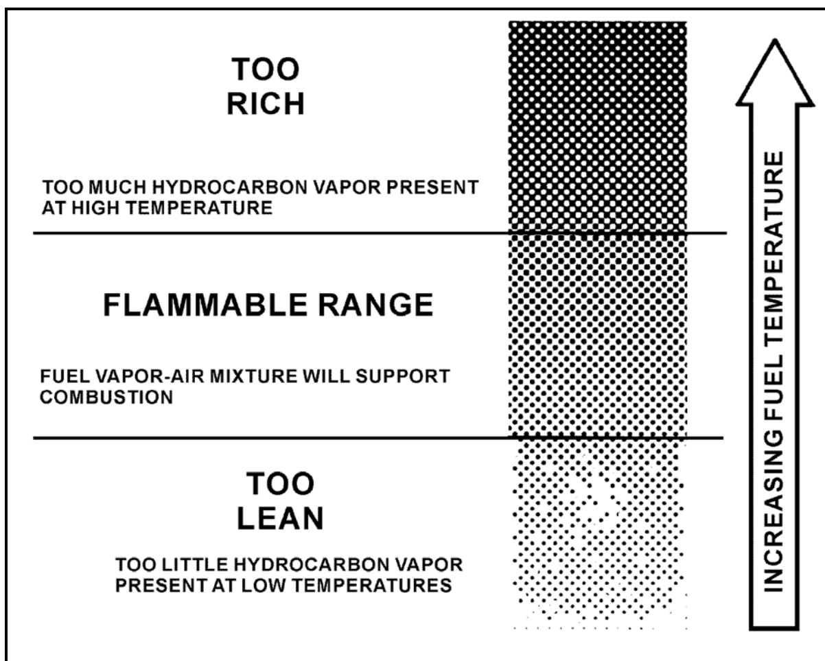
Figure G-1. Effect of temperature in generating hydrocarbon fuel flammable vapors.
