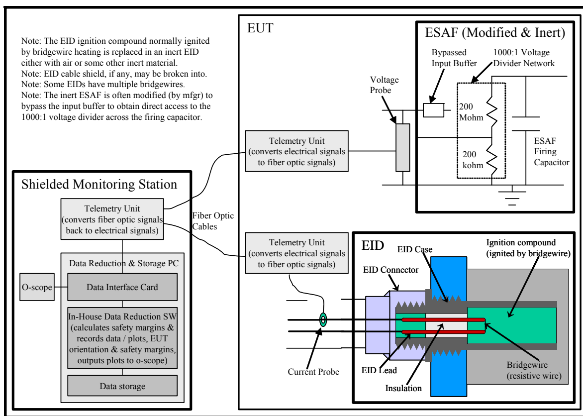
Figure E-1. Typical instrumentation block diagram.
