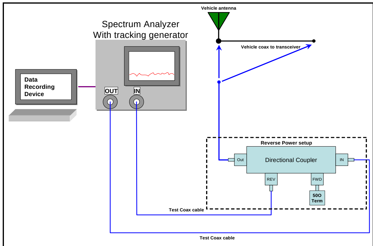
Figure A-5. Reverse power test setup.
