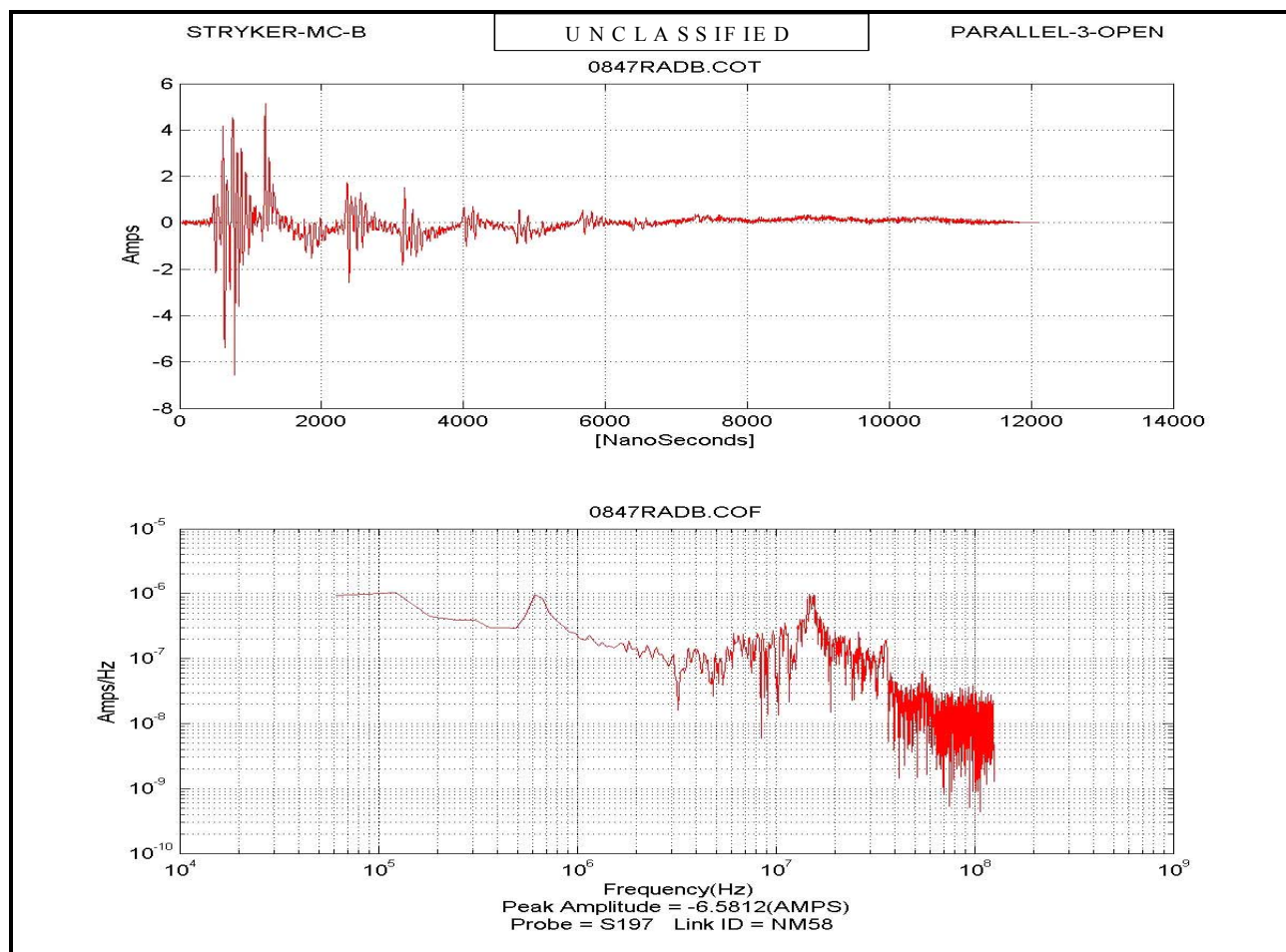
Figure C-5. Sample induced current waveform.
