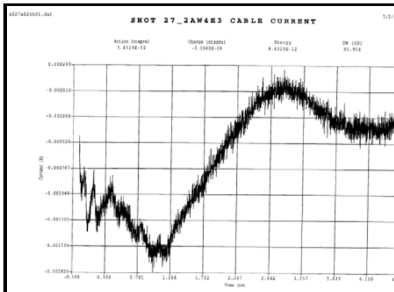
Figure N-12. Example cable current data plot.
