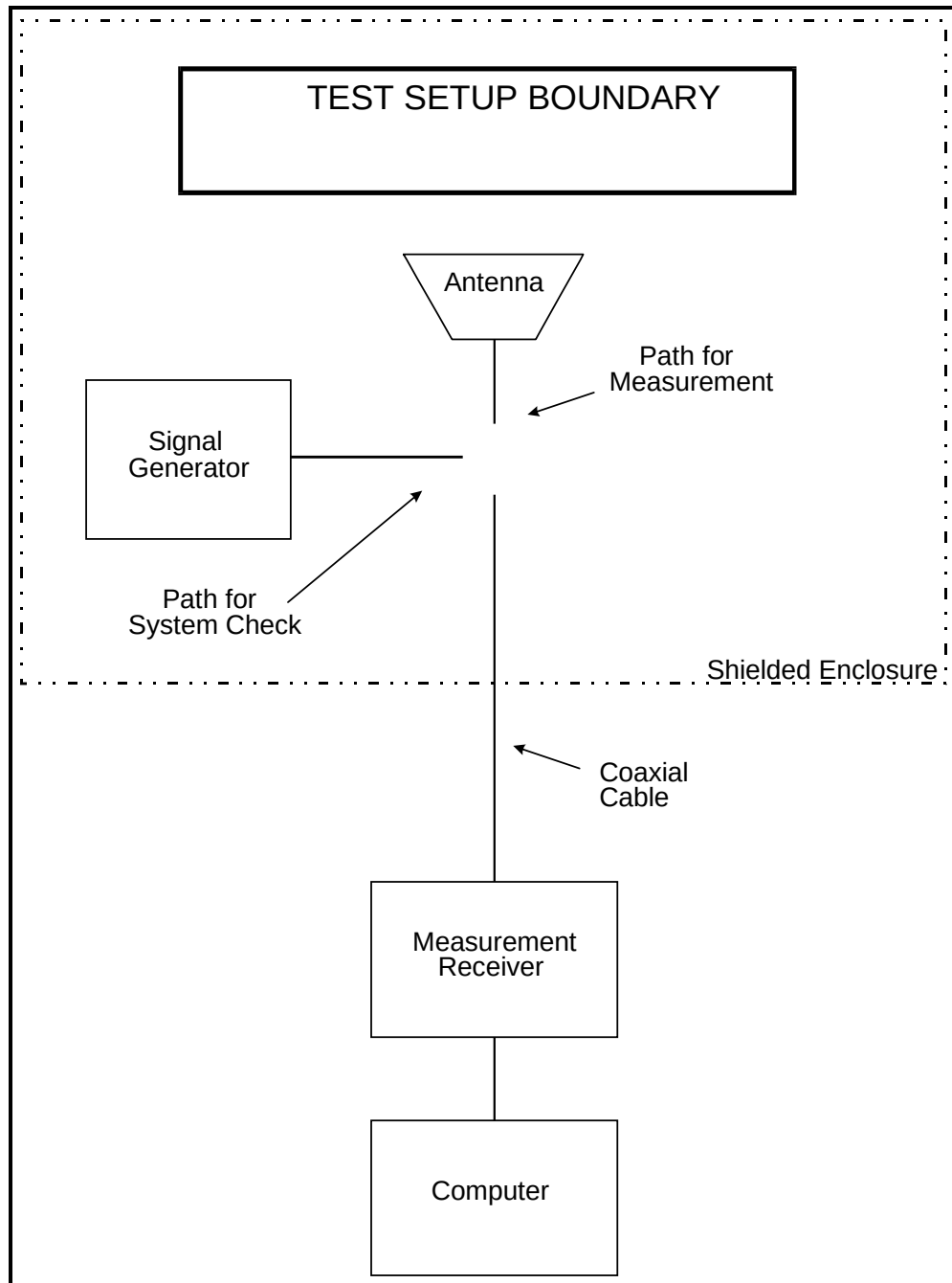
Figure K-1. System emissions basic test setup.
