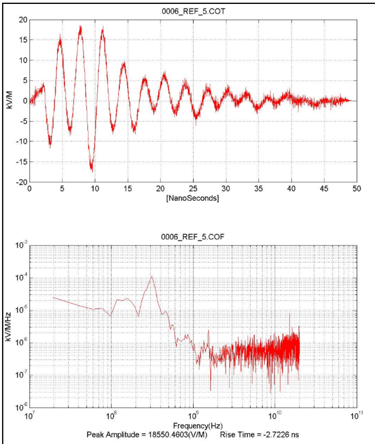
Figure J-6. Wideband signal reference probe data.
