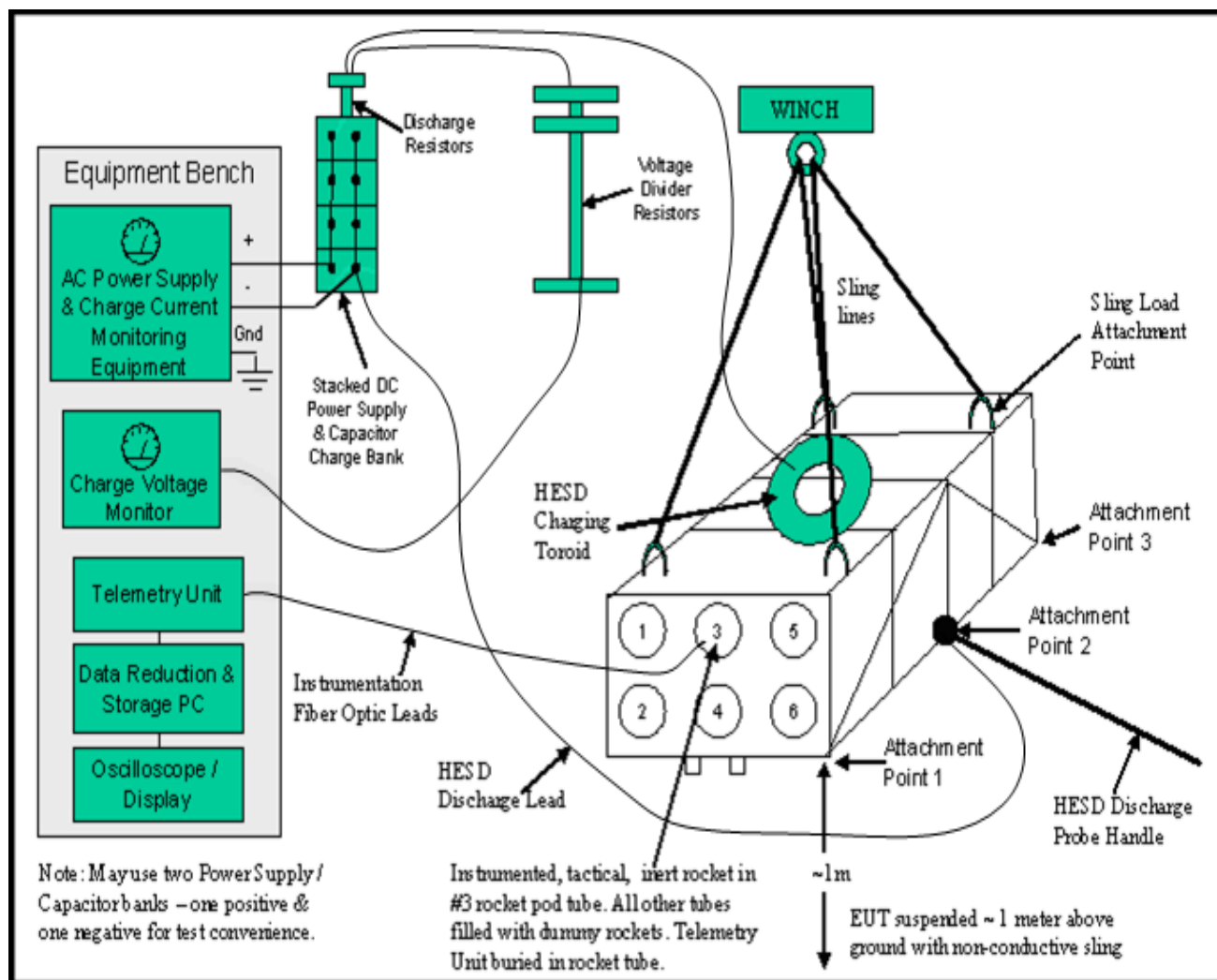
Figure E-2. Typical HESD test setup.
