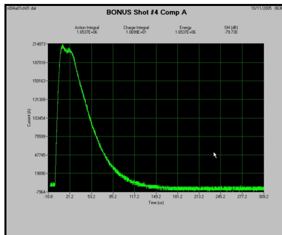
Figure N-9. Example component A test waveform.
