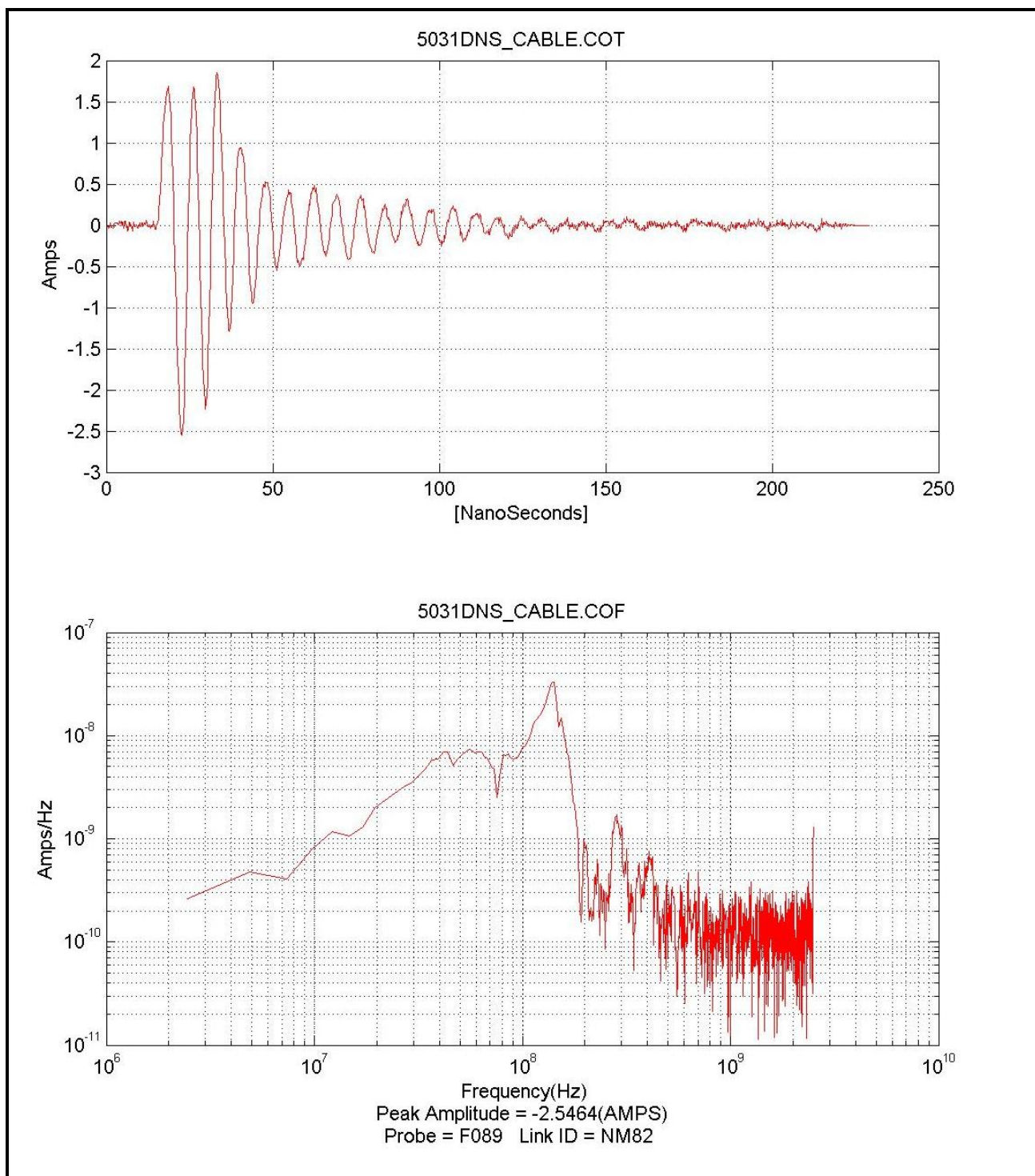
Figure D-2. Typical EMP data plots.
