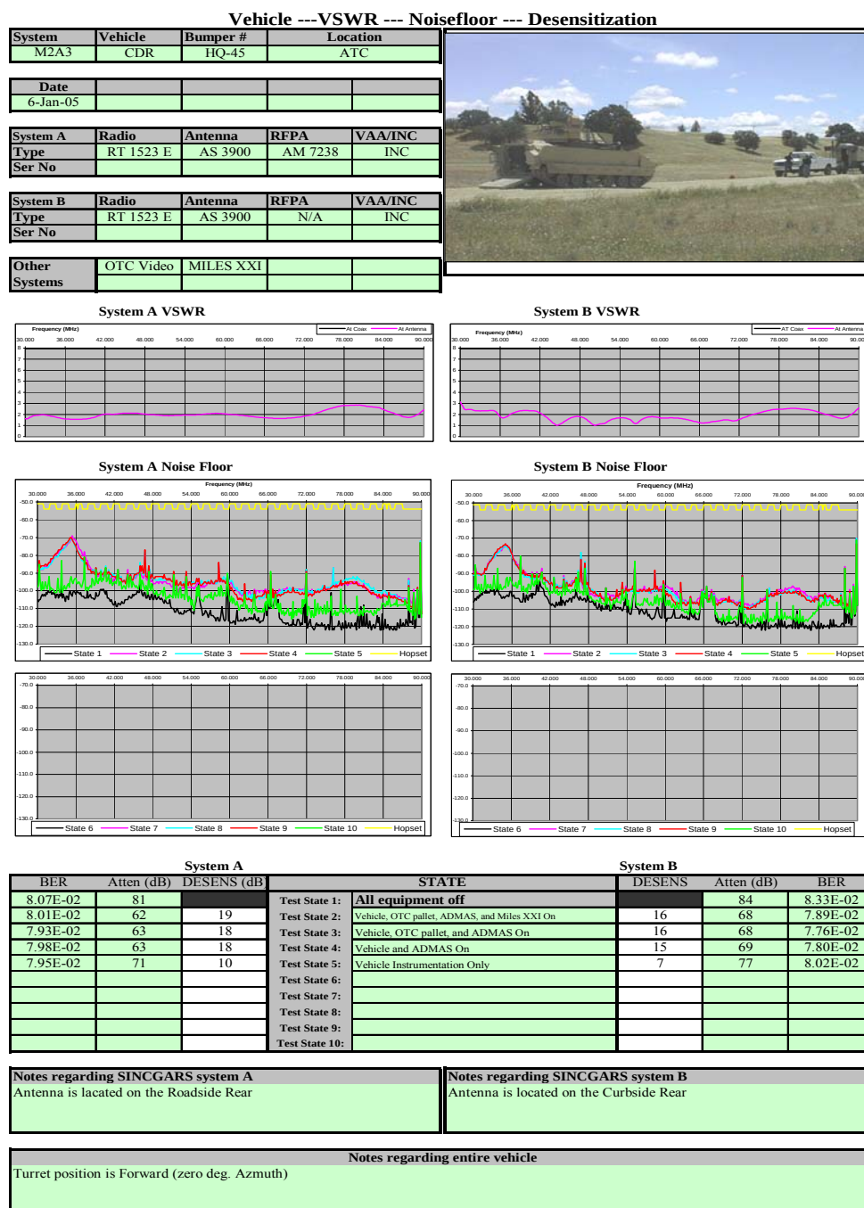
Figure A-7. Example SINCGARS desensitization data sheet.
