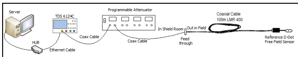
Figure J-2. Coaxial cable configuration for example.
