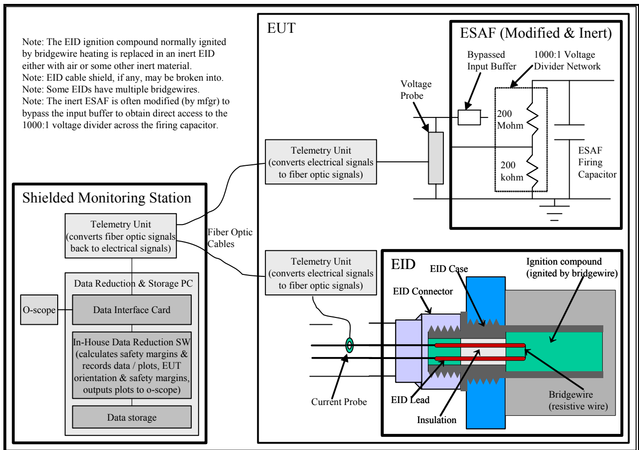
Figure N-2. Typical instrumentation block diagram.
