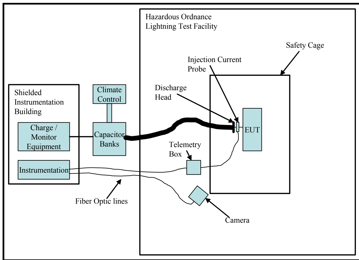
Figure N-4. DSL test facility typical test setup for testing hazardous ordnance.
