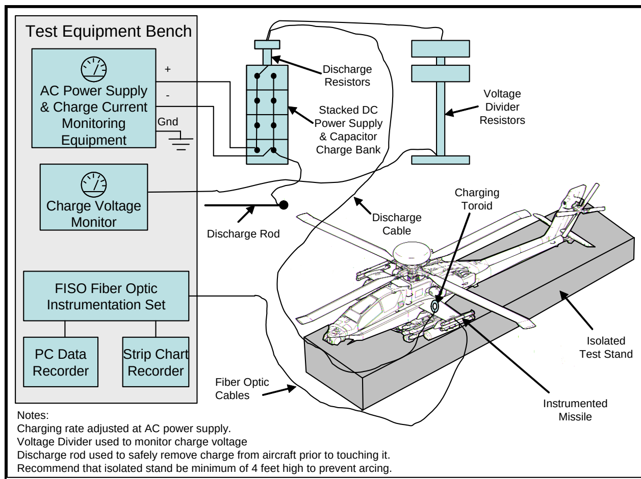
Figure F-2. Typical P-static test setup.
