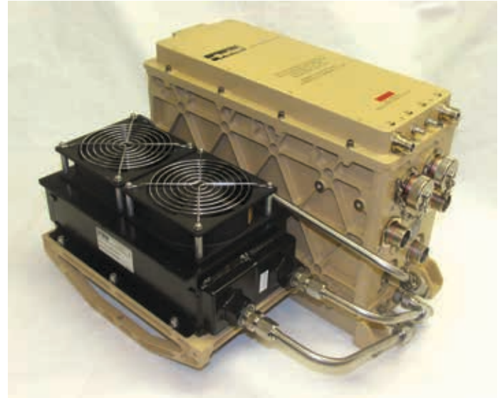
ABOVE AND RIGHT: The Laboratory is developing a novel ground-penetrating radar capability to be used by combat engineers. An initial prototype has been integrated onto an Army Husky vehicle.
