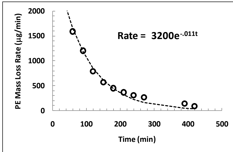
Figure 1. Propyl ether mass loss rate versus time and logarithmic correlation equation.
