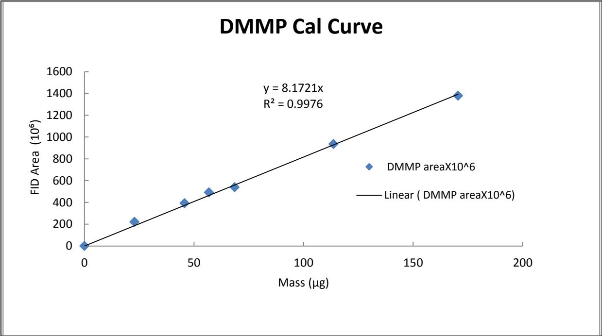
Figure C-3. DMMP calibration.
