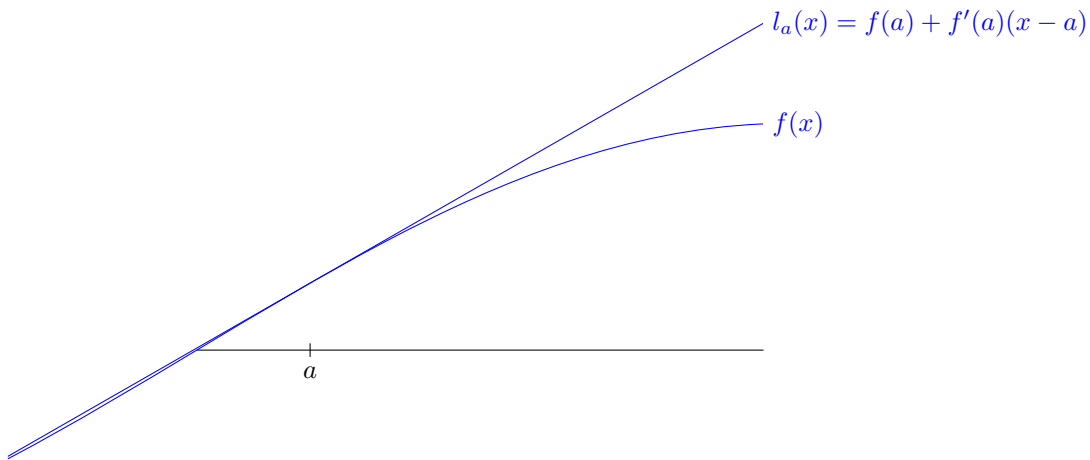
Figure A.1 Approximation by a Tangent Line
