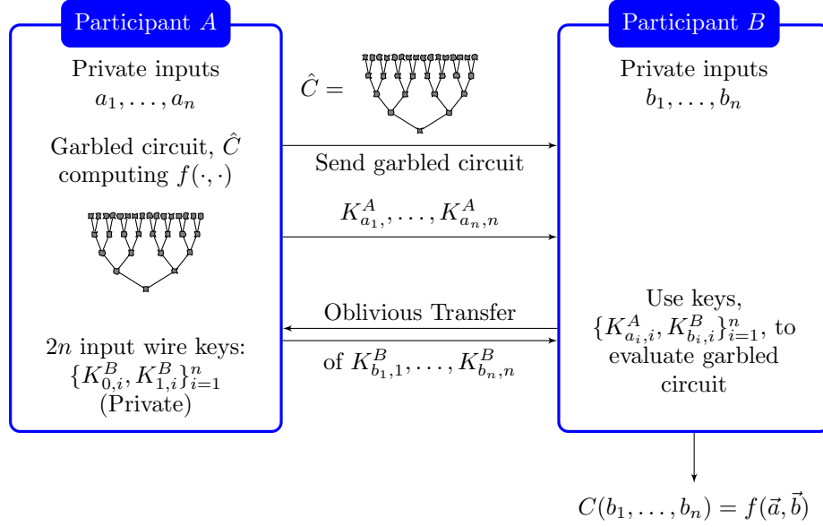
Figure 2.3 Garbled Gate
