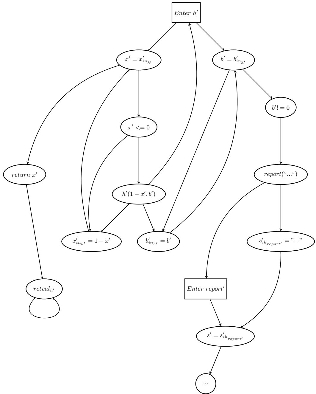
Fig. 7. The System Definition Graph [HRB90] of the sub-program starting in function h' , defined in Fig 5.
