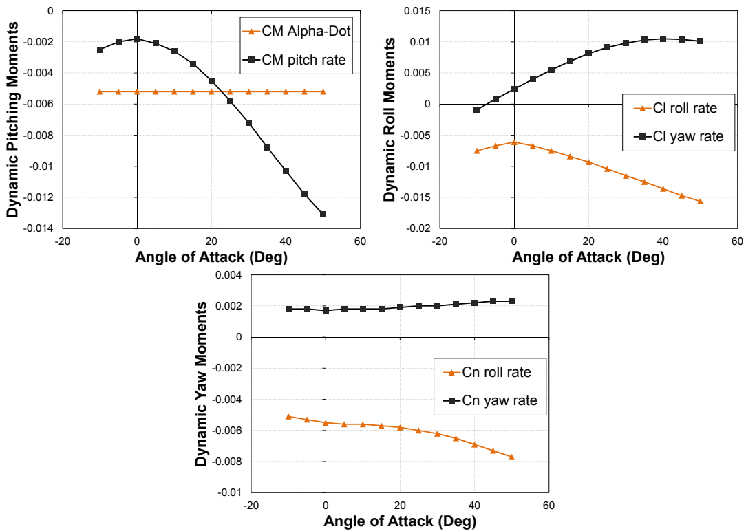
Figure 13. Dynamic Derivatives for Mach 1.5.
