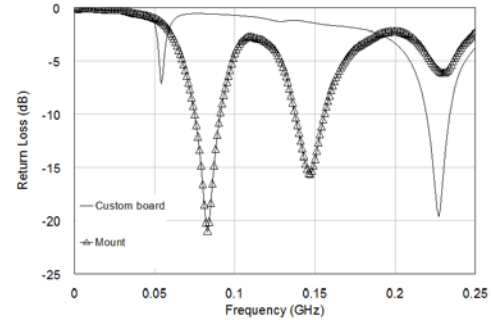
Figure 6: Clock pin RL (dB) for both boards.
