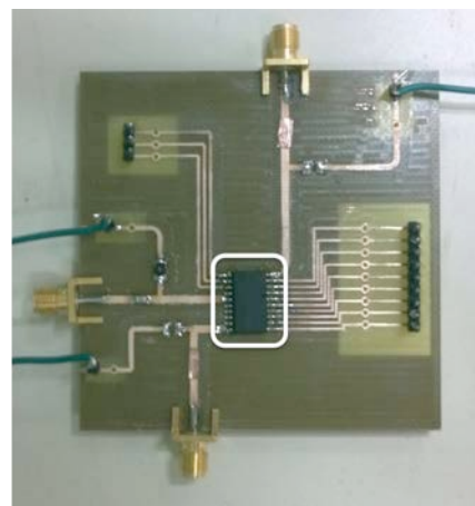
Figure 2: Custom board.
