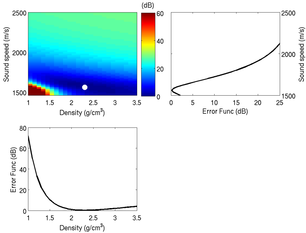
Figure 11: Ambiguity surface of the error function (cost or objective function) as a function of sediment sound speed and density as the geoacoustic parameters are swept one at a time. The attenuation is held at the optimum value of 0.7 dB/λ. Cross-sections pass through the white dot, with sound speed fixed (lower left) and with density fixed (upper right).
