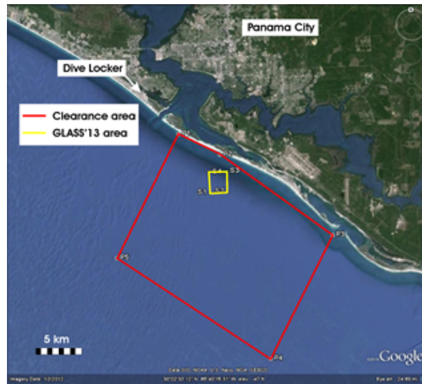
Figure 1: Clearance area (red box) defined for the TREX experiment in the Gulf of Mexico off the coast of Panama City, Florida, USA. The yellow box indicates the operational area during the GLASS'13.
