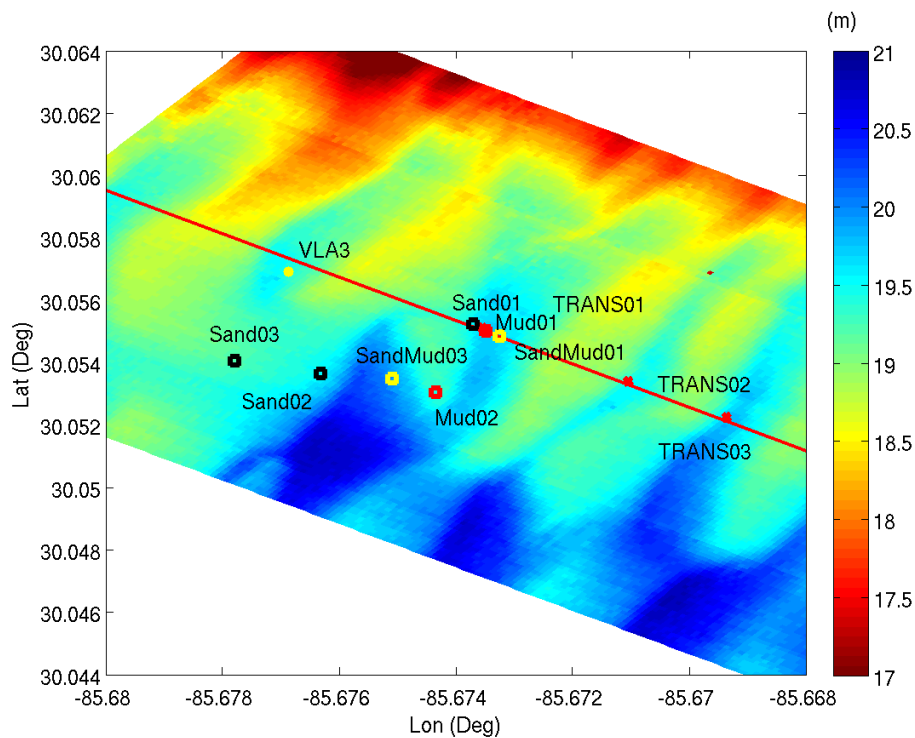
Figure 2: Bathymetry along the TREX main reverberation track (red line) obtained by a calibrated multi-beam system survey during the TREX experiment [10]. The undulations in the bathymetry along the main reverberation track have been shown to correlate with backscattering strength
