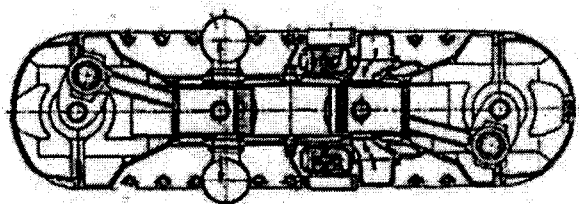
Figure 1: JUMO Diesel Opposed-Piston Engine
