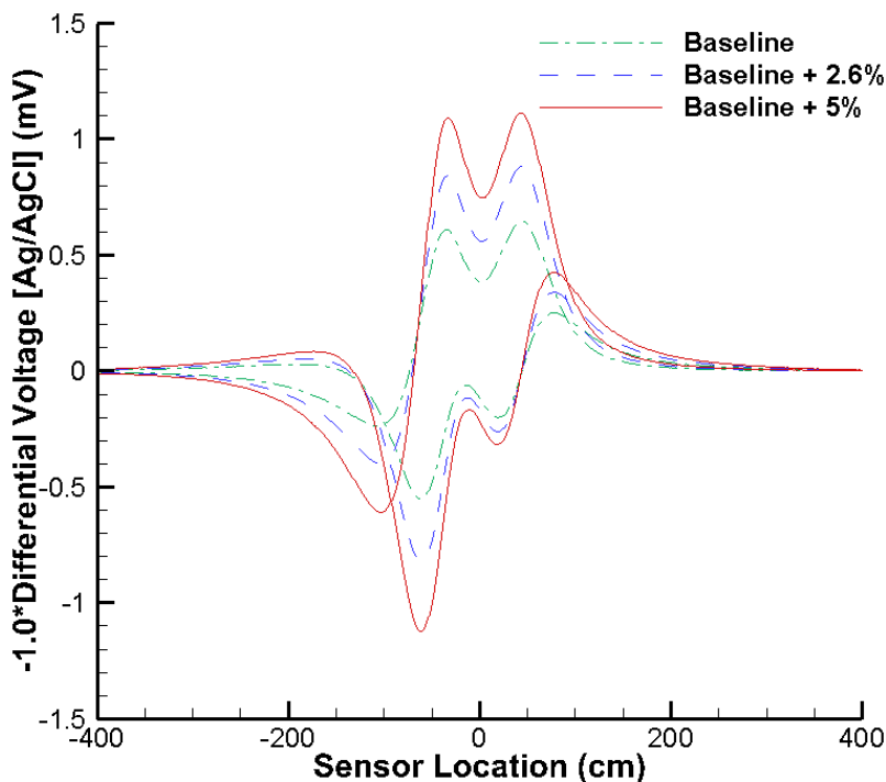
Figure 6-4. Comparison of calculated electric potential differential for various amounts of damage.
