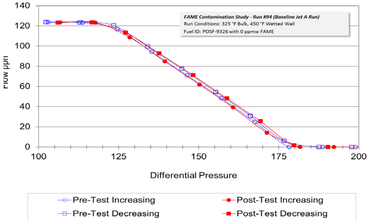
Figure D- 3 Servo Valve Hysteresis, Run 94, Baseline, LT Temperature Profile
