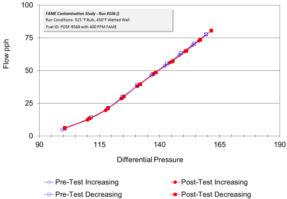
Figure E- 17 FDV Hysteresis, Run 106, FAME, HT+ Temperature Profile, EDTST Protocol
