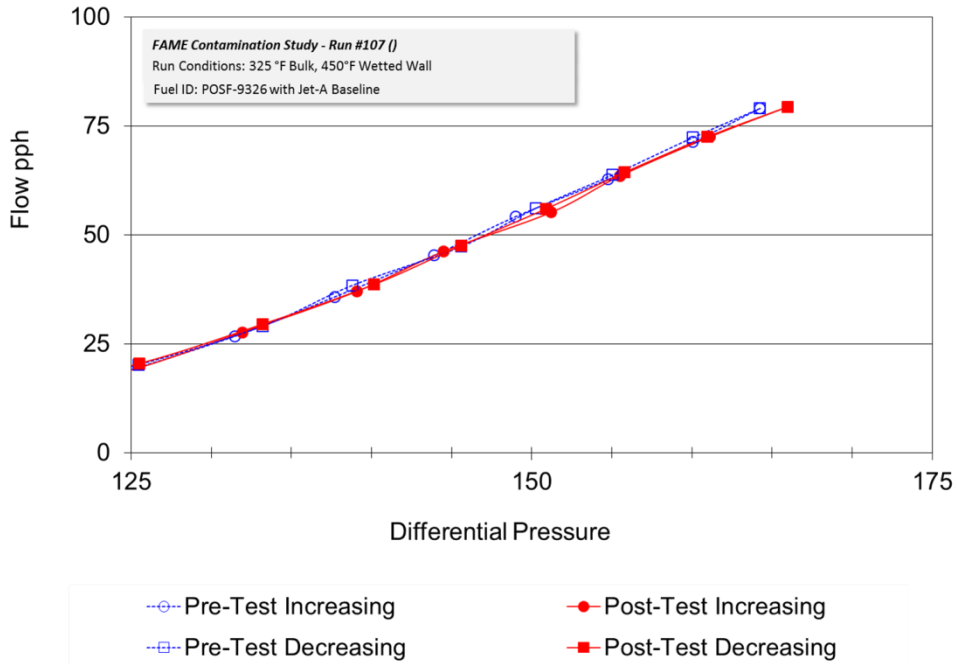
Figure E- 15 FDV Hysteresis, Run 107, Baseline, HT+ Temperature Profile, EDTST Protocol
