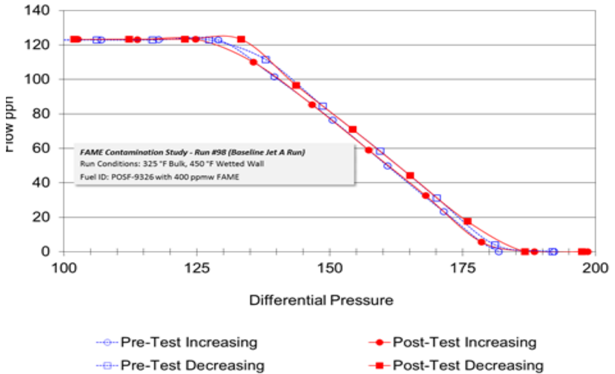
Figure D- 7 Servo Valve Hysteresis, Run 98, 400 PPM FAME, LT Temperature Profile
