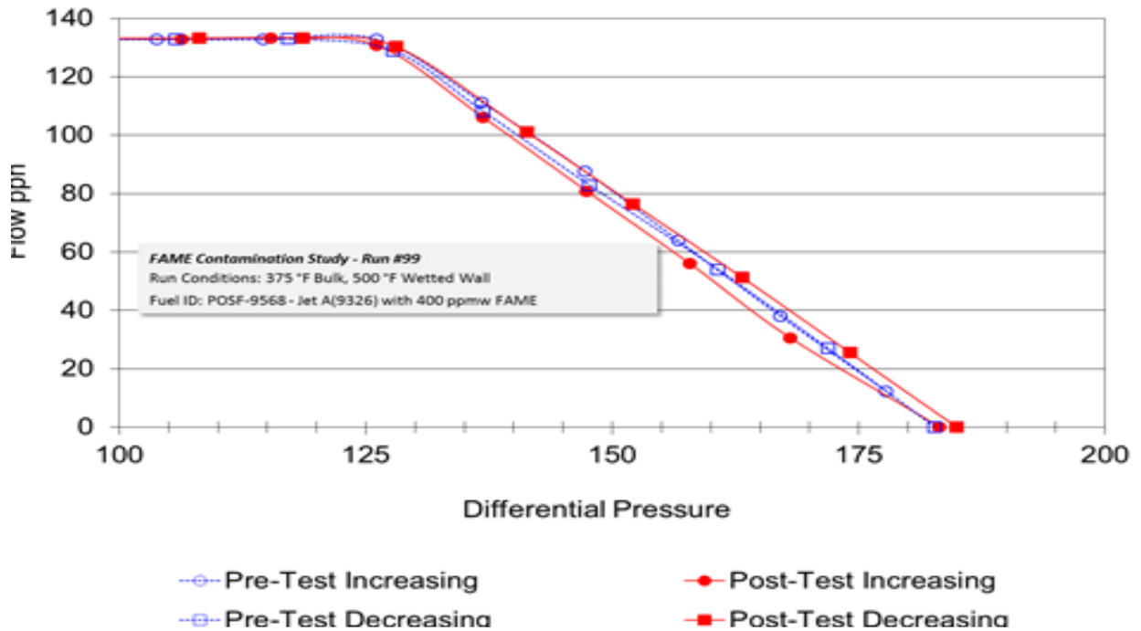
Figure D- 8 Servo Valve Hysteresis, Run 99, 400 PPM FAME, HT Temperature Profile
