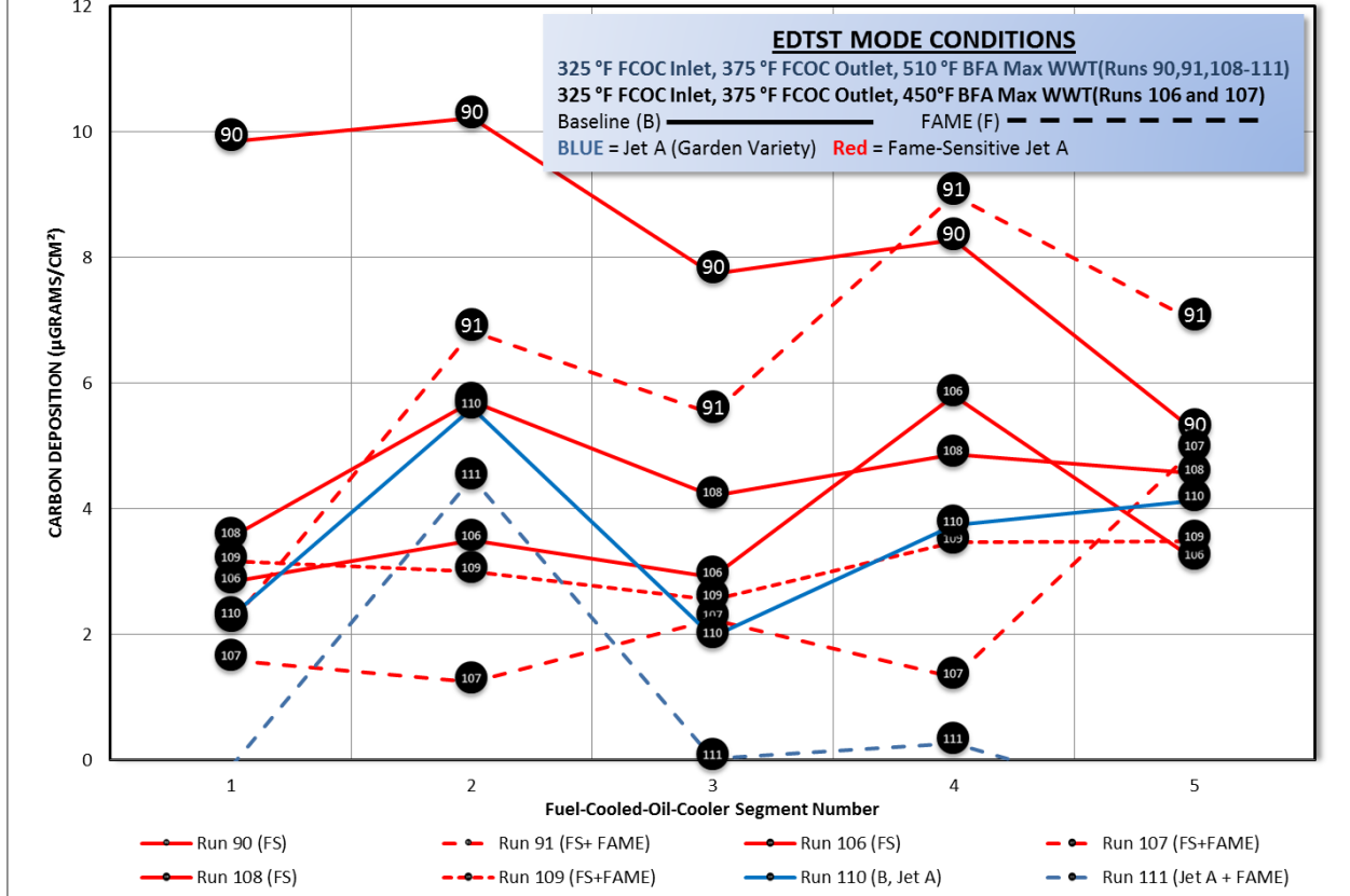
Figure 35 – FCOC Carbon Deposition in FAME-Sensitive and Typical Jet A
