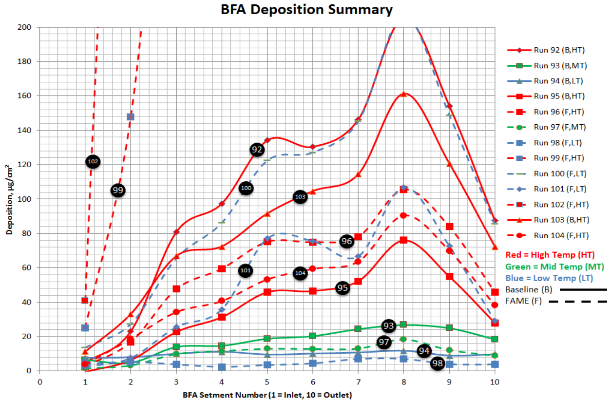
Figure 17 – Composite of All BFA Deposition Data
