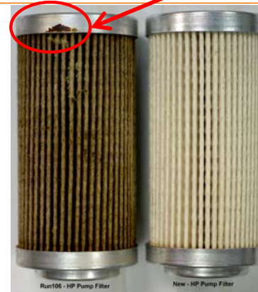
Figure G-2 – HP Pump Filter Comparison, EDTST Protocol, HT+ Conditions
