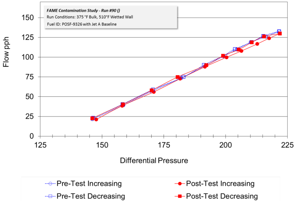
Figure E- 14 FDV Hysteresis, Run 90, Baseline, HT+ Temperature Profile, EDTST Protocol
