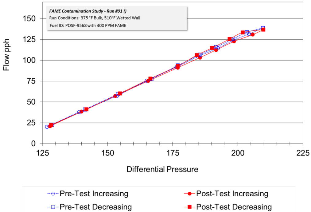
Figure E- 16 FDV Hysteresis, Run 91, FAME, HT+ Temperature Profile, EDTST Protocol
