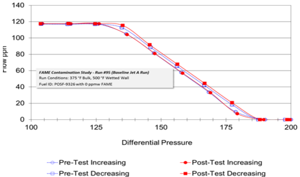
Figure D- 4 Servo Valve Hysteresis, Run 95, Baseline, HT Temperature Profile (Repeat of Run 92)
