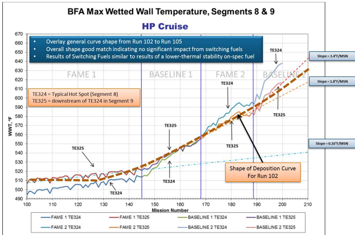
Figure 27 – Curve Shape of Run 102 Overlaid on BFA WWT Curve Run 105
