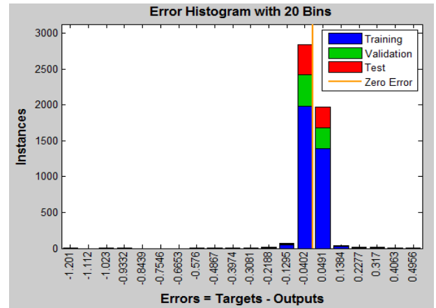
Fig. 6. Error Histogram with 20 Bins
