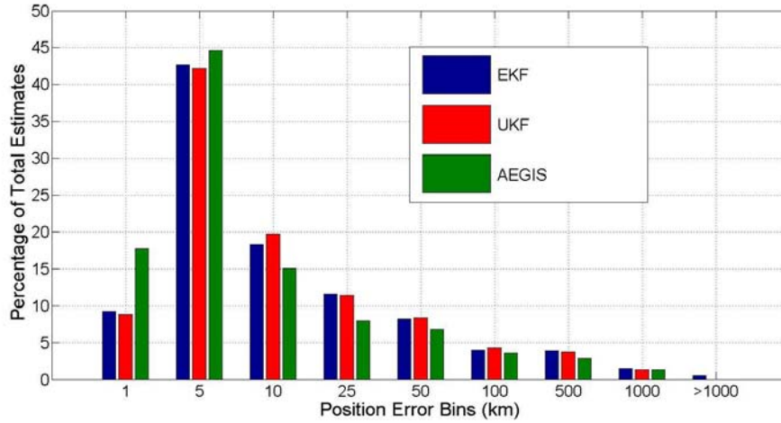
Figure 66. EKF, UKF, and AEGIS histograms of position estimate error distributions for SIG simulation. Plots include data from all objects at all simulation time steps.
