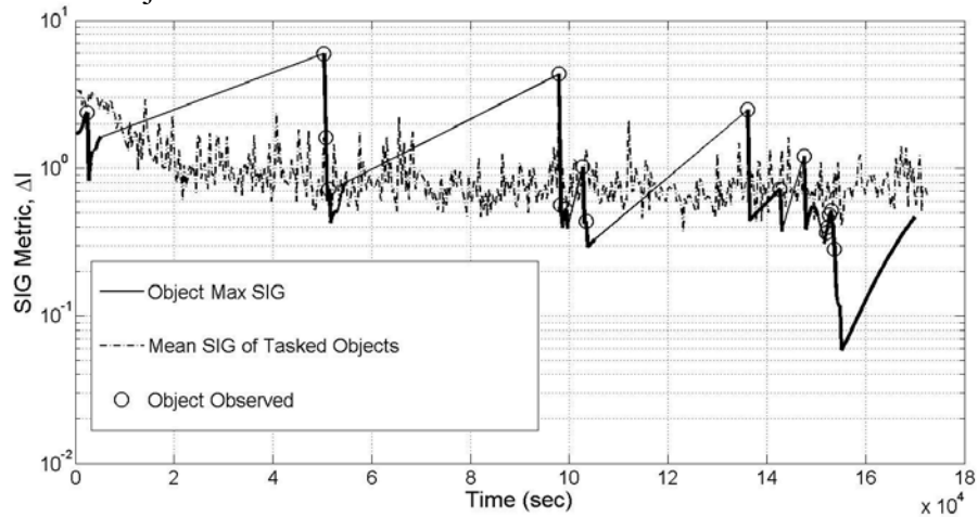
Figure 73. Plot of the SIG utility metric \Delta I and tasking decisions for object 39 using SIG tasking strategy in conjunction with an EKF. Thick sections of line reflect times when observations were available between that object and one or more sensors.
