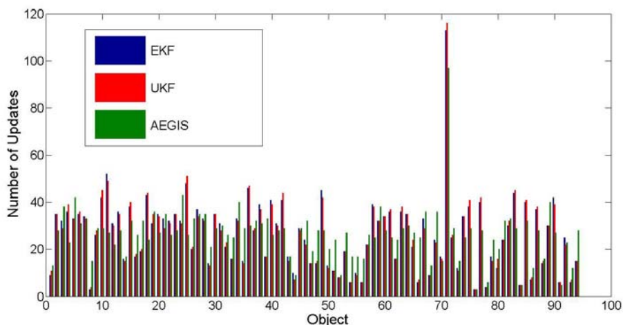
Figure 69. Bar graphs showing the updates each object received through implementation of an EKF, UKF, and AEGIS filter in conjunction with a SIG tasking strategy.
