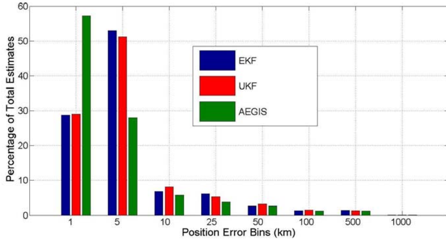
Figure 14. EKF, UKF, and AEGIS histograms of position estimate error distributions for all data simulation. Plots include data from all objects at all simulation time steps.
