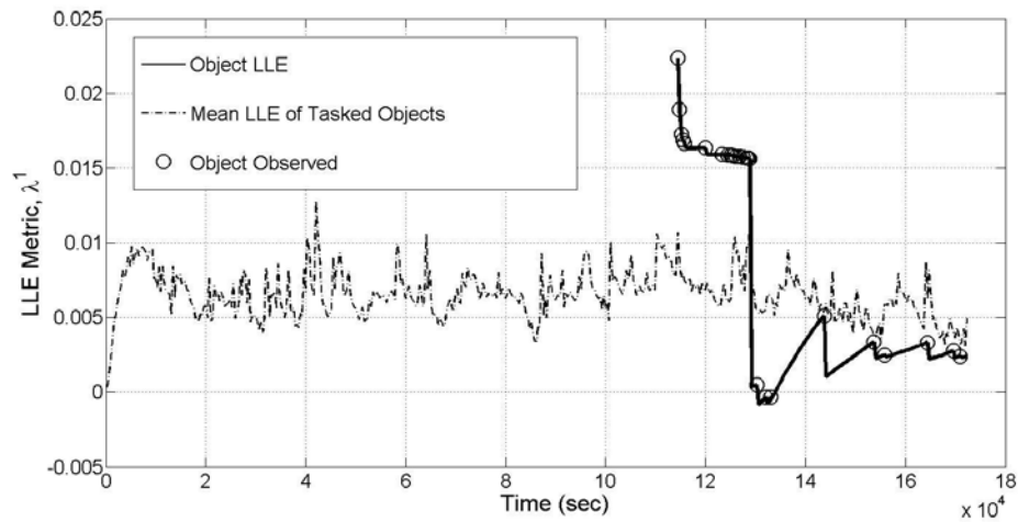
Figure 47. Plot of the LLE utility metric \hat{\lambda}^1 and tasking decisions for object 21 using the LLE tasking strategy in conjunction with an EKF. Thick sections of line reflect times when observations were available between that object and one or more sensors.
