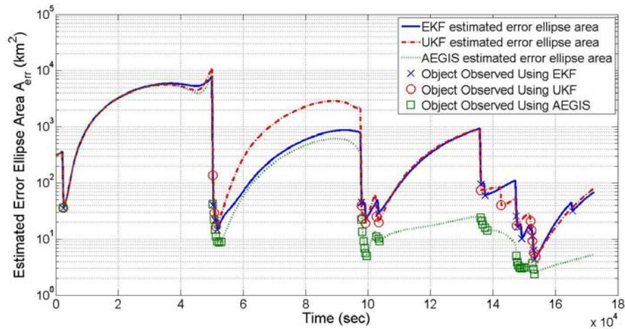
Figure 76. EKF, UKF, and AEGIS plots of \hat{A}_{err} = \pi \sqrt{\zeta_{i,k}^1 \zeta_{i,k}^2} metric for object 39 in the SIG simulation.
