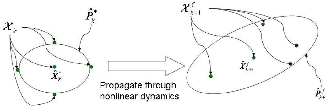
Figure 8. Illustration of propagation of sigma points through nonlinear object equations of motion to calculate forecast state and covariance estimates. The ellipses represent a 3\sigma Gaussian error ellipse, which can be obtained from the covariance estimate \hat{P}_k^* and \hat{P}_{k+1}^f
