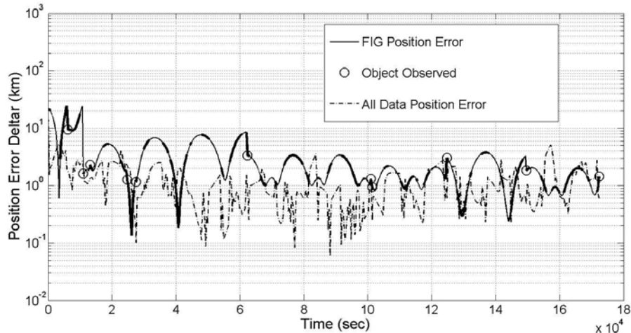
Figure 62. Plot of the position error \Delta r_{i,k} and tasking decisions for object 59 using FIG tasking strategy in conjunction with an AEGIS filter. Thick sections of line reflect times when observations were available between object 59 and one or more sensors.
