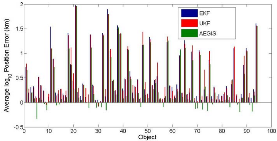
Figure 31. Bar graphs showing the \log_{10} average position error for each object given in Equation 200, through implementation of an EKF, UKF and AEGIS filter in conjunction with a SIG tasking strategy.
