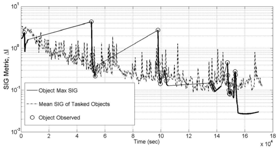
Figure 75. Plot of the SIG utility metric \Delta I and tasking decisions for object 39 using SIG tasking strategy in conjunction with an AEGIS filter. Thick sections of line reflect times when observations were available between that object and one or more sensors.
