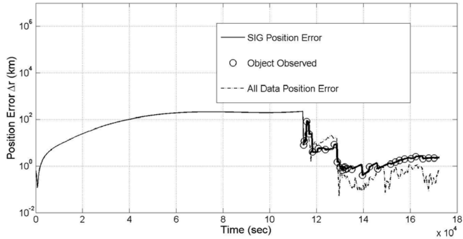
Figure 34. Plot of the position error \Delta r_{i,k} and tasking decisions for object 21 using SIG tasking strategy in conjunction with a UKF. Thick sections of line reflect times when observations were available between object 21 and one or more sensors.
