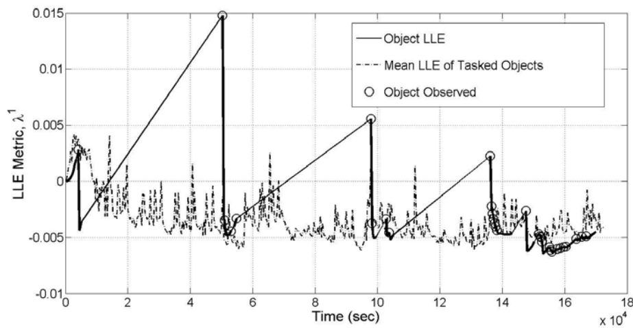
Figure 84. Plot of the LLE utility metric \hat{\lambda}^1 and tasking decisions for object 39 using LLE tasking strategy in conjunction with an EKF. Thick sections of line are times at which observations were available between that object and one or more sensors.
