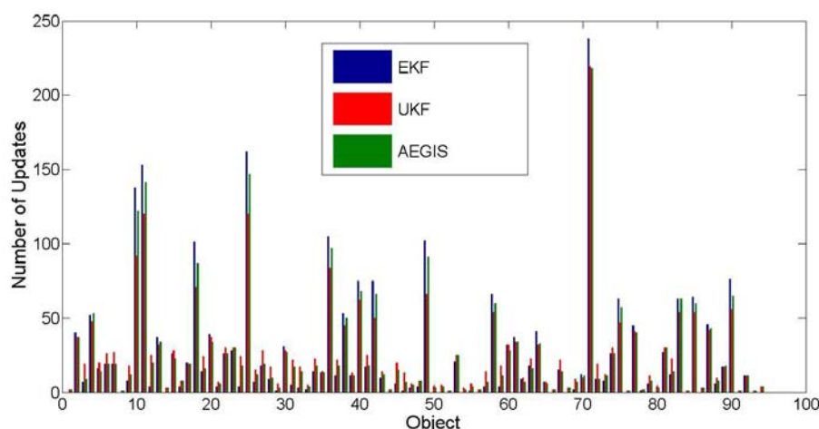
Figure 59. Bar graphs showing the updates each object received through implementation of an EKF, UKF, and AEGIS filter in conjunction with a FIG tasking strategy. As with the low-error scenario, the FIG tasking results in many updates to a select few objects, while many other objects receive little to none.
