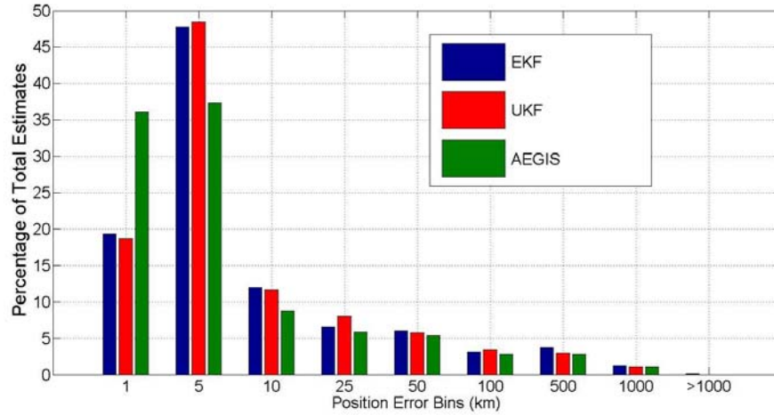
Figure 51. EKF, UKF, and AEGIS histograms of position estimate error distributions for all data simulation. Plots include data from all objects at all simulation time steps.
