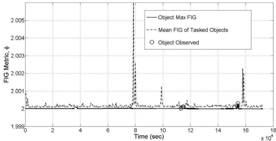
Figure 26. Plot of the FIG utility metric and tasking decisions for object 71 using FIG tasking strategy in conjunction with an EKF. Thick sections of line represent times when observations were available between that object and one or more sensors.
