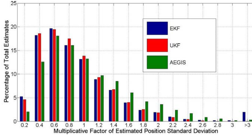
Figure 52. EKF, UKF, and AEGIS histograms of J_{i,k}^P metric in Equation 202 for all data simulation. Plots include data from all objects at all simulation time steps.
