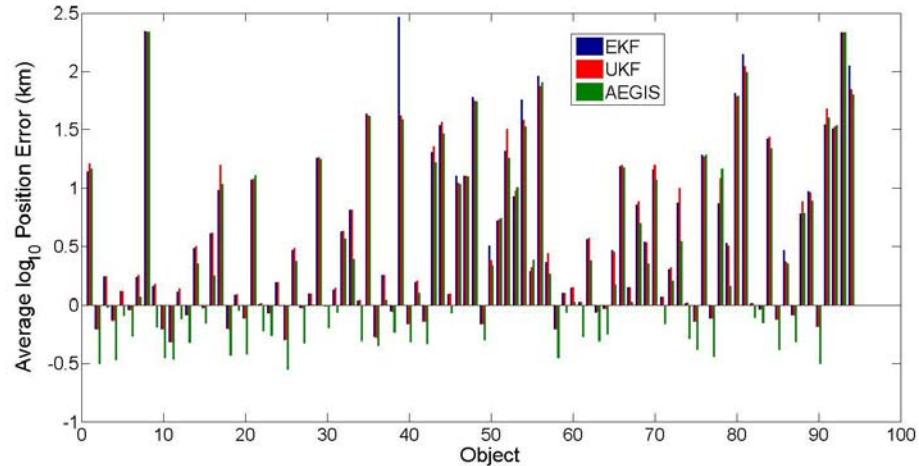
Figure 54. Bar graphs showing the \log_{10} average position error for each object given in Equation 200, through implementation of an EKF, UKF, and AEGIS filter in conjunction with all data tasking strategy. In this case, the filters have equal amounts of updates, reflecting the maximum updates possible for all objects.
