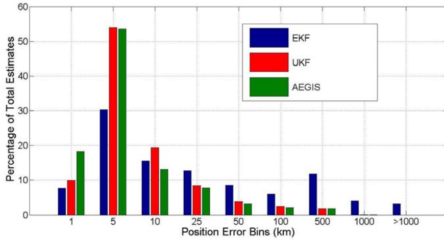
Figure 19. EKF, UKF, and AEGIS histograms of position estimate error distributions for FIG simulation. Plots include data from all objects at all simulation time steps.
