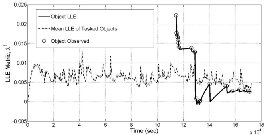
Figure 48. Plot of the LLE utility metric \hat{\lambda}^1 and tasking decisions for object 21 using the LLE tasking strategy in conjunction with a UKF. Thick sections of line reflect times when observations were available between that object and one or more sensors.
