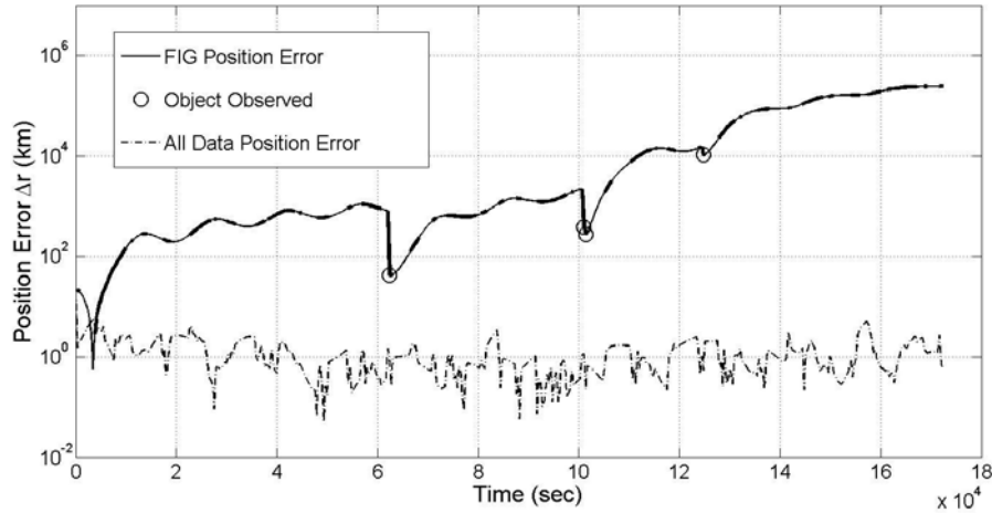
Figure 60. Plot of the position error \Delta r_{i,k} and tasking decisions for object 59 using FIG tasking strategy in conjunction with an EKF. Thick sections of line reflect times when observations were available between object 59 and one or more sensors.
