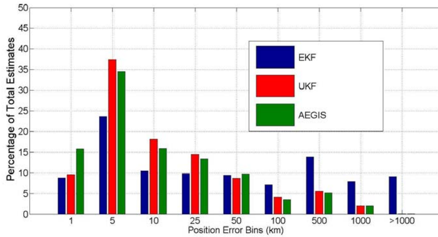
Figure 56. EKF, UKF, and AEGIS histograms of position estimate error distributions for FIG simulation. Plots include data from all objects at all simulation time steps.
