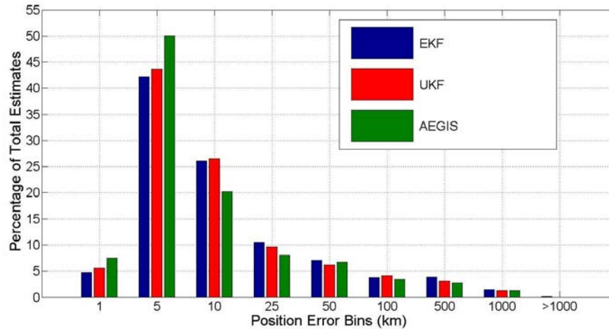
Figure 77. EKF, UKF, and AEGIS histograms of position estimate error distributions for LLE simulation. Plots include data from all objects at all simulation time steps.
