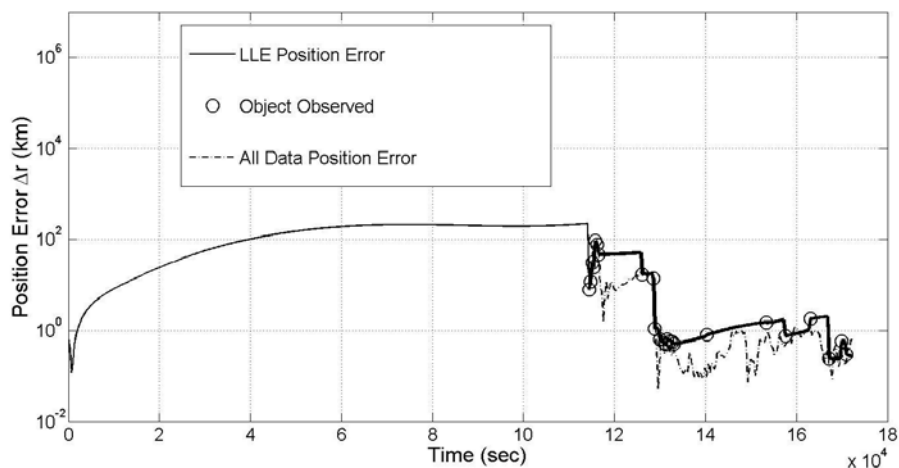
Figure 45. Plot of the position error \Delta r_{i,k} and tasking decisions for object 21 using the LLE tasking strategy in conjunction with a UKF. Thick sections of line reflect times when observations were available between object 21 and one or more sensors.
