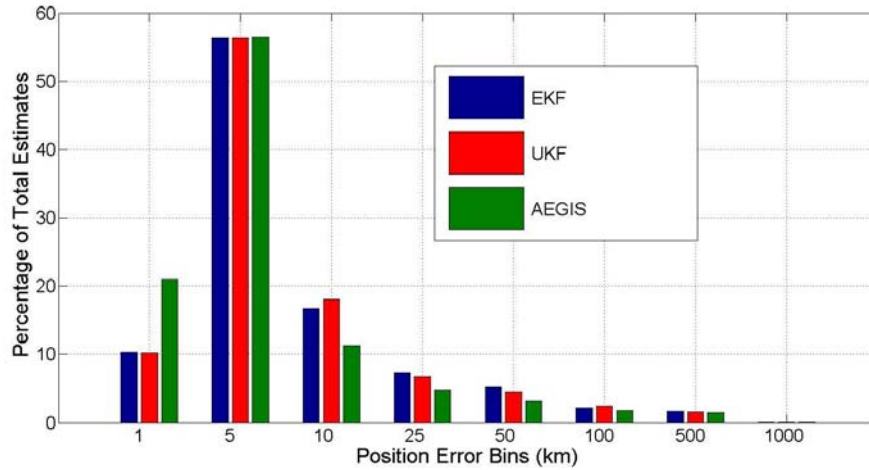
Figure 40. EKF, UKF, and AEGIS histograms of position estimate error distributions for the LLE simulation. Plots include data from all objects at all simulation time steps.
