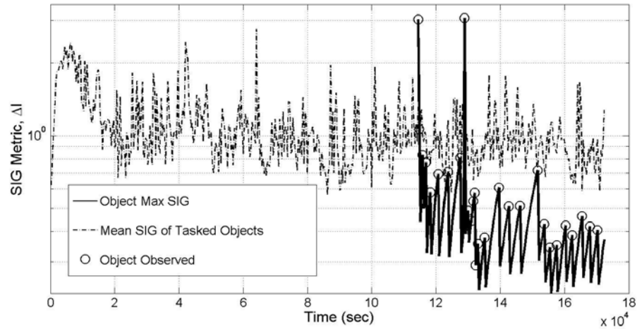
Figure 37. Plot of the SIG utility metric \Delta I and tasking decisions for object 21 using SIG tasking strategy in conjunction with a UKF. Thick sections of line reflect times when observations were available between that object and one or more sensors.
