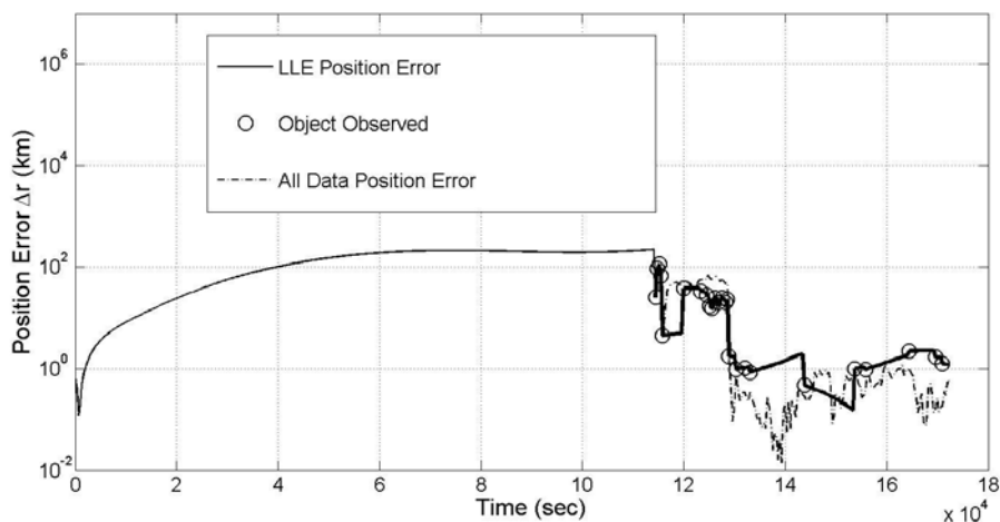
Figure 44. Plot of the position error \Delta r_{i,k} and tasking decisions for object 21 using the LLE tasking strategy in conjunction with an EKF. Thick sections of line reflect times when observations were available between object 21 and one or more sensors.
