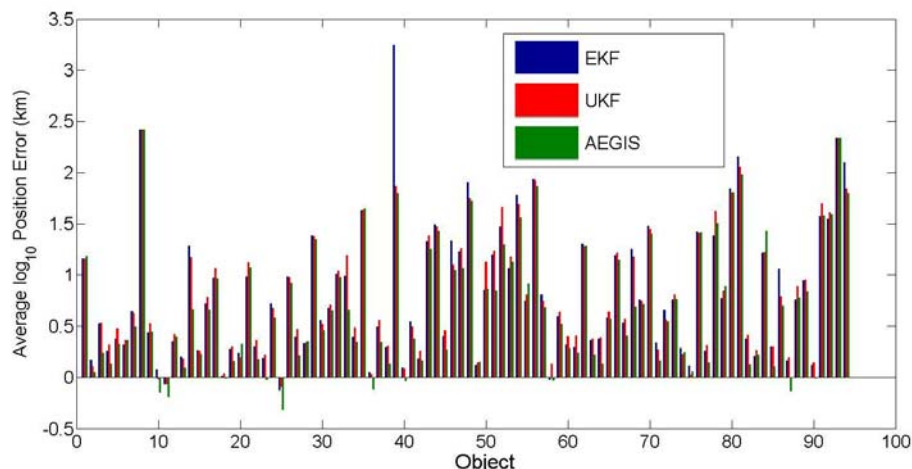
Figure 67. EKF, UKF, and AEGIS histograms of J_{i,k}^p metric in Equation 202 for SIG simulation. Plots include data from all objects at all simulation time steps.
