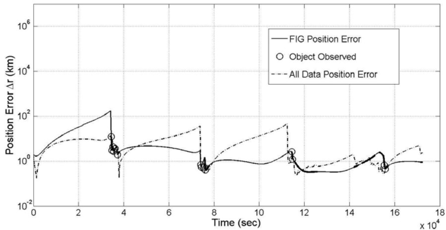
Figure 25. Plot of the position error \Delta r_{i,k} and tasking decisions for object 71 using FIG tasking strategy in conjunction with an AEGIS filter. Thick sections of line represent times when observations were available between object 71 and one or more sensors.
