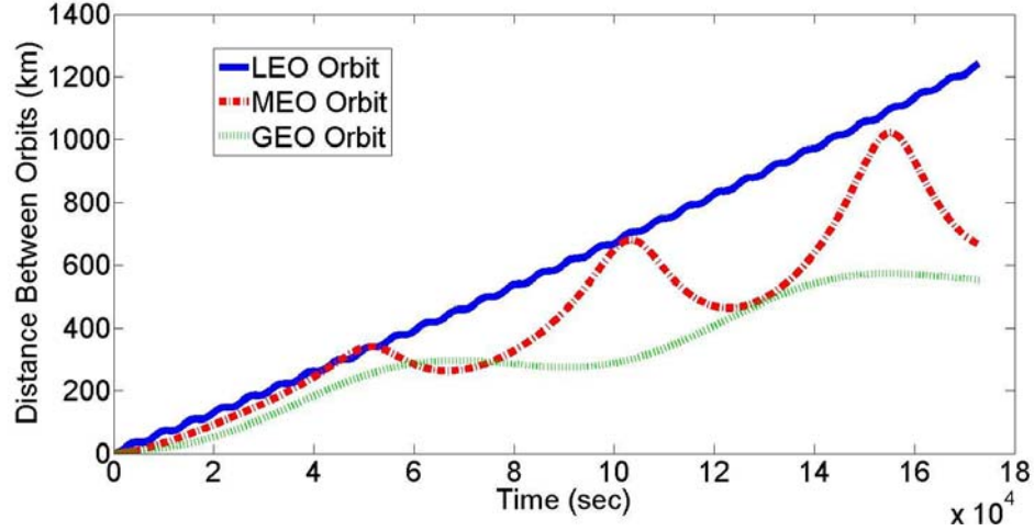
Figure 12. Plots of the propagation of displacement between two initially close LEO, MEO and GEO orbits.
