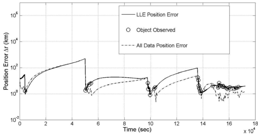
Figure 82. Plot of the position error \Delta r_{i,k} and tasking decisions for object 39 using LLE tasking strategy in conjunction with a UKF. Thick sections of line are times at which observations were available between object 39 and one or more sensors.
