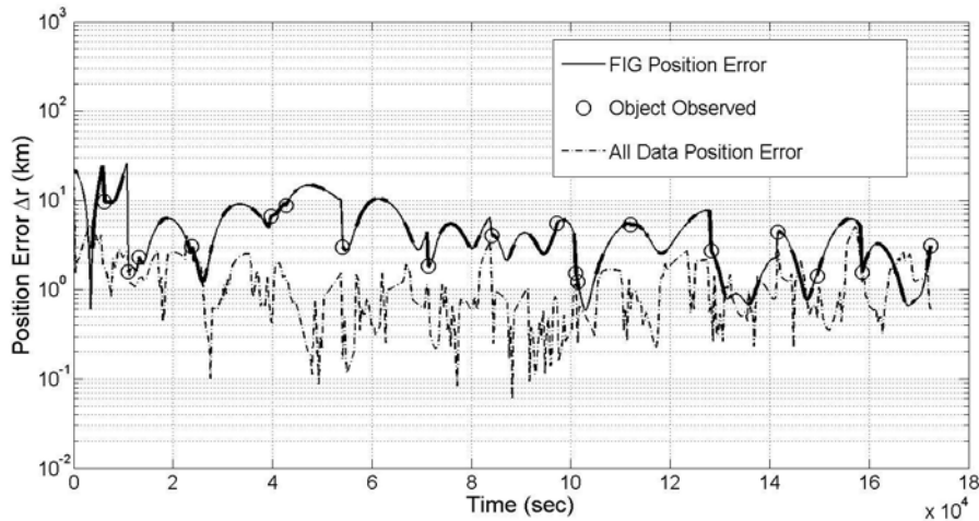
Figure 61. Plot of the position error \Delta r_{i,k} and tasking decisions for object 59 using FIG tasking strategy in conjunction with a UKF. Thick sections of line reflect times when observations were available between object 59 and one or more sensors.
