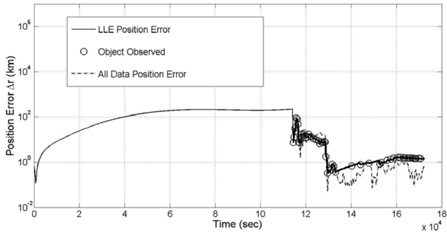
Figure 46. Plot of the position error \Delta r_{i,k} and tasking decisions for object 21 using the LLE tasking strategy in conjunction with an AEGIS filter. Thick sections of line reflect times when observations were available between object 21 and one or more sensors.
