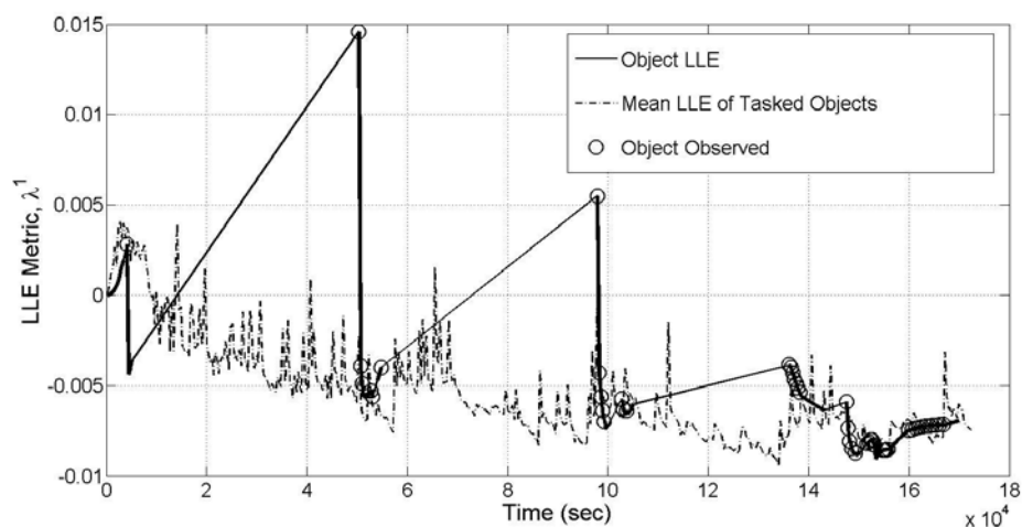
Figure 86. Plot of the LLE utility metric \hat{\lambda}^1 and tasking decisions for object 39 using LLE tasking strategy in conjunction with an AEGIS filter. Thick sections of line are times at which observations were available between that object and one or more sensors.
