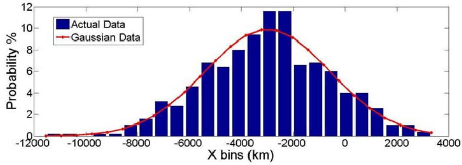
Figure 5. x-variable PDF of propagated distribution of space objects (binned into 25 equally spaced x-position locations) with corresponding Gaussian PDF overlay.
