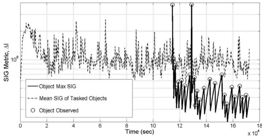
Figure 36. Plot of the SIG utility metric \Delta I and tasking decisions for object 21 using SIG tasking strategy in conjunction with an EKF. Thick sections of line reflect times when observations were available between that object and one or more sensors.
