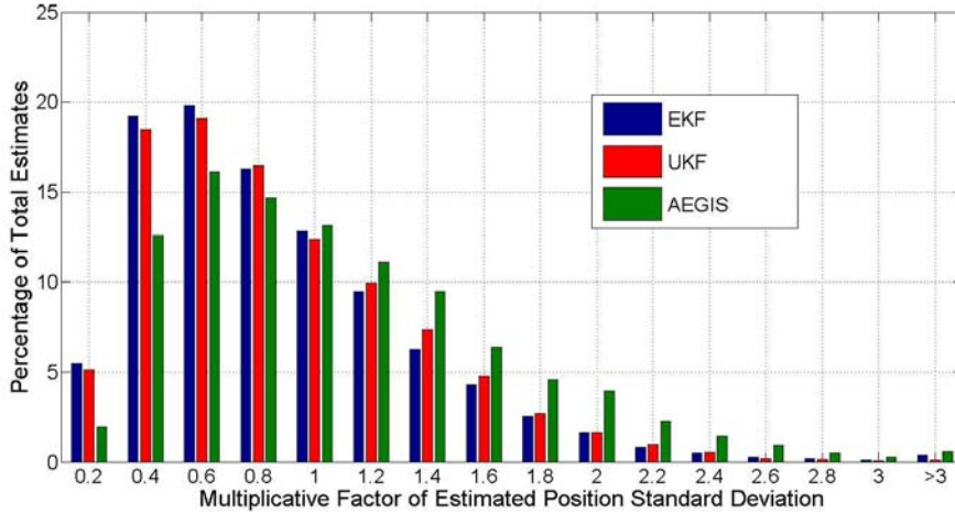
Figure 15. EKF, UKF, and AEGIS histograms of J_{i,k}^P metric in Equation 202 for all data simulation. Plots include data from all objects at all simulation time steps
