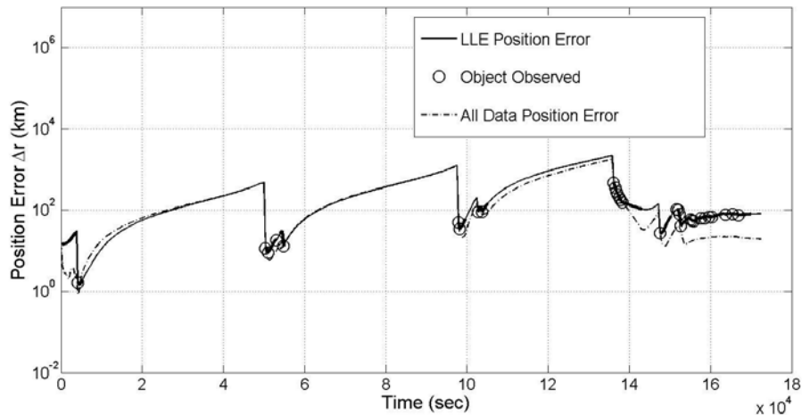
Figure 81. Plot of the position error \Delta r_{i,k} and tasking decisions for object 39 using LLE tasking strategy in conjunction with an EKF. Thick sections of line are times at which observations were available between object 39 and one or more sensors.
