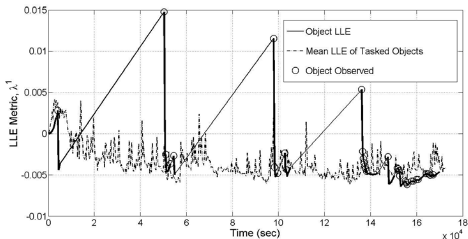
Figure 85. Plot of the LLE utility metric \hat{\lambda}^1 and tasking decisions for object 39 using LLE tasking strategy in conjunction with a UKF. Thick sections of line are times at which observations were available between that object and one or more sensors.
