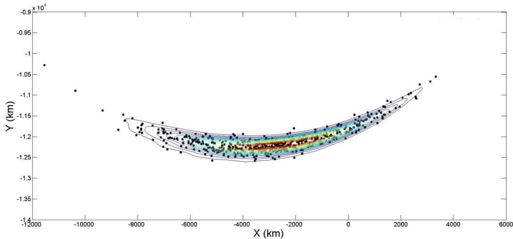
Figure 11. Propagation of initial Gaussian distribution with GMM PDF contour overlay calculated from propagating initial Gaussian PDF using AEGIS methods
