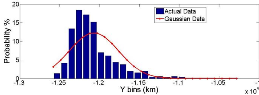
Figure 6. y-variable PDF of propagated distribution of space objects (binned into 25 equally spaced y-position locations) with corresponding Gaussian PDF overlay.
