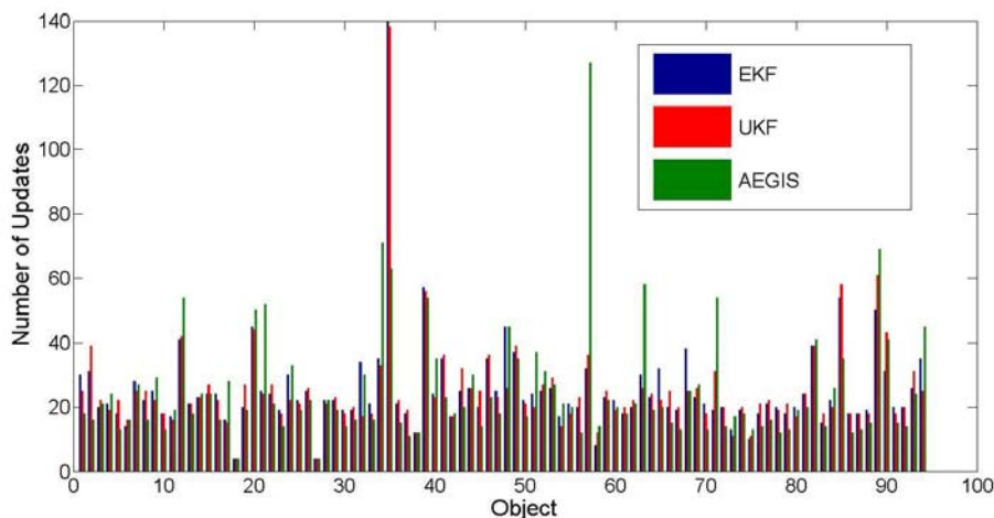
Figure 43. Bar graphs showing the updates each object received through implementation of an EKF, UKF, and AEGIS filter in conjunction with an LLE tasking strategy.
