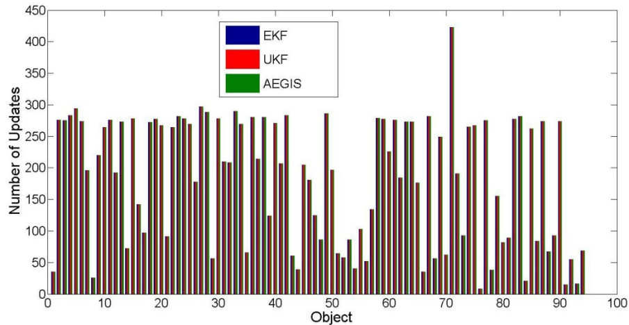
Figure 55. Bar graphs showing the updates each object received through implementation of an EKF, UKF, and AEGIS filter in conjunction with all data tasking strategy. In this case, the filters have equal amounts of updates, reflecting the maximum updates possible for all objects.
