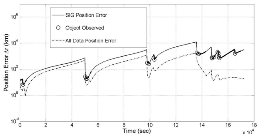
Figure 70. Plot of the position error \Delta r_{i,k} and tasking decisions for object 39 using SIG tasking strategy in conjunction with an EKF. Thick sections of line reflect times when observations were available between object 39 and one or more sensors.
