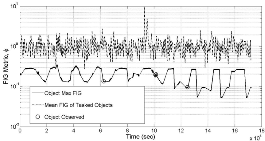
Figure 63. Plot of the FIG utility metric and tasking decisions for object 59 using FIG tasking strategy in conjunction with an EKF. Thick sections of line reflect times when observations were available between that object and one or more sensors.
