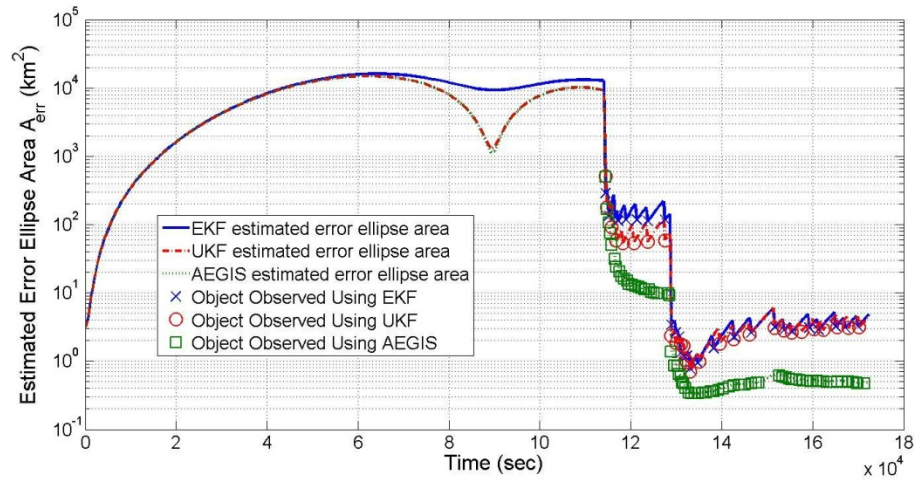
Figure 39. EKF, UKF, and AEGIS plots of \hat{A}_{err} = \pi\sqrt{\hat{\zeta}_{i,k}^1 \hat{\zeta}_{i,k}^2} metric for object 21 in the SIG simulation
