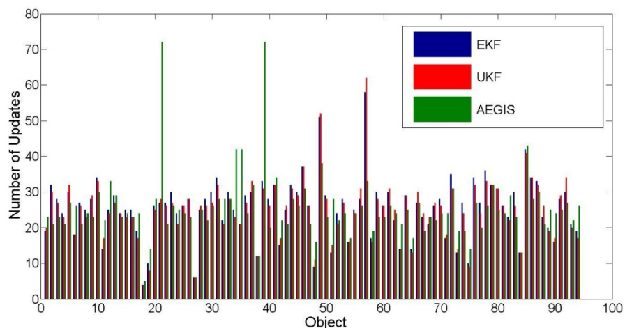
Figure 32. Bar graphs showing the updates each object received through implementation of an EKF, UKF, and AEGIS filter in conjunction with a SIG tasking strategy.
