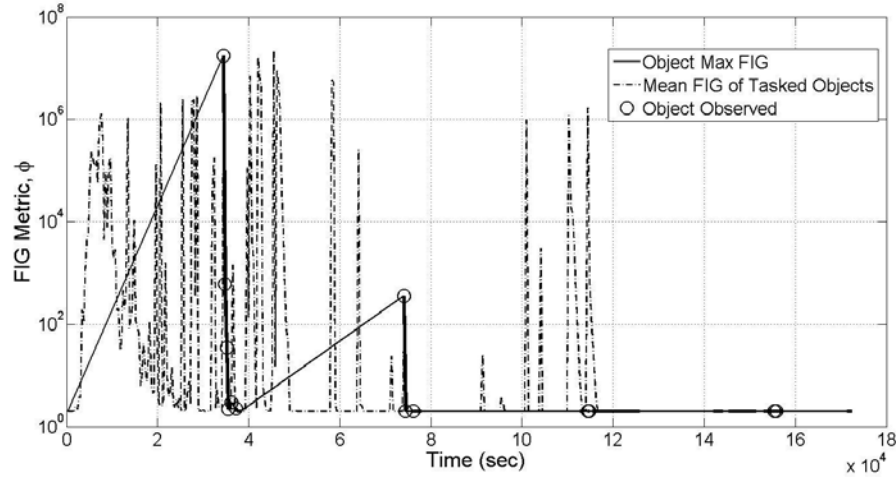
Figure 28. Plot of the FIG utility metric and tasking decisions for object 71 using FIG tasking strategy in conjunction with an AEGIS filter. Thick sections of line represent times when observations were available between that object and one or more sensors.
