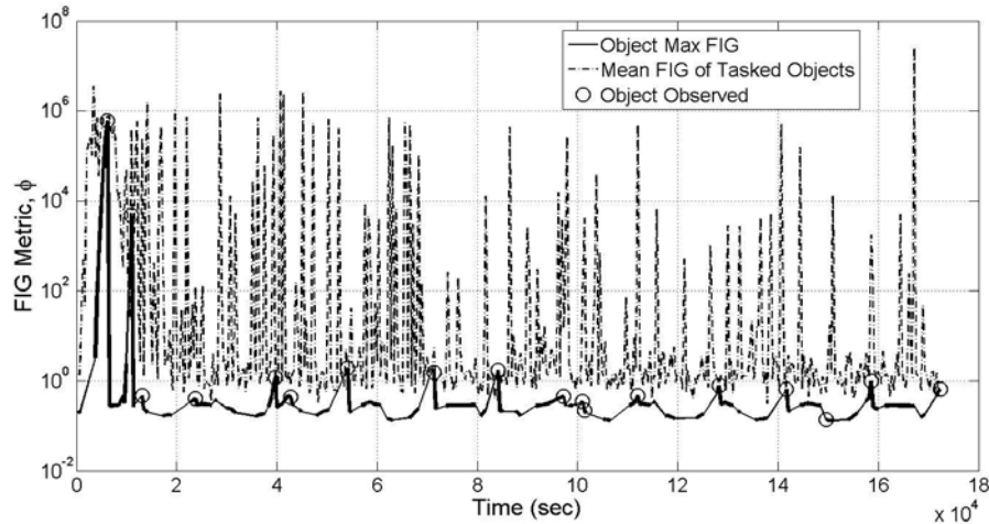
Figure 64. Plot of the FIG utility metric and tasking decisions for object 59 using FIG tasking strategy in conjunction with a UKF. Thick sections of line reflect times when observations were available between that object and one or more sensors.
