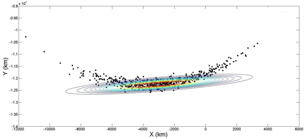
Figure 9. Propagation of initial Gaussian distribution showing contour overlay of the evaluation of Equation 19 with EKF forecast mean and covariance.
