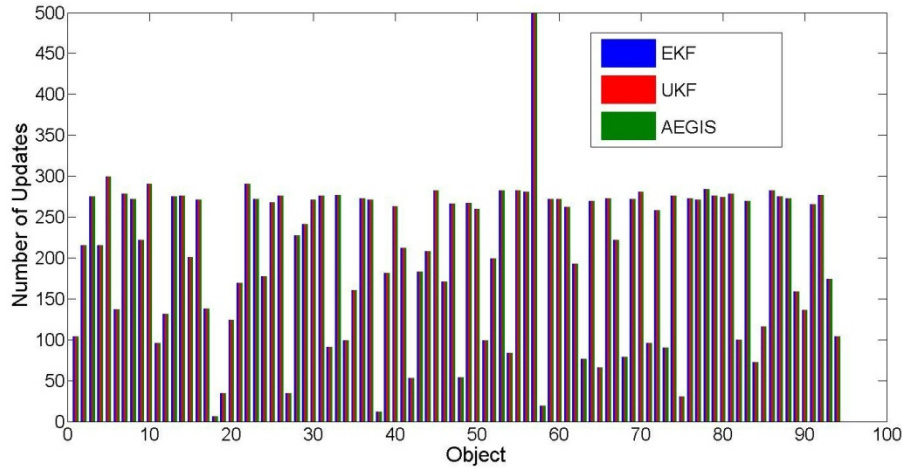
Figure 18. Bar graphs showing the updates each object received through implementation of an EKF, UKF, and AEGIS filter in conjunction with all data tasking strategy. In this case, all filters have equal amounts of updates for each object, reflecting the maximum updates possible for all objects.
