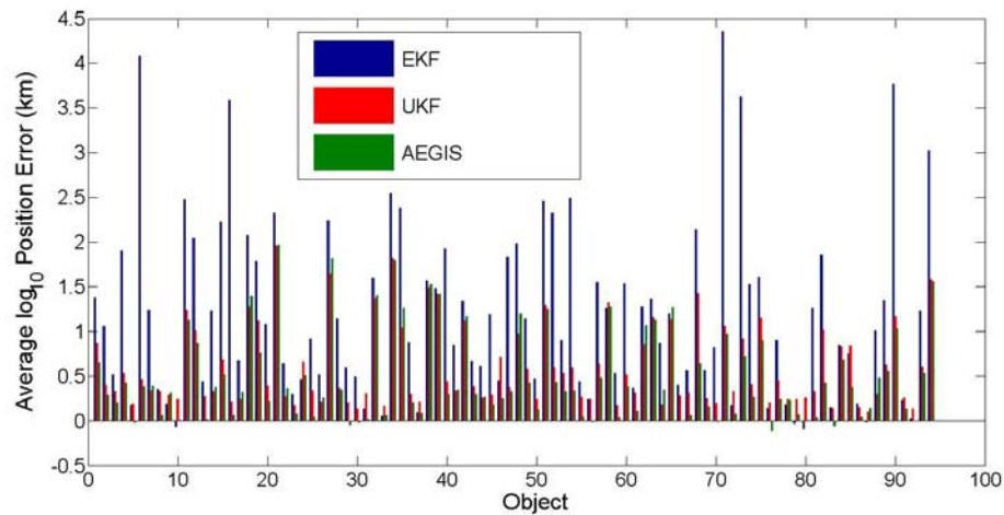
Figure 21. Bar graphs showing the \log_{10} average position error for each object given in Equation 200, through implementation of an EKF, UKF and AEGIS filter in conjunction with an FIG tasking strategy.
