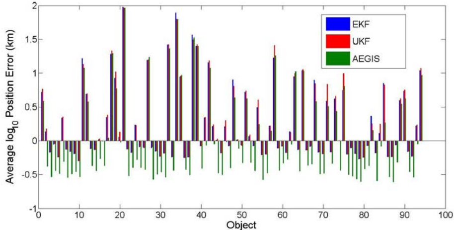
Figure 17. Bar graphs showing the \log_{10} average position error for each object given in Equation 200, through implementation of an EKF, UKF, and AEGIS filter in conjunction with all data tasking strategy. In this case, all filters have equal amounts of updates for each object, reflecting the maximum updates possible for all objects.
