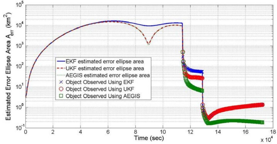
Figure 16. EKF, UKF, and AEGIS plots of \hat{A}_r^* = \pi \sqrt{\zeta_{i,k}^1 \zeta_{i,k}^2} metric for the object with the highest average position error in the all data simulation.
