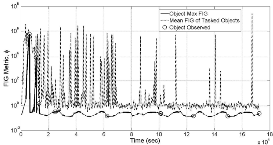
Figure 65. Plot of the FIG utility metric and tasking decisions for object 59 using FIG tasking strategy in conjunction with an AEGIS filter. Thick sections of line reflect times when observations were available between that object and one or more sensors.
