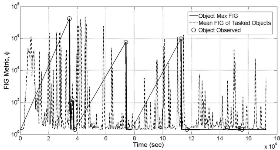
Figure 27. Plot of the FIG utility metric and tasking decisions for object 71 using FIG tasking strategy in conjunction with a UKF. Thick sections of line represent times when observations were available between that object and one or more sensors.
