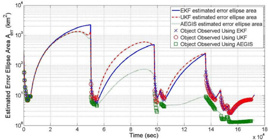
Figure 53. EKF, UKF, and AEGIS plots of \hat{A}_{err} = \pi\sqrt{\zeta_{i,k}^1\zeta_{i,k}^2} metric for the object with the highest average position error in the all data simulation.
