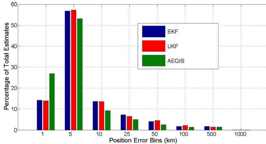
Figure 29. EKF, UKF, and AEGIS histograms of position estimate error distributions for SIG simulation. Plots include data from all objects at all simulation time steps.
