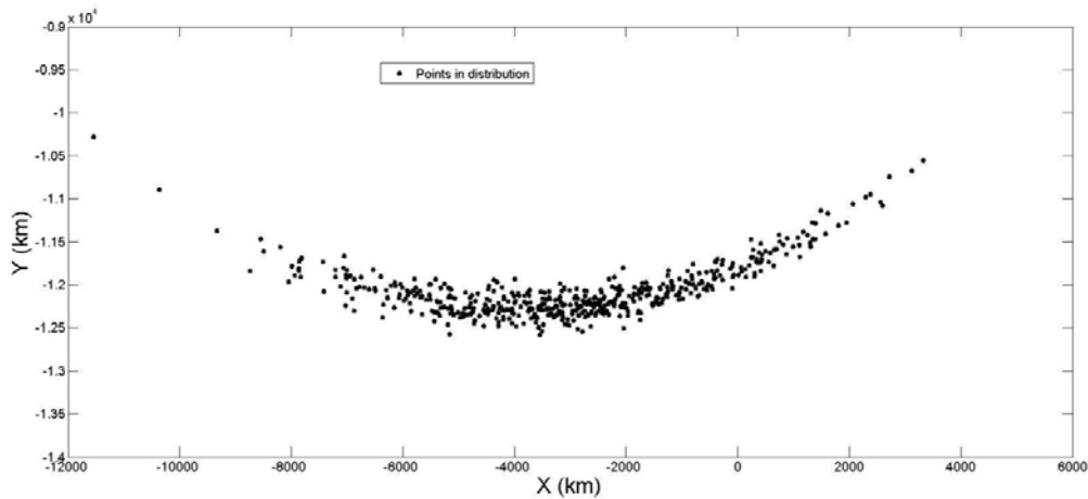
Figure 4. Illustration of Initial Gaussian Uncertainty Distribution Propagated Through Nonlinear Orbit Dynamics
