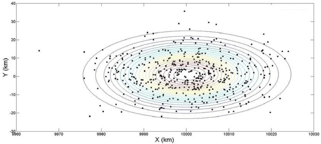
Figure 3. Illustration of Initial Gaussian Uncertainty Distribution of Space Object and Contour Overlay of PDF Evaluation Using Equation 19
