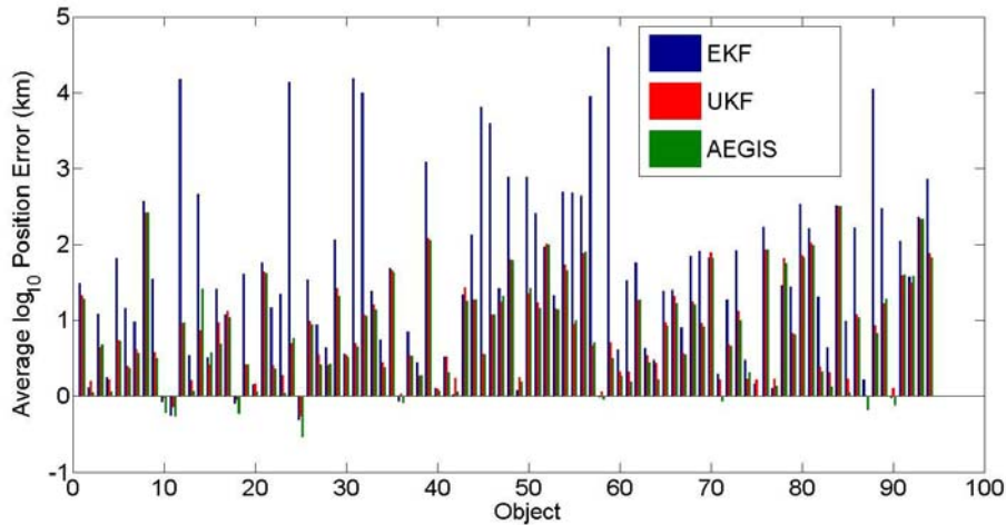
Figure 58. Bar graphs showing the \log_{10} average position error for each object given in Equation 200, through implementation of an EKF, UKF and AEGIS filter in conjunction with a FIG tasking strategy.
