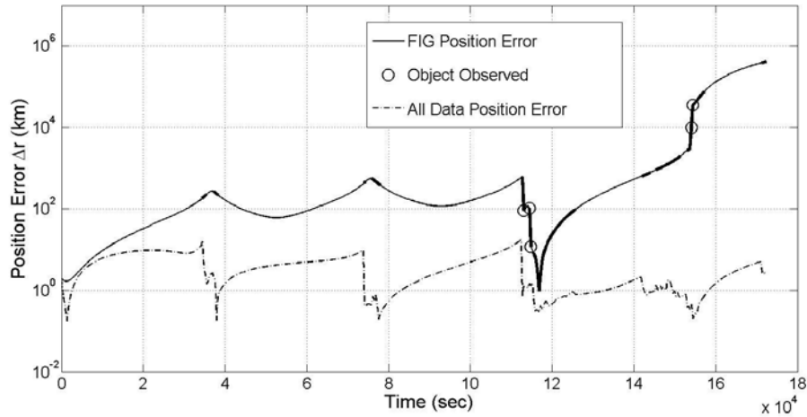
Figure 23. Plot of the position error \Delta r_{i,k} and tasking decisions for object 71 using FIG tasking strategy in conjunction with an EKF. Thick sections of line represent times when observations were available between object 71 and one or more sensors.
