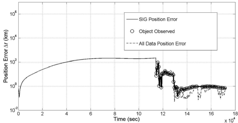
Figure 35. Plot of the position error \Delta r_{i,k} and tasking decisions for object 21 using SIG tasking strategy in conjunction with an AEGIS Filter. Thick sections of line reflect times when observations were available between object 21 and one or more sensors.
