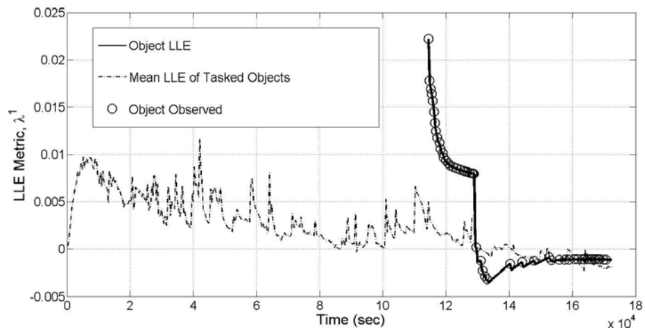
Figure 49. Plot of the LLE utility metric \hat{\lambda}^1 and tasking decisions for object 21 using the LLE tasking strategy in conjunction with an AEGIS filter. Thick sections of line reflect times when observations were available between that object and one or more sensors.
