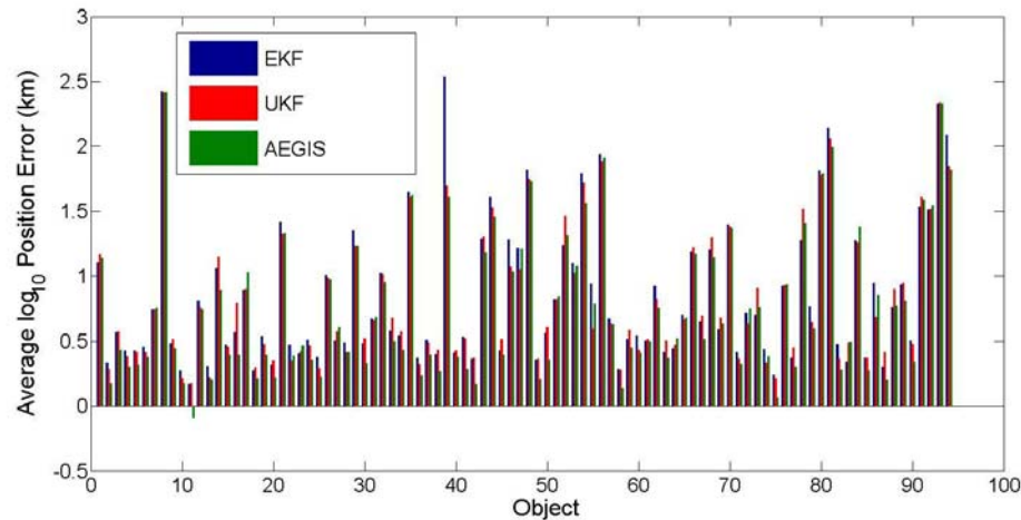
Figure 79. Bar graphs showing the \log_{10} average position error for each object given in Equation 200, through implementation of an EKF, UKF and AEGIS filter in conjunction with an LLE tasking strategy.
