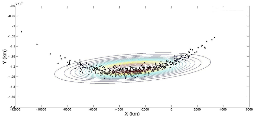
Figure 10. Propagation of initial Gaussian distribution showing contour overlay of the evaluation of Equation 19 with UKF forecast mean and covariance.
