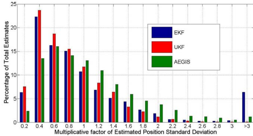
Figure 20. EKF, UKF, and AEGIS histograms of J_{i,k}^{\hat{p}} metric in Equation 202 for FIG simulation. Plots include data from all objects at all simulation time steps.
