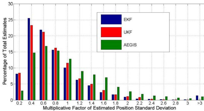
Figure 41. EKF, UKF, and AEGIS histograms of J_{i,k}^p metric in Equation 202 for the LLE simulation. Plots include data from all objects at all simulation time steps
