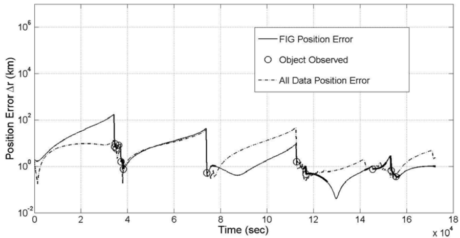
Figure 24. Plot of the position error \Delta r_{i,k} and tasking decisions for object 71 using FIG tasking strategy in conjunction with a UKF. Thick sections of line represent times when observations were available between object 71 and one or more sensors.
