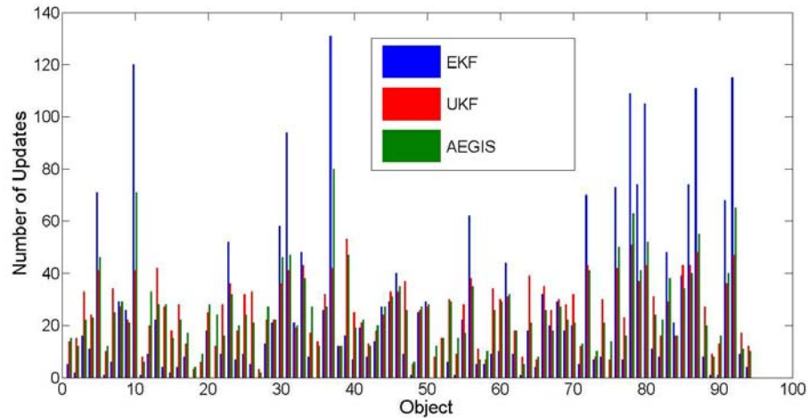
Figure 22. Bar graphs showing the updates each object received through implementation of an EKF, UKF, and AEGIS filter in conjunction with an FIG tasking strategy. The FIG tasking results in many updates to a select few objects, while many other objects receive little to none.
