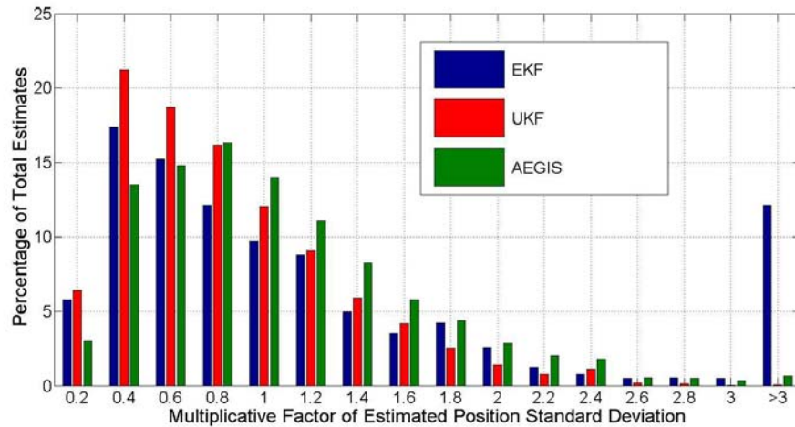
Figure 57. EKF, UKF, and AEGIS histograms of J_{i,k}^{\hat{p}} metric in Equation 202 for FIG simulation. Plots include data from all objects at all simulation time steps
