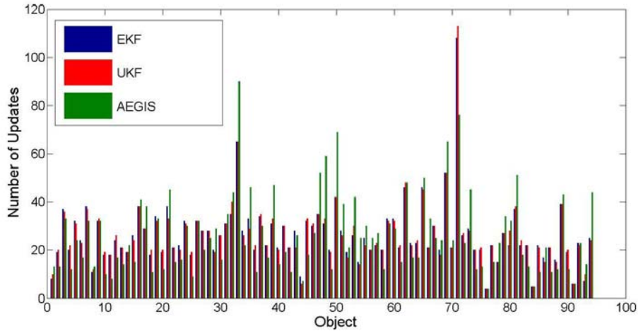
Figure 80. Bar graphs showing the updates each object received through implementation of an EKF, UKF, and AEGIS filter in conjunction with an LLE tasking strategy.
