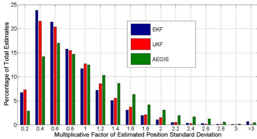
Figure 30. EKF, UKF, and AEGIS histograms of J_{i,k}^p metric in Equation 202 for SIG simulation. Plots include data from all objects at all simulation time steps
