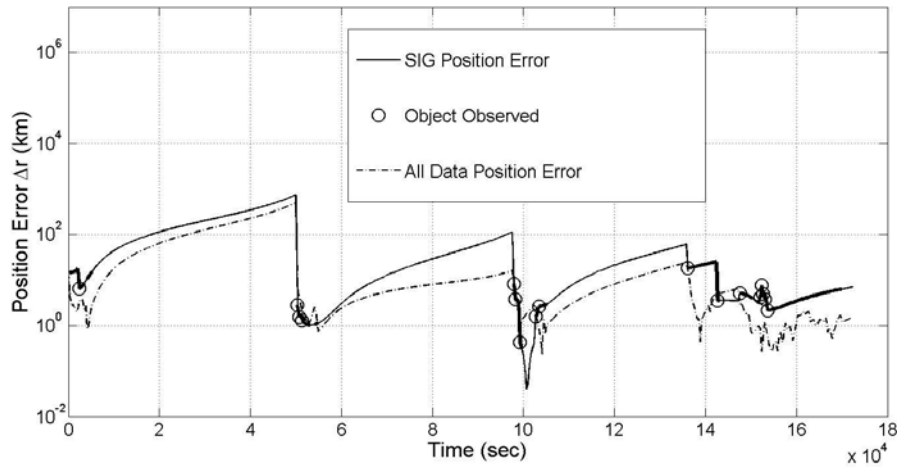
Figure 71. Plot of the position error \Delta r_{i,k} and tasking decisions for object 39 using SIG tasking strategy in conjunction with a UKF. Thick sections of line reflect times when observations were available between object 39 and one or more sensors.
