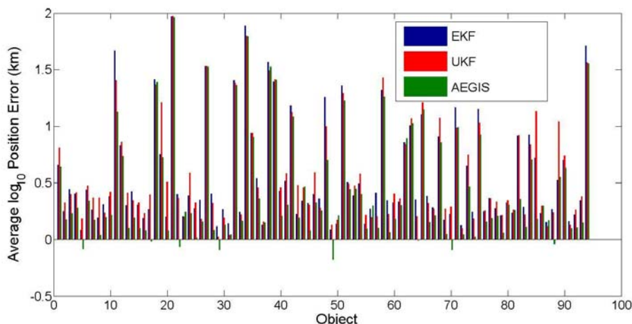
Figure 42. Bar graphs showing the \log_{10} average position error for each object given in Equation 200, through implementation of an EKF, UKF and AEGIS filter in conjunction with an LLE tasking strategy.
