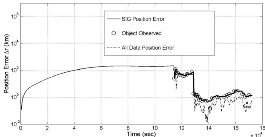
Figure 33. Plot of the position error \Delta r_{i,k} and tasking decisions for object 21 using SIG tasking strategy in conjunction with an EKF. Thick sections of line reflect times when observations were available between object 21 and one or more sensors.
