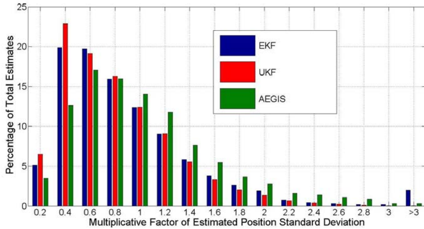
Figure 78. EKF, UKF, and AEGIS histograms of J_{i,k}^p metric in Equation 202 for LLE simulation. Plots include data from all objects at all simulation time steps.
