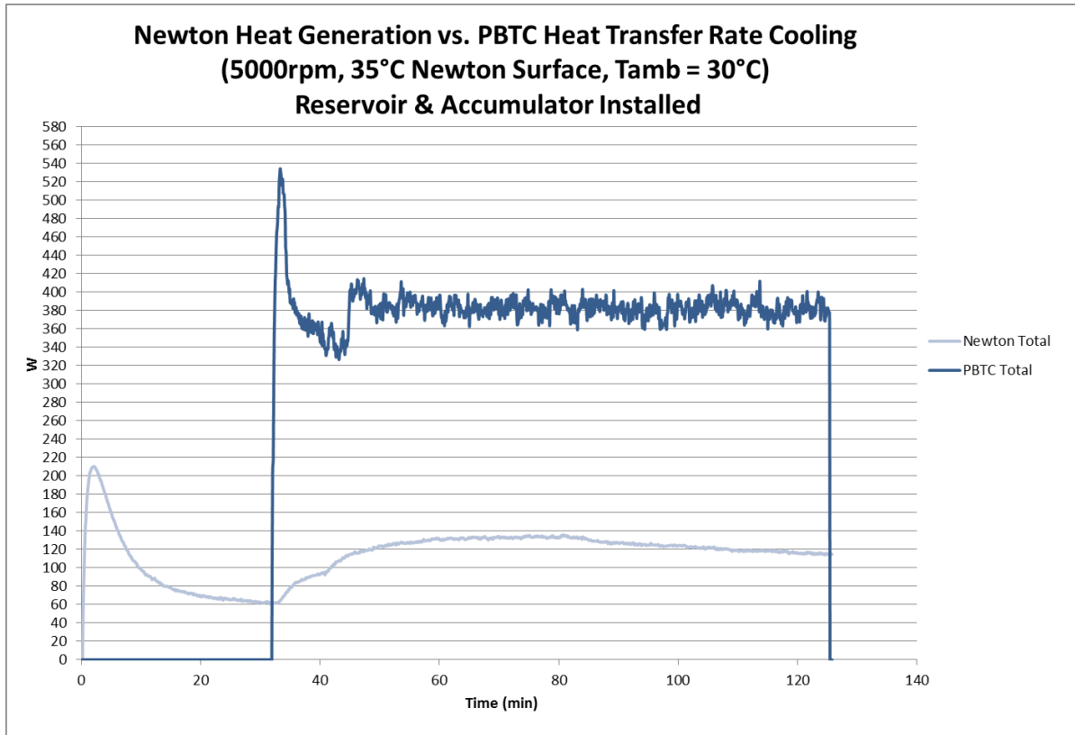
Figure 21. PBTC cooling capacity evaluation with reservoir & accumulator
