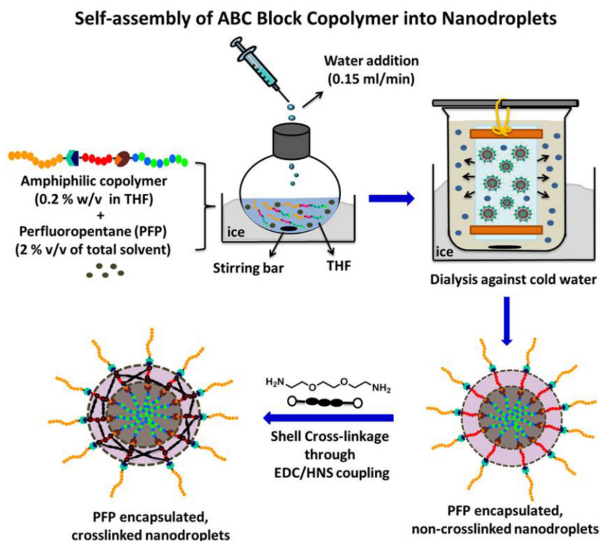
Fig 1. Formulation of PFP-loaded nanodroplets by self-assembly of amphiphilic triblock PEG 45 - b -PAA 10 - b -P(HDFMA 8 - co -MMA 21 ) copolymer around the PFP core followed by shell cross-linkage via EDC/HNS coupling reactions.
