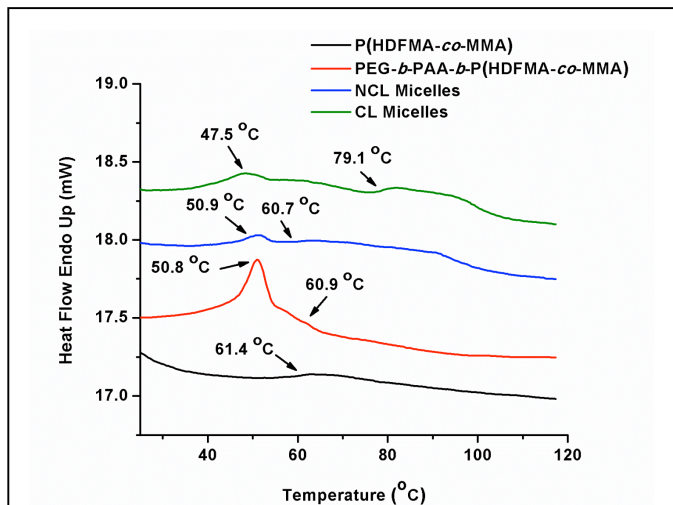
Figure 5. Thermal properties of P(HDFMA- co -MMA), PEG- b -PAA- b -P(HDFMA- co -MMA) (ABC-1), non-crosslinked micelles and crosslinked micelles made out of ABC-1 block copolymer.
