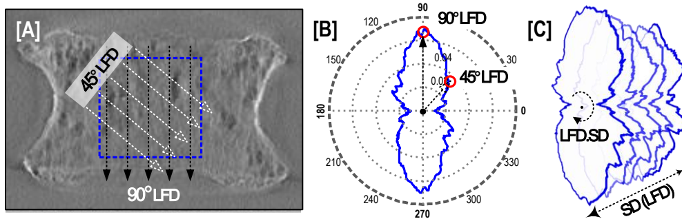
Figure 3 - [A] A square region cropped out of the DTS image is analyzed using the fractal, MIL and LFD analysis methods. MIL and LFD are calculated in all directions in the image. [B] A typical polar plot representation of the LFD data, from which an average, standard deviation, max and anisotropy (LFD at
