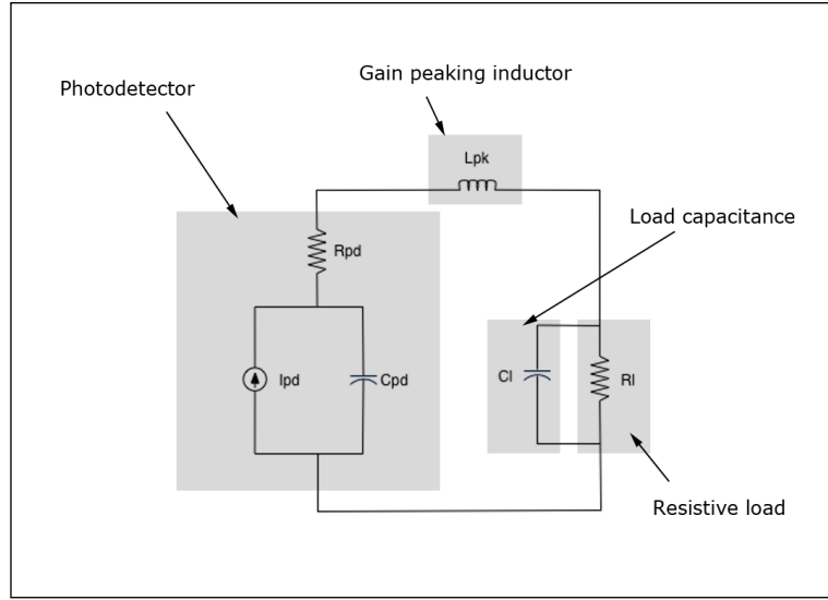
Fig. 5. Small-signal AC circuit for an enhanced series gain peaked photodetector circuit. The additional capacitor C_l is in parallel with the load resistance. This could be a load capacitance due to bump-bonding or another form of packaging, or it could be an intentionally added capacitance via a MIM capacitor layer.
