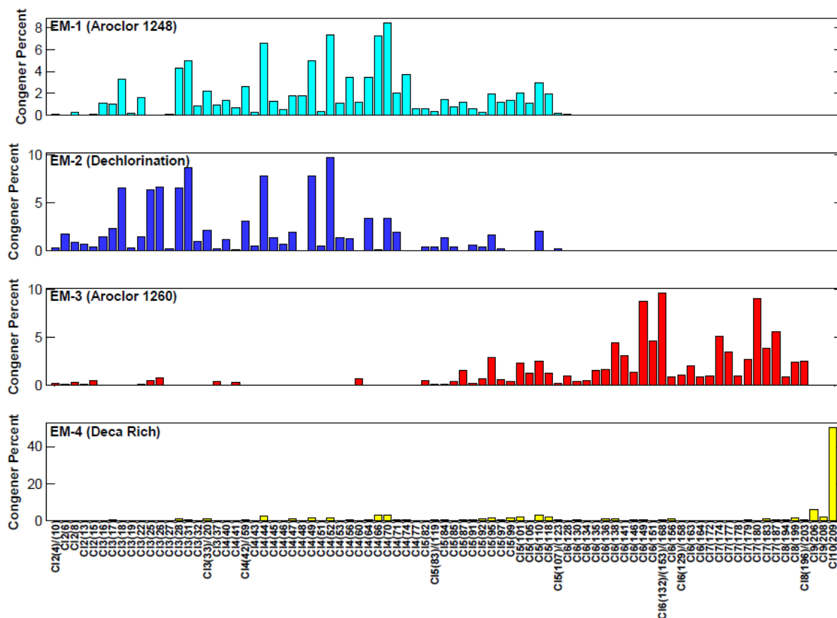
Figure 19. Ashtabula End-member (EM) compositions.
