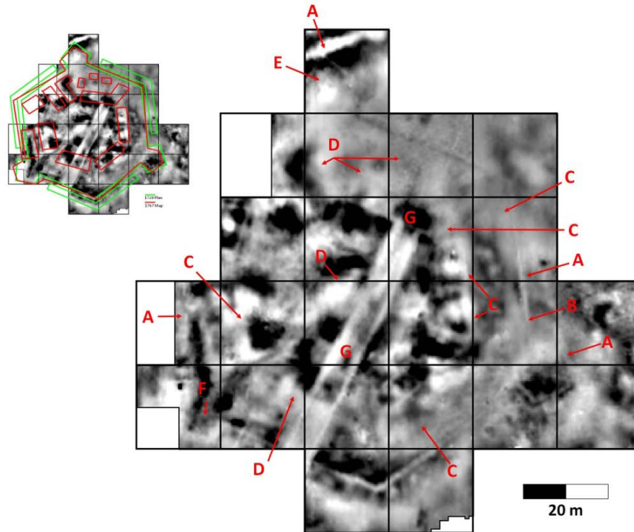
Figure 10. Preliminary interpretation of electrical resistance data prior to excavations. Anomalies labeled in red are discussed in Table 3.
