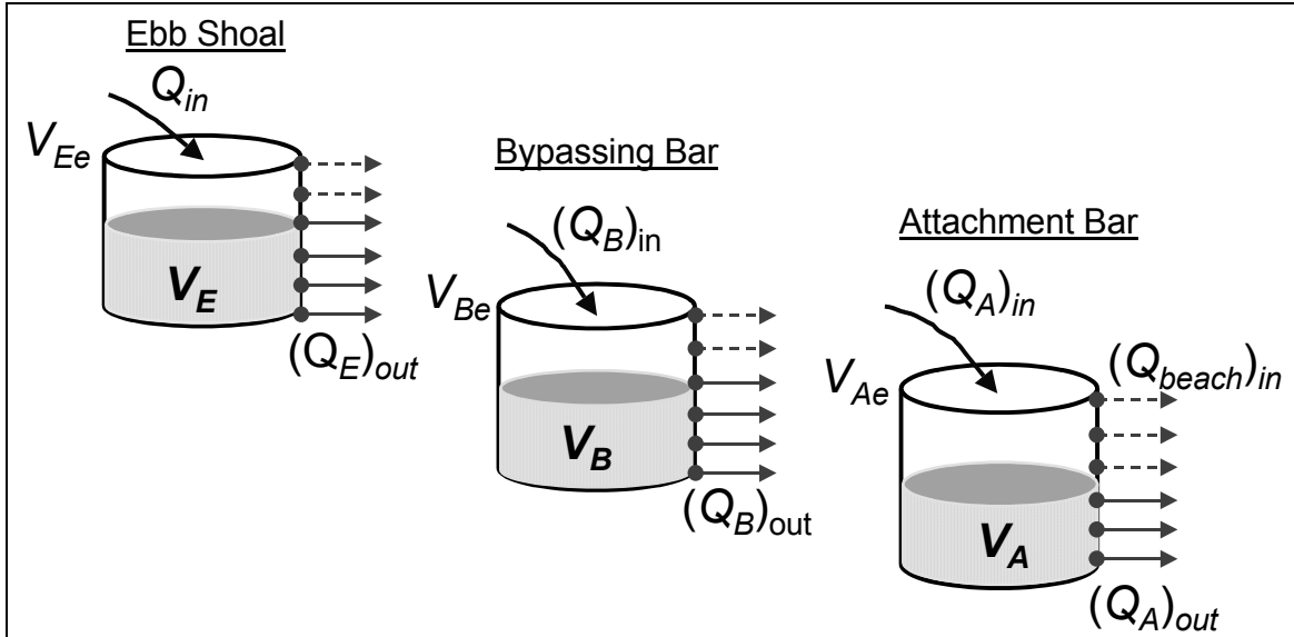
FIG. 3. Definition Sketch for Reservoir Inlet Morphology Aggregate Model
