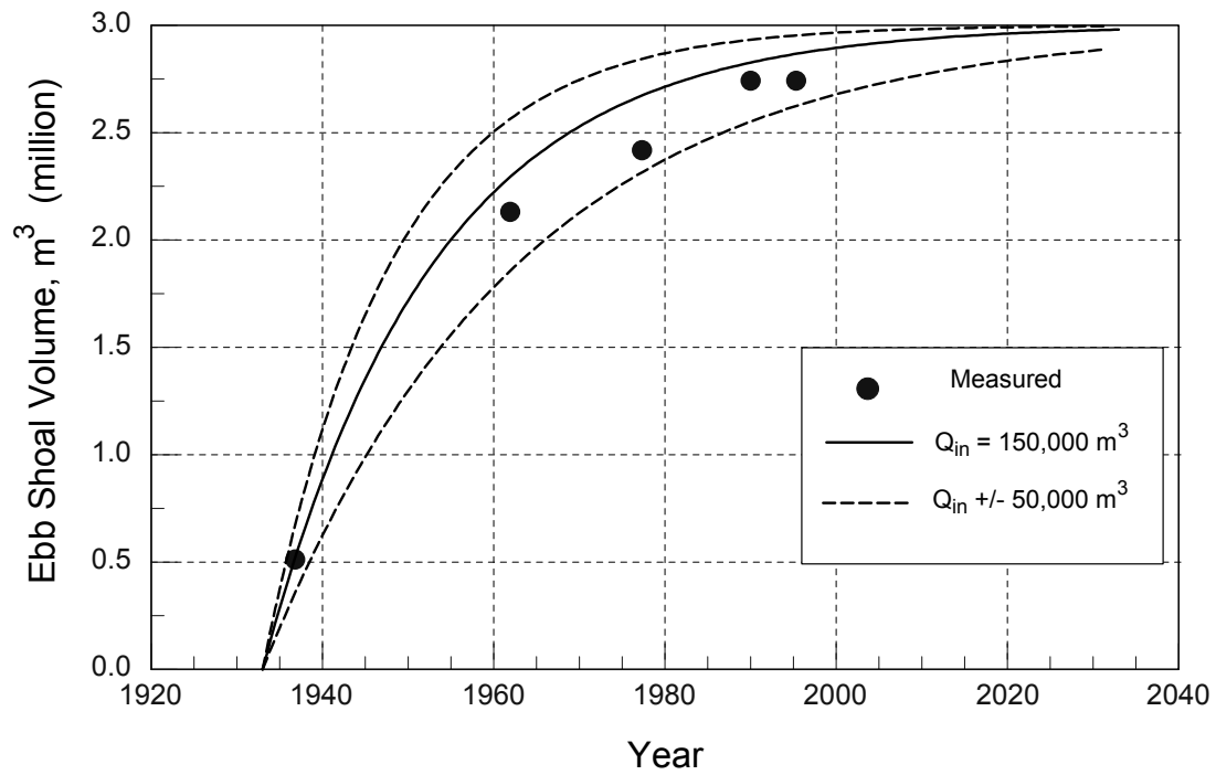
FIG. 5. Volume of Ebb-Shoal, Ocean City Inlet
