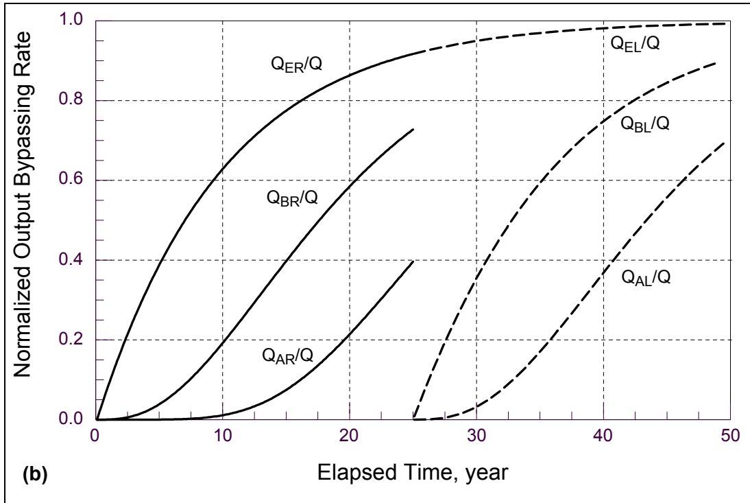
FIG. 10. Bypassing Rates for Simple Bi-directional Transport
