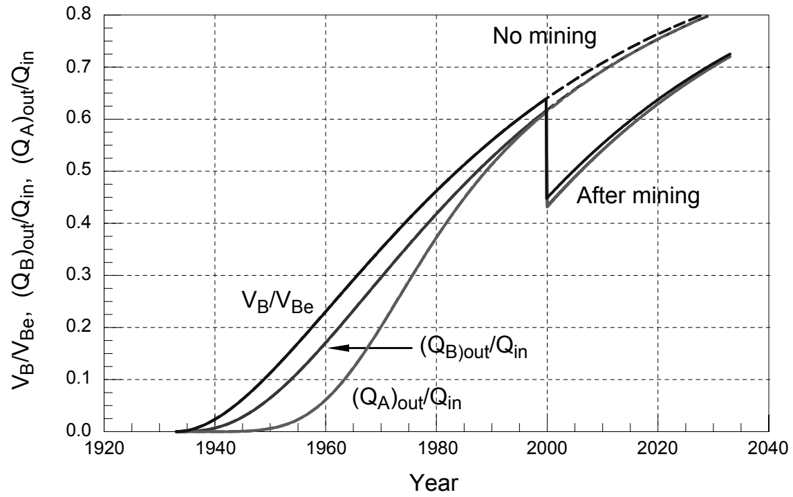
FIG. 9. Bypassing Bar Volume and Bypassing Rates With/Without Mining
