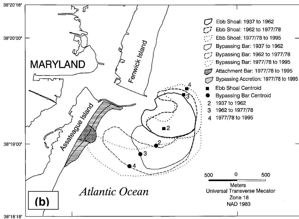
FIG. 4. Ebb-Shoal Plan Form Determined from Interpretation of 7-m Contour, Ocean City Inlet
