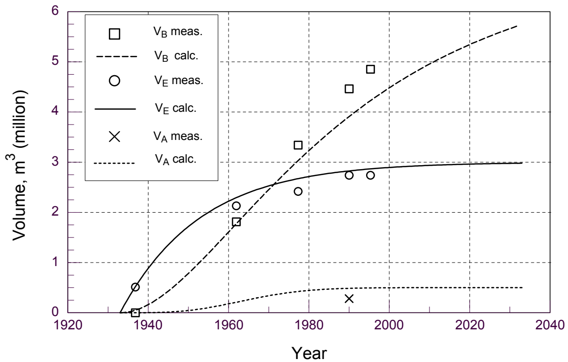
FIG. 6. Volumes of Ebb Shoal, Bypassing Bar, and Attachment Bar, Ocean City Inlet
