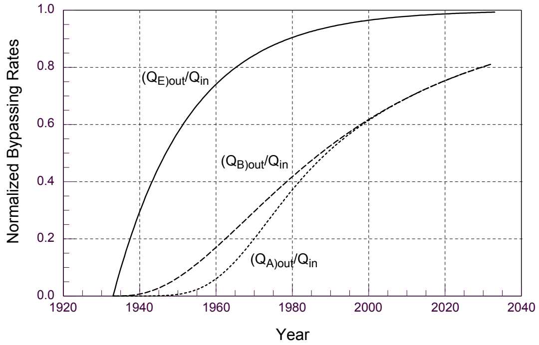
FIG. 7. Calculated Bypassing Rates, Ocean City Inlet
