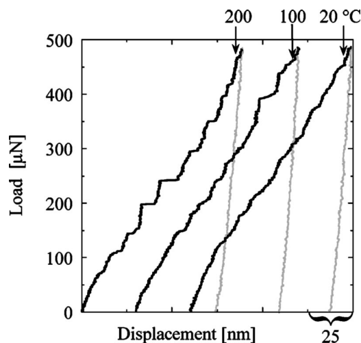
FIG. 1. Typical load-displacement curves measured at 20, 100, and 200 °C, with their origins offset for clarity of presentation. The loading portion of each curve is shown in black, and the unloading portion in grey. As temperature is raised, there is a pronounced increase in the prominence of the horizontal “pop-ins” in the loading part of the experiments.
