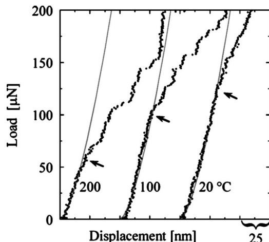
FIG. 2. Initial nanoindentation response of (100) Pt at three different temperatures. In each case, the first portion of the experimental data (black points) can be well described by the Hertzian elastic contact law (grey lines), but the departure from ideal elasticity occurs earlier for specimens at higher temperatures.
