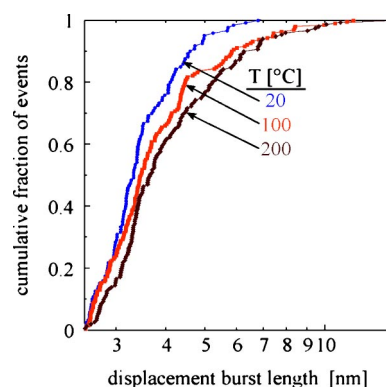
FIG. 3. (Color online). Cumulative fraction of pop-in events of a given size, incorporating data from many indentations under the same conditions; the x axis is logarithmic to better observe trends. The tendency for displacement bursts of every size increases monotonically with temperature.
