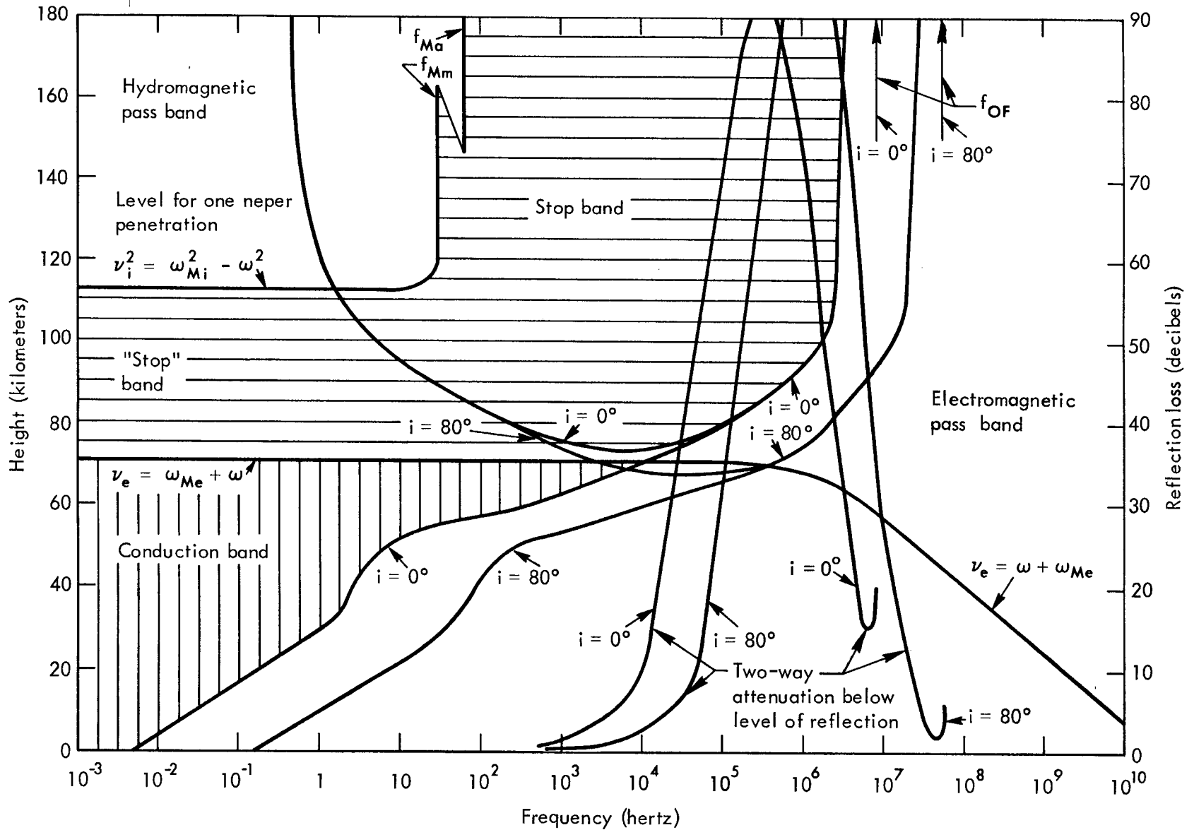
Fig. 7—Quasi-longitudinal propagation of the 0 wave for ambient (undisturbed) day conditions
