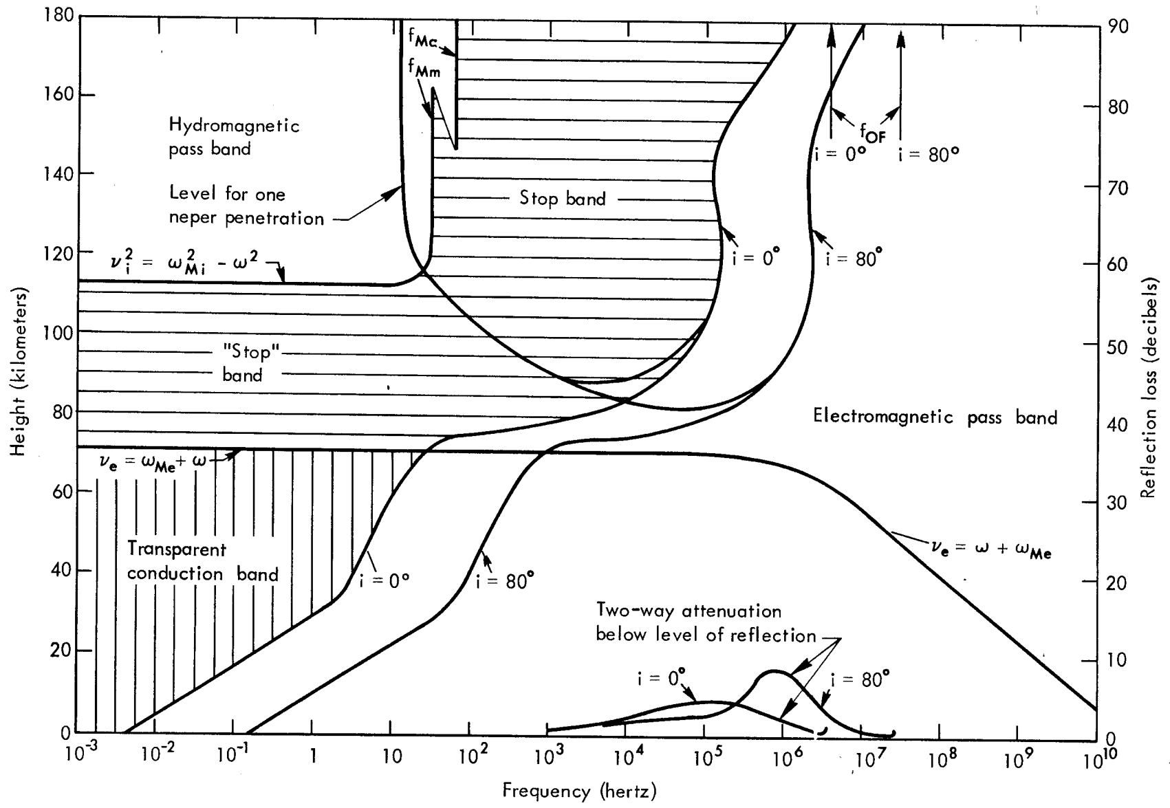
Fig. 3—Quasi-longitudinal propagation of the 0 wave for ambient (undisturbed) night conditions
