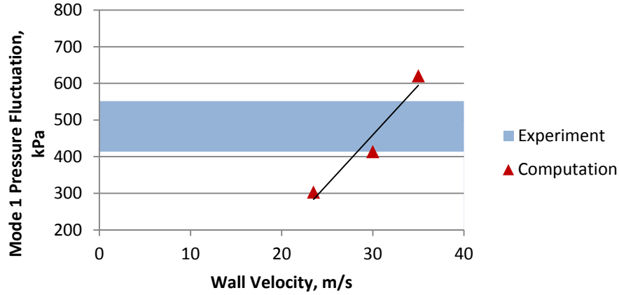
Figure 3: Effect of wall velocity on pressure.
