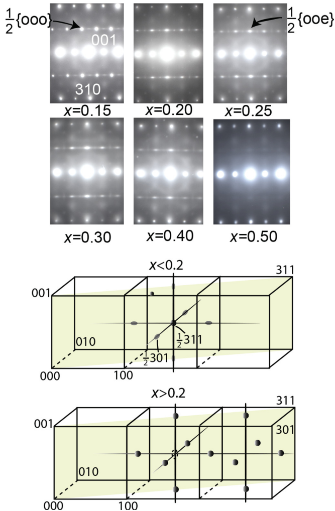
FIG. 2. (Color online) Representative \langle 310 \rangle selected area electron diffraction patterns for a series of (1-x)\text{NBT}-x\text{KBT} compositions. The superlattice reflections change from 1/2\{ooo\} for x < 0.2 to 1/2\{ooe\} for x > 0.2 . For x = 0.2 , both types of reflections are present though the dominant type varies from grain to grain. For x < 0.2 , the diffuse spots at 1/2\{ooe\} , which are streaked along \langle 100 \rangle directions, signify short-range ordered in-phase tilting. In contrast, for x \geq 0.2 , the round-shaped diffuse spots at 1/2\{ooo\} arise from intersections of several \langle 100 \rangle diffuse rods associated with 1/2\{ooe\} reflections, as discussed in the text. The reciprocal lattices for both cases are illustrated in the figure.
