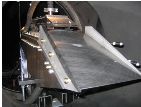
Figure 46: HyShot wind tunnel model installed in the HEG test section
