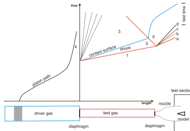
Figure 2: Schematic and wave (x-t) diagram of a free piston driven shock tunnel
