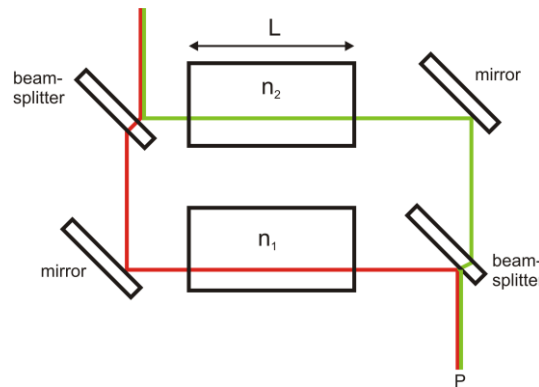
Figure 20: Schematic of interference experiment
