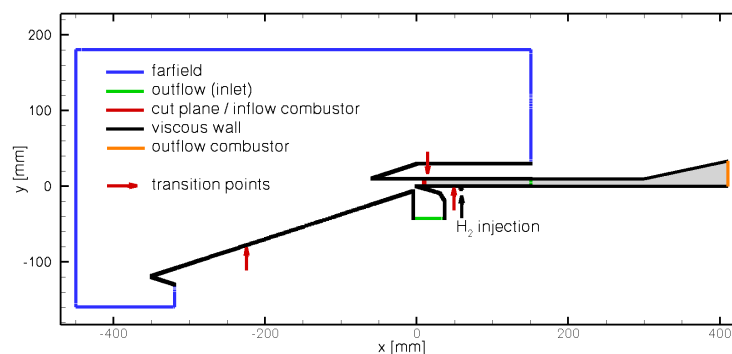
Figure 48: Computational domains and boundary conditions used for the intake and combustor / nozzle investigations
