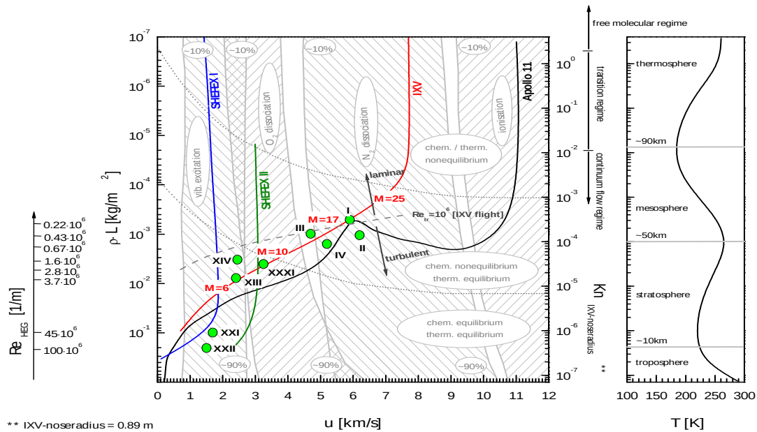
Figure 6: HEG operating conditions in terms of the binary scaling parameter pL and the flow velocity u
