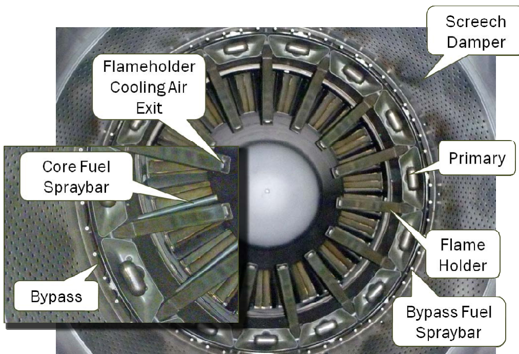
Figure 31: EJ200 Afterburner.
