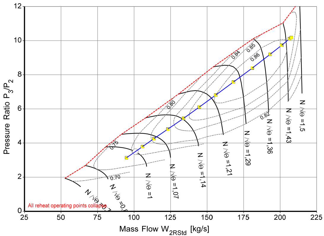
Figure 15: Compressor Design 1: \Pi_{bs} = 10 .
