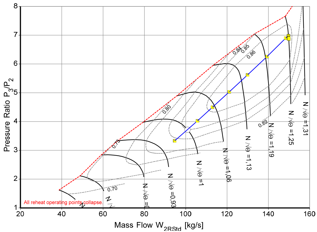
Figure 16: Compressor Design 2: \Pi_{bs} = 7 .
