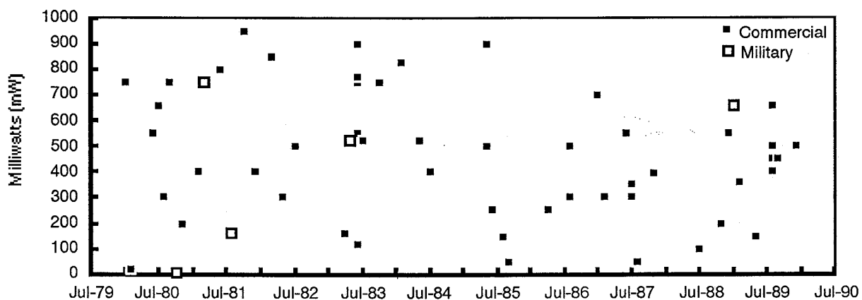
Figure 89 presents a comparison of power dissipation in commercial and military ROMs. There is a limited number of military data points, but the data points that are available appear to be evenly distributed, with military ROMs appearing at both the low and the high ends of the power dissipation range.
