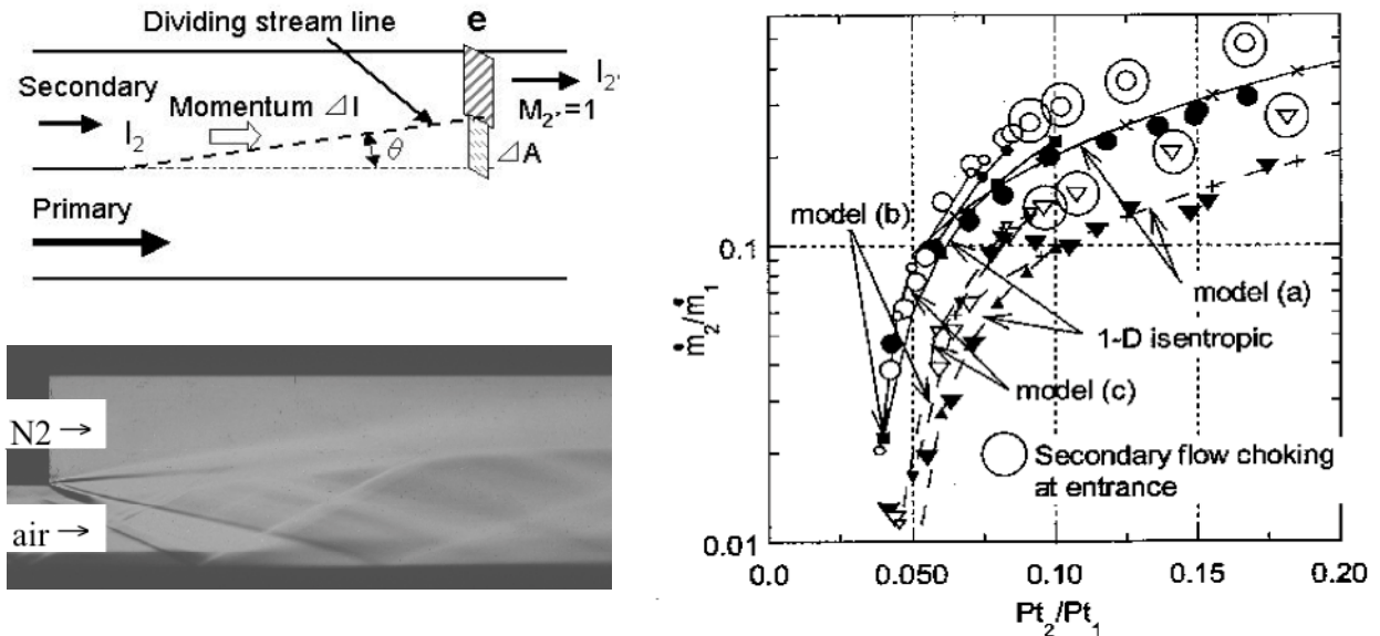
Figure 5: Ejector modelling (upper left), cold flow example (lower left) and ejector prediction profiles.
