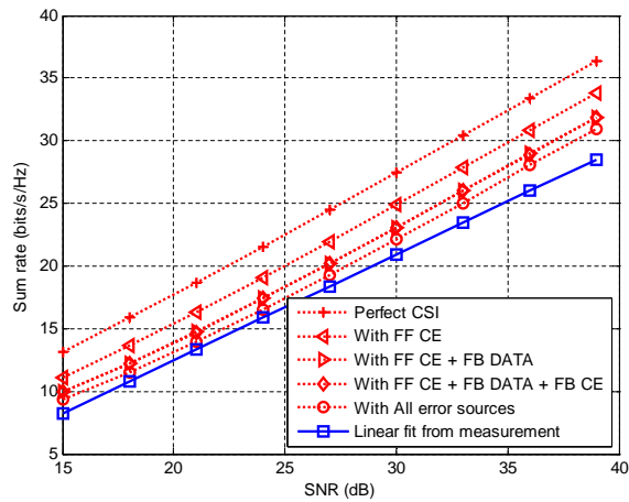
(b) Comparison of measured sum rate to simulated sum rate.
