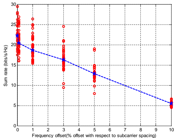
Figure 19: IA performance with the residual frequency synchronization error
