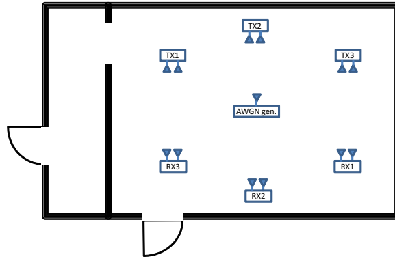
Figure 16: Test environment of distributed nodes.
