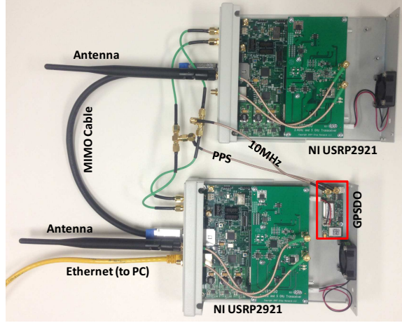
Figure 15: Hardware configuration of one node.
