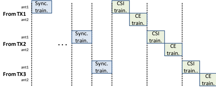
(a) Feedforward packet structure for training phase.
