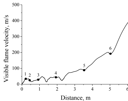
Figure 8: Predicted flame propagation velocity in the 6.1-meter tube. Black dots denote locations with different flame shapes, shown in Fig. 5.
