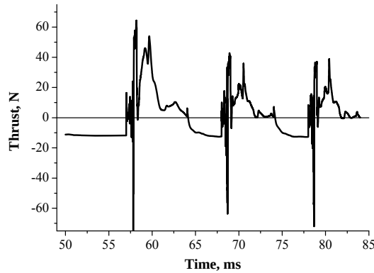
Figure 23: Predicted time history of PDE thrust in the course of three engine cycles.
