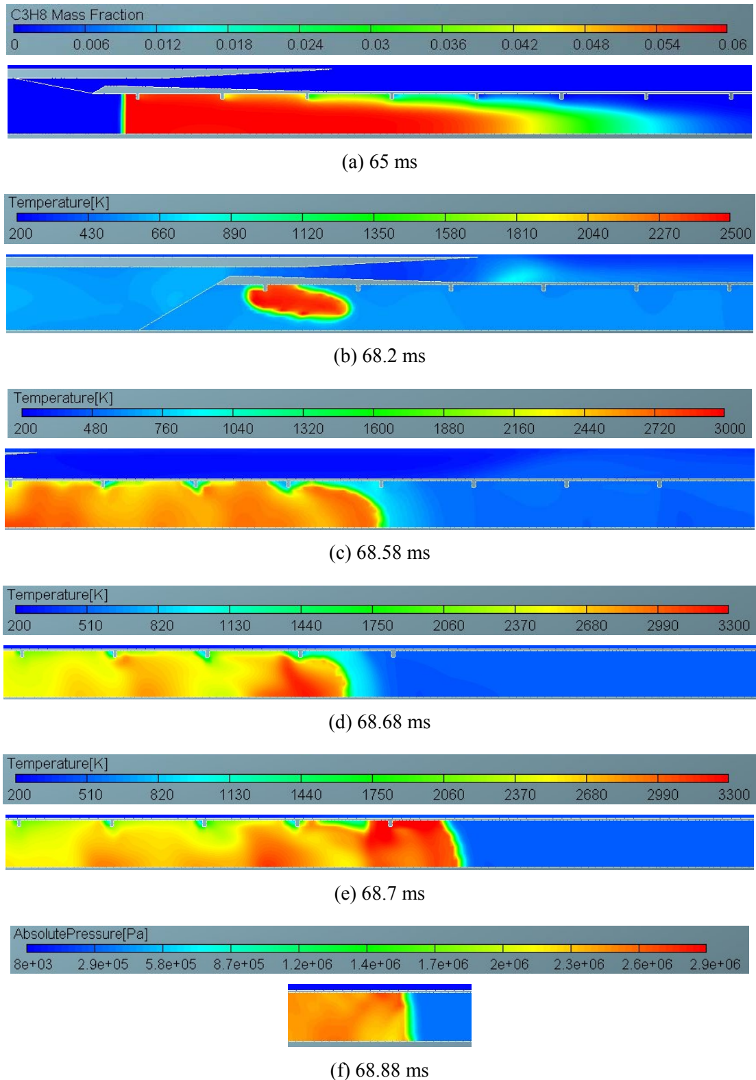
Figure 25: Flow patterns at detonation chamber filling with fuel (a), flame propagation shortly after ignition (b) and at a later stage, when flame accelerates considerably (c), as well as shortly prior to DDT (d) and shortly after DDT (e), and at detonation propagation in the detonation chamber (f).
