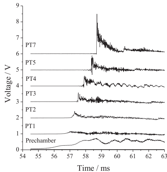
Figure 31: Example of pressure records by transducers PT1 to PT7 at ignition energy 0.1 J indicating the onset of detonation.
