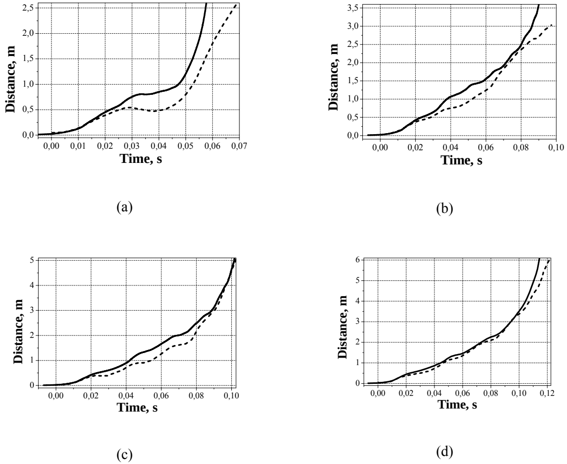
Figure 7: Comparison between predicted (solid curves) and measured [19] (dashed curves) distances traveled by the flame vs. time in 40 x 40 mm straight channels of different lengths filled with the stoichiometric propane-air mixture: (a) channel length 2.6 m, (b) 3.6 m, (c) 5.1 m, and (d) 6.1 m.
