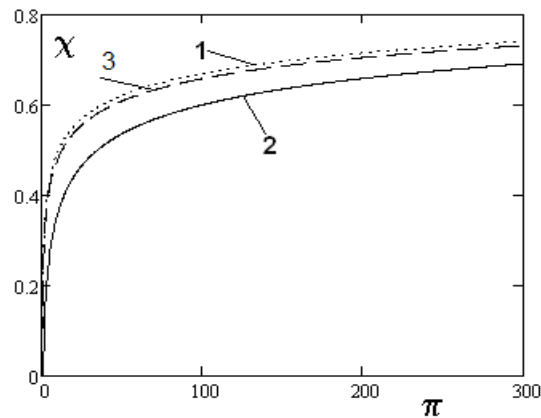
Figure 3: Predicted thermodynamic efficiency of PDE (1), Brayton (2), and Humphry (3) cycles depending on the precompression ratio \pi .
