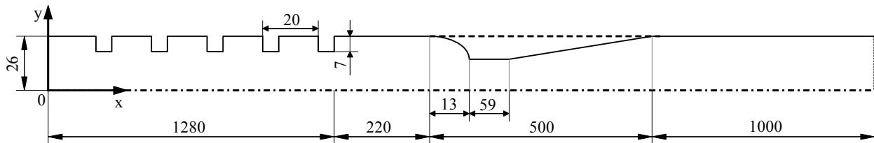
Figure 14: Schematic of a PDE tube with flame accelerator and shock focusing nozzle. Dimensions are in millimetres.
