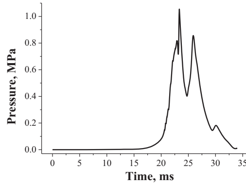
Figure 21: Predicted absolute pressure history at the head end of the PDE tube (PDE thrust wall).
