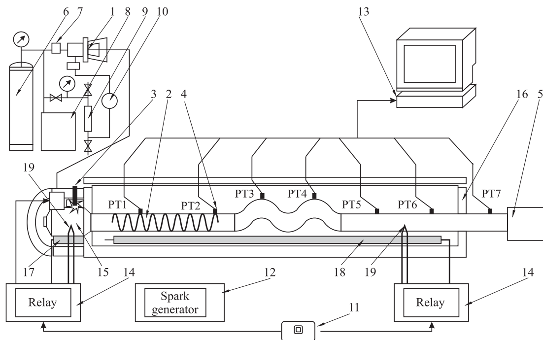
Figure 29: Kerosene-fueled predetonator with curved tube segment.
