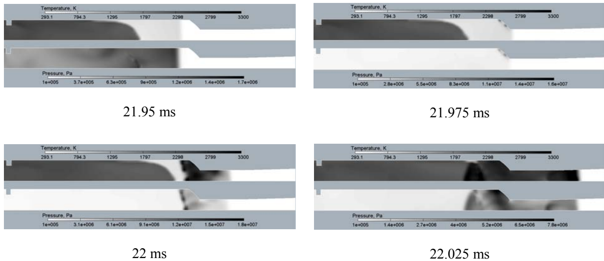
Figure 17: Snapshots of temperature and pressure fields prior, at and after shock-to-detonation transition (the transverse size of the tube is purposely increased to clarify the details).
