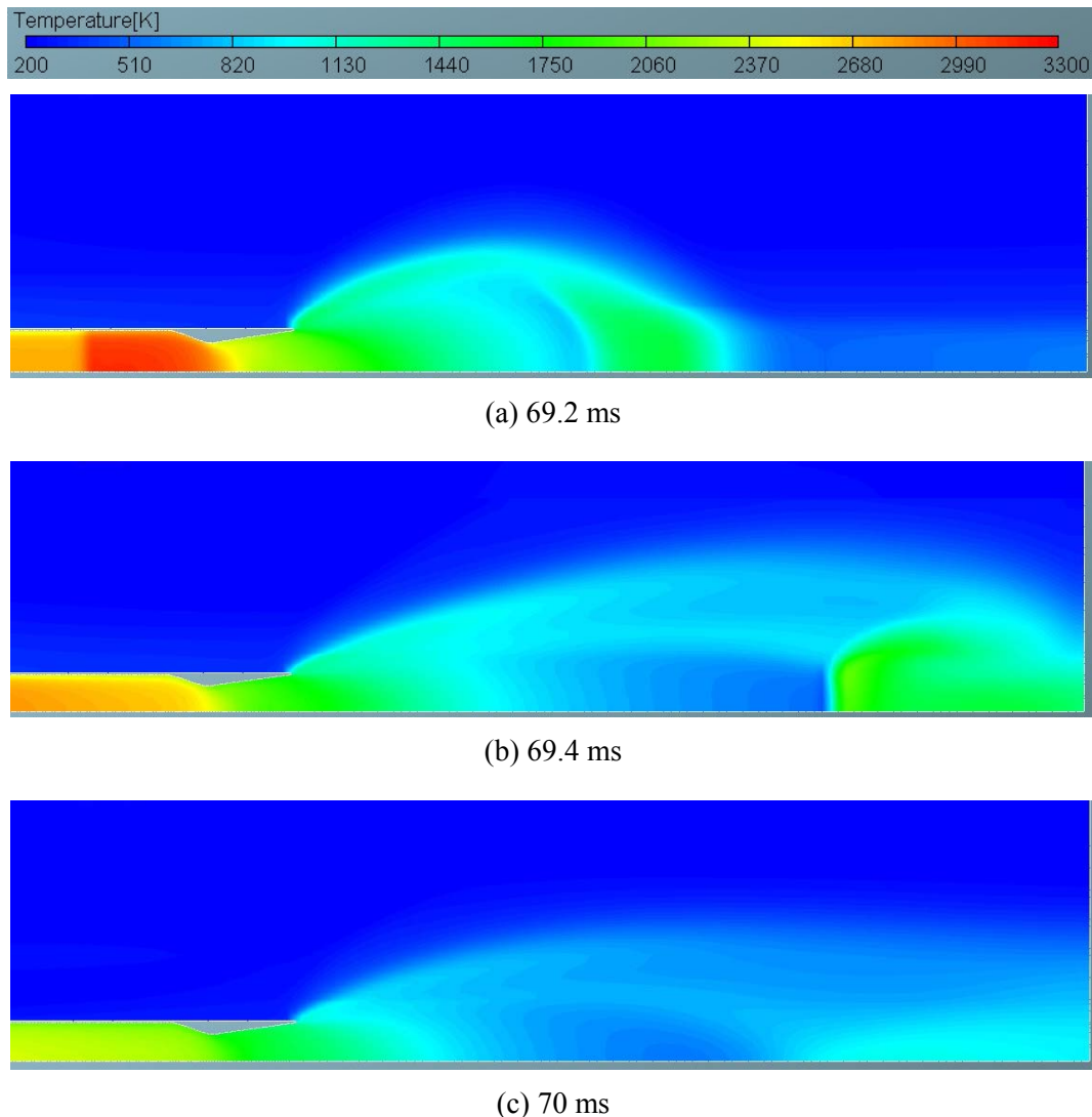
Figure 26: Flow patterns in the nozzle of the PDE-based vehicle and in the exhaust plume.
