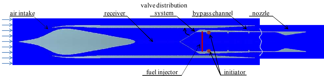
Figure 4: Pulsed detonation engine with supersonic air intake, bypass channel, mechanical valve, and nozzle.
