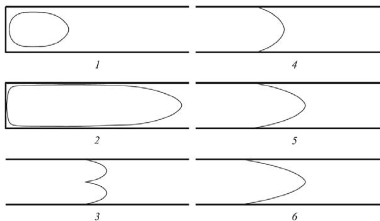
Figure 9: Snapshots of mean flame shapes at different locations in the 6.1-meter tube, shown by black dots in Fig. 8.
