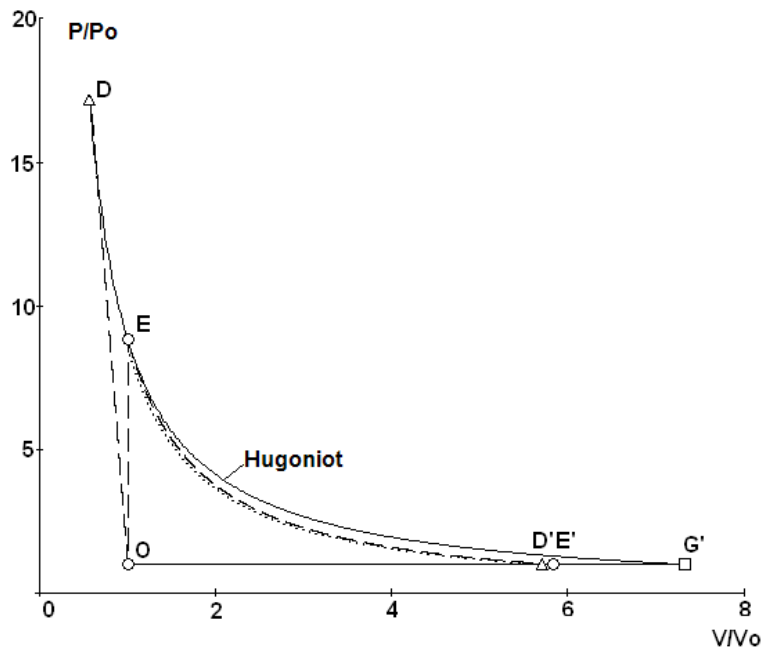
Figure 1: Thermodynamic cycles with constant-pressure, constant-volume, and detonative combustion (no precompression).
