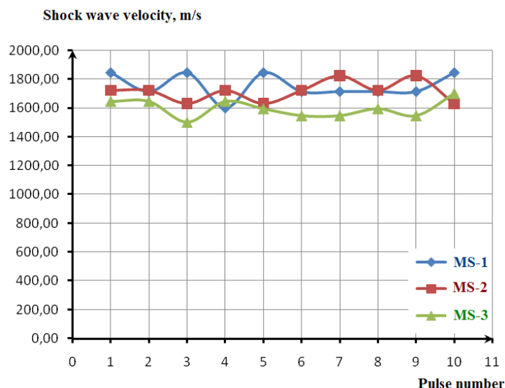
Figure 33: Measured shock wave velocities at three measuring segments MS-1, MS-2, and MS-3 (see Fig. 32) in 10 successive pulses.
