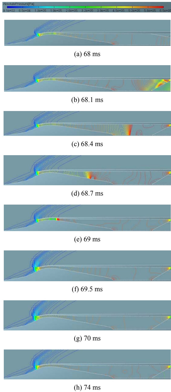
Figure 24: Predicted response of the flow in the engine receiver to a change in the valve position in terms of static pressure isolines.
