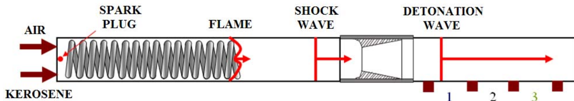
Figure 32: Kerosene-fueled predetonator with a CD nozzle as a shock-focusing element.
