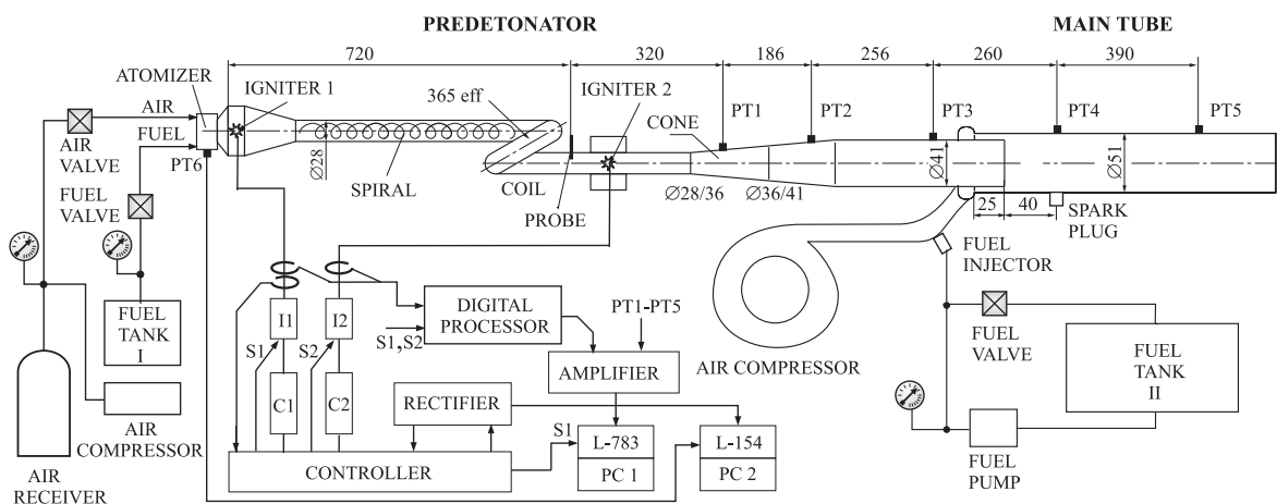
Figure 27: The Semenov Institute RPDE demonstrator.
