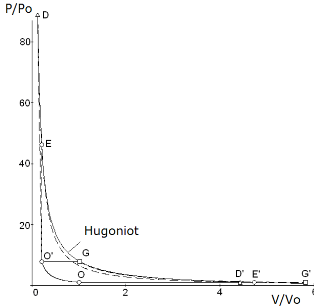
Figure 2: Thermodynamic cycles with constant-pressure, constant-volume, and detonative combustion (with precompression).
