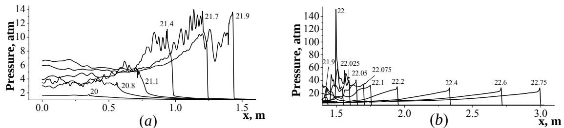
Figure 18: Predicted spatial pressure distributions in the PDE channel at different time (in ms) after ignition. Different pressure scales are used for t < 21.9 (a) and t > 21.9 ms (b).
