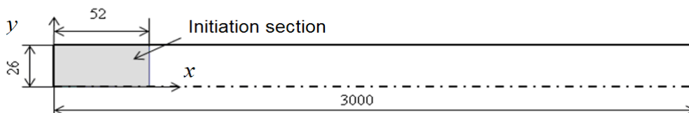
Figure 5: Schematic of an idealized PDE with a section for direct detonation initiation.
