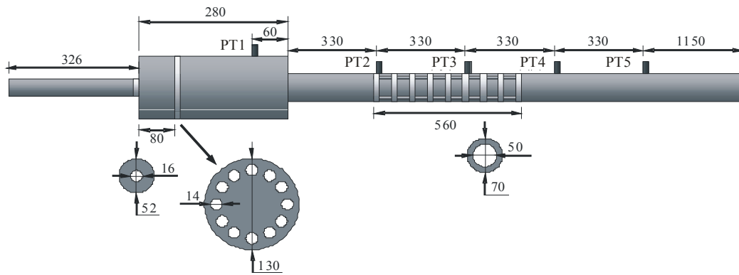
Figure 11: Schematic of experimental setup (PT stands for pressure transducer). Dimensions are in millimeters.
