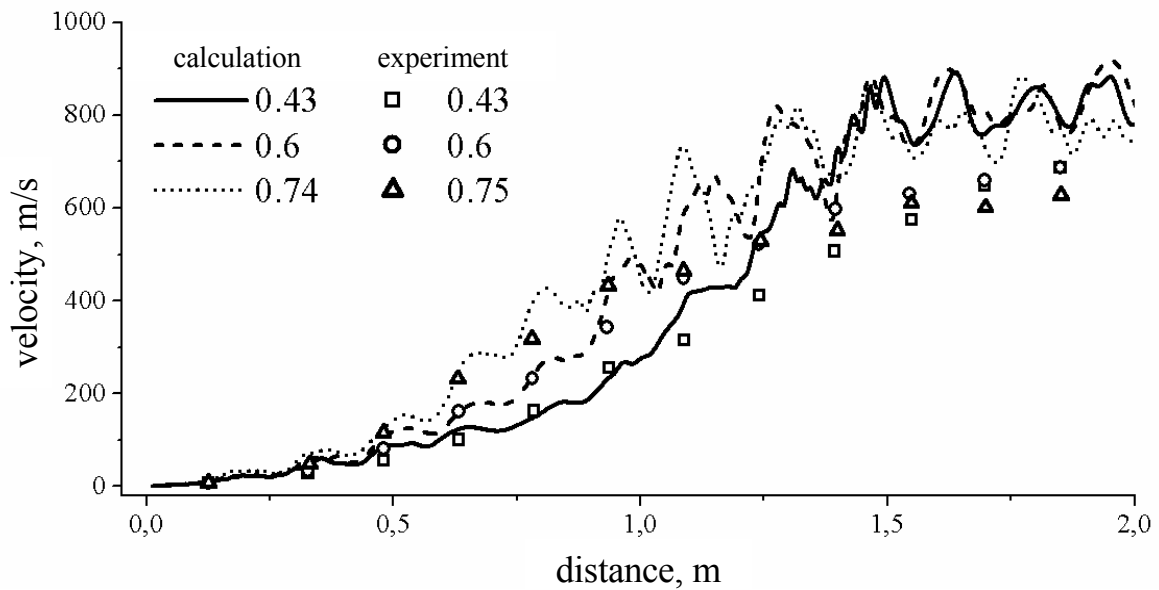
Figure 10: Predicted (curves) and measured (symbols [20]) visible flame velocities vs. distance in tubes of D = 152 mm with regular orifice plates (BR = 0.43, 0.6, and 0.75, pitch S = D ). Stoichiometric propane – air mixture at T_0 = 293 K and p_0 = 1 atm.
