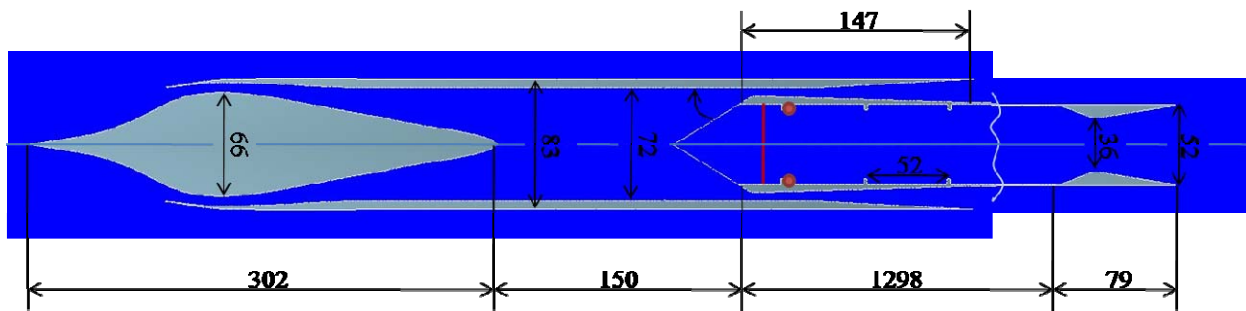
Figure 22: Flying PDE-based vehicle. Dimensions are in millimeters.
