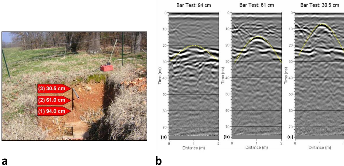
Figure 14. Ground-Penetrating Radar Velocity Bar Test: (a) a metal bar was inserted into a trench wall at three different depths; (b) reflection hyperbolas from each depth. In this case the test was done at 94, 61, and .305 m. (The reflection from the deepest bar persist in each test because we were unable to retrieve the bar after the initial test.)
