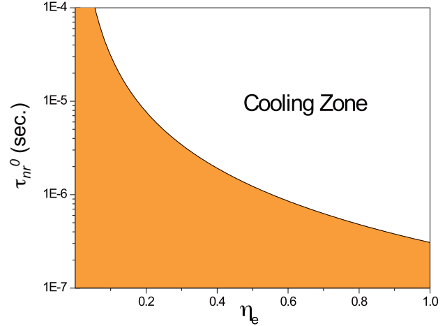
Figure 8 (online color at: www.lpr-journal.org) The break-even nonradiative lifetime as a function of the luminescence extraction efficiency in bulk GaAs calculated using typical values of radiative and Auger recombination at room temperature.
