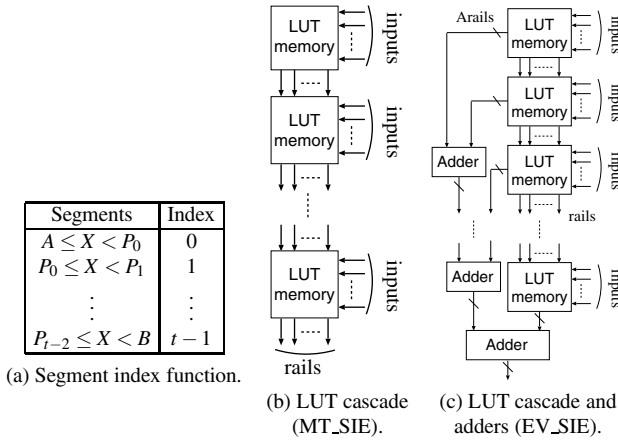
Fig. 5 Segment index encoders.
