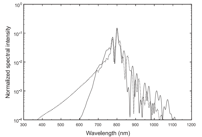
FIGURE 5 Frequency spectrum calculated on the beam axis without consideration of the self-steepening term \pm(i/\omega_0)(\partial/\partial\tau) in (6) ( solid line ) and with the inclusion of this term so that (\omega_0\tau_0)^{-1} = 0.007 ( dotted line ). In the simulations the pulse duration was \tau_0 = 90 \text{ fs} (150 fs FWHM), the ratio of the peak power to the critical power for self-focusing P_{\text{peak}}/P_{\text{cr}} = 6 , the input beam radius a_0 = 0.18 \text{ mm} , and z = z_d . The intensity is normalized to the peak input spectral intensity
