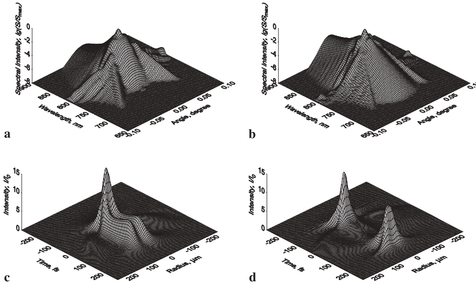
FIGURE 6 Frequency angular spectrum (a, b) and spatio-temporal distribution (c, d) of the pulse at two propagation distances: a, c z = 0.43z_d ; b, d z = 0.6z_d . In the simulations the pulse duration was \tau_0 = 150 fs (250 fs FWHM), the ratio of the peak power to the critical power for self-focusing P_{\text{peak}}/P_{\text{cr}} = 6.3 , and the input beam radius a_0 = 0.18 mm
