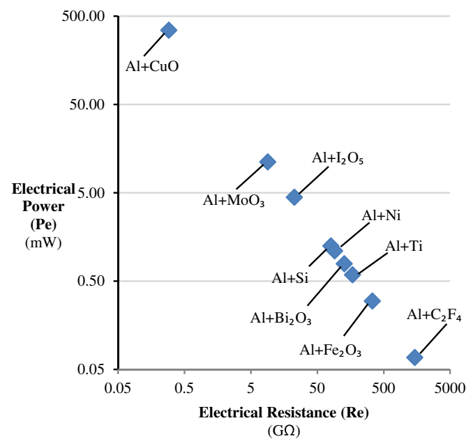
Fig. 5. Variation of electrical power with electrical resistance.
