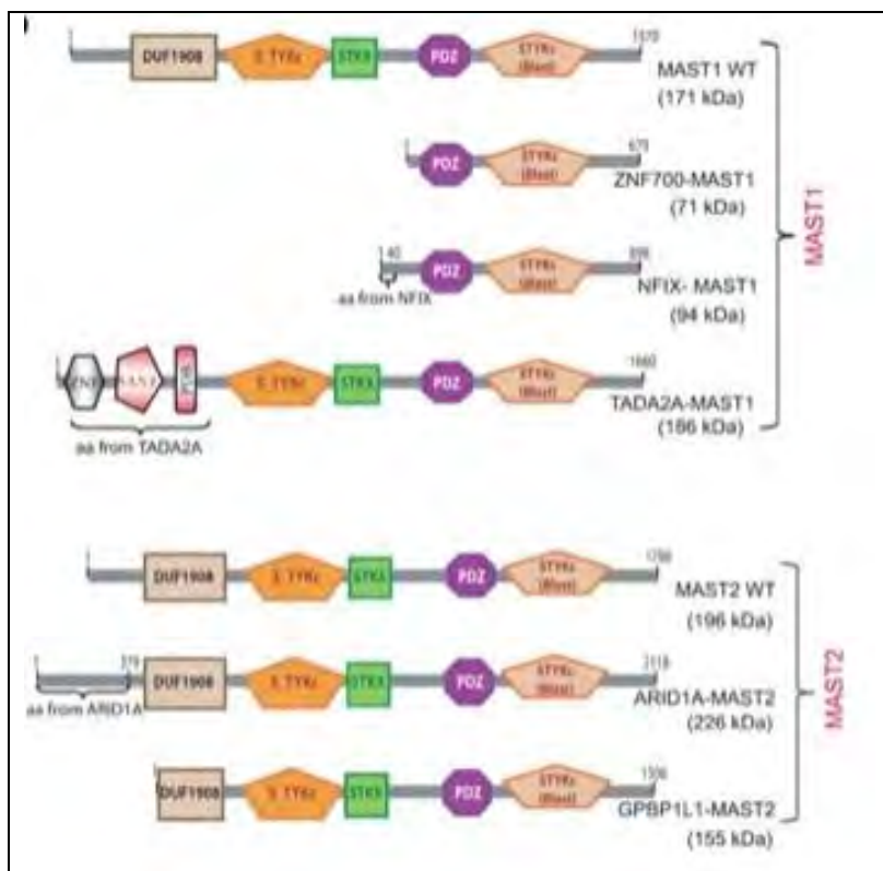
Figure 8. Schematic representation of functional domains retained in the putative chimeric proteins involving MAST1 and MAST2. Nat Med. 2011 Nov 20;17(12):1646-51.
