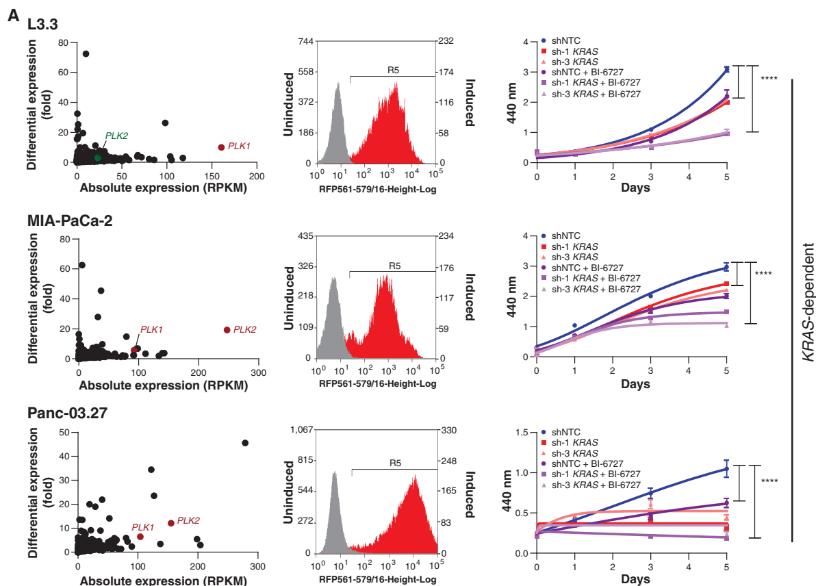
Figure 6. Knockdown of KRAS combined with PLK inhibition reduces cell proliferation in indicated KRAS -dependent cell lines (A) but not in KRAS -independent cell lines (B). (continued on following page)
