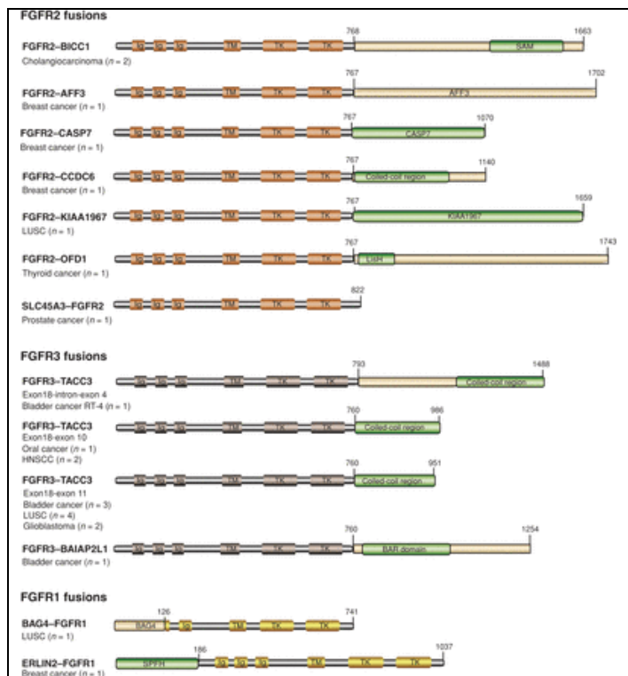
Figure 22. Schematic representations of the predicted FGFR fusions identified by transcriptome sequencing of human cancers. Data used include RNA sequencing results from the 4 index patients, our internal tumor cohort, and the TCGA compendium. Out of 4 FGFR receptor family members, FGFR1, FGFR2, and FGFR3 are involved in gene fusions with various partners located on several chromosomes. Eleven distinct fusion partners of FGFRs were identified. Cancer Discov. 2013 Jun;3(6):636-47
