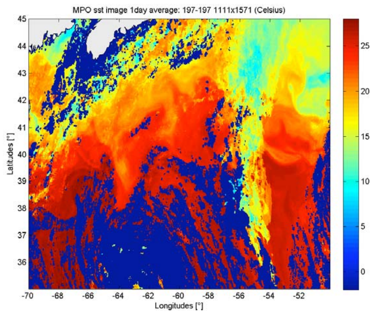
Figure 3: 15 July 2008 DFO SST average pixel.
