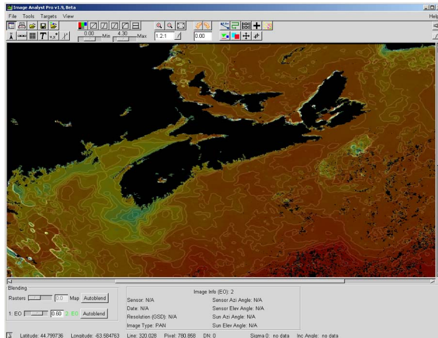
Figure 9: Colourized SST field and embedded SST gradient.
