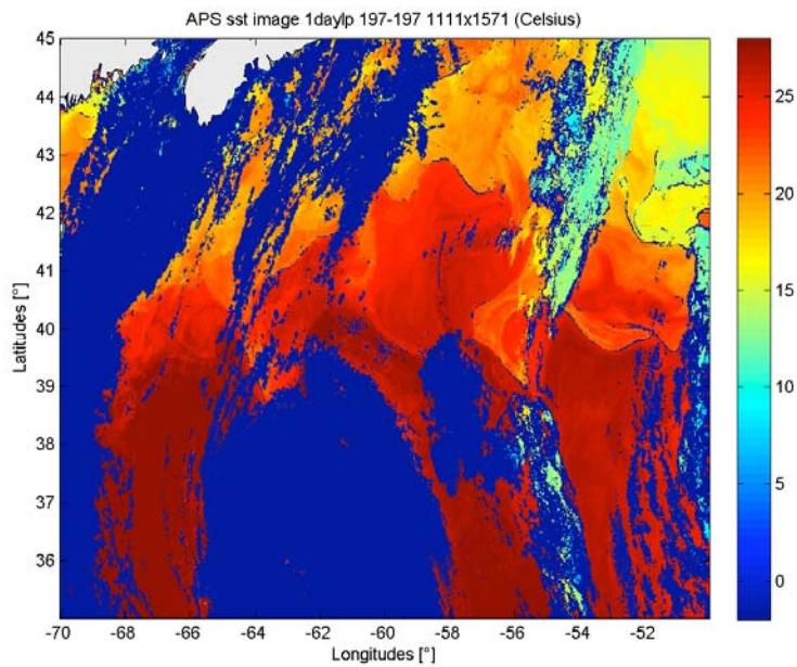
Figure 2: 15 July 2008 APS 1-day latest pixel.
